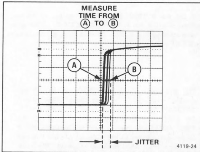
Figure 23. Pulse jitter.
