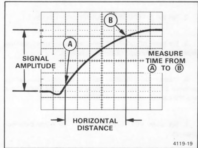
Figure 18. Rise time.
