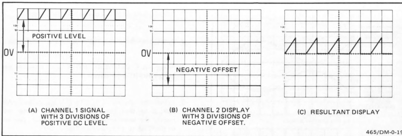
Figure 15. Algebraic addition.
