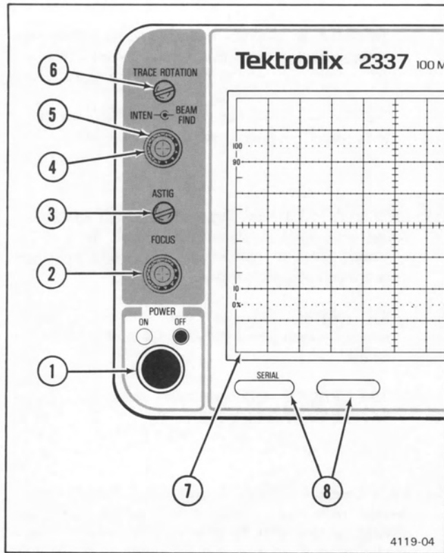
Figure 3. Power and display controls and indicators.
