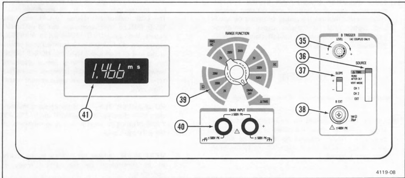
Figure 7. DMM and B TRIGGER controls, connectors, and LCD readout.
