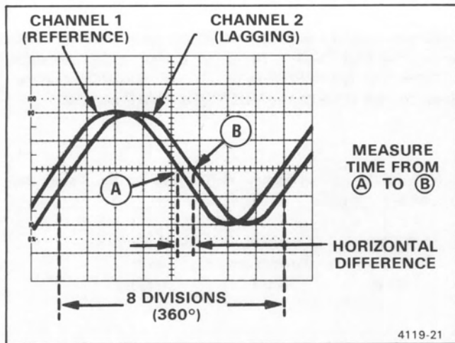
Figure 20. Phase difference.
