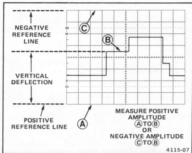
Figure 14. Instantaneous voltage measurement.
