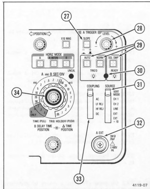
Figure 6. A TRIGGER controls, connector, and indicator.
