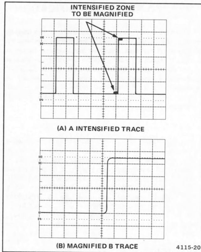
Figure 22. Delayed-sweep magnification.
