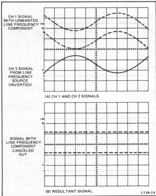
Figure 16. Common-mode rejection.
