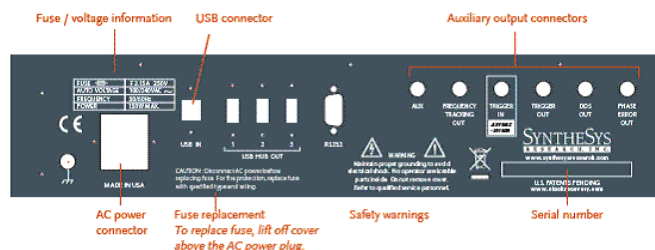
Rear Panels
