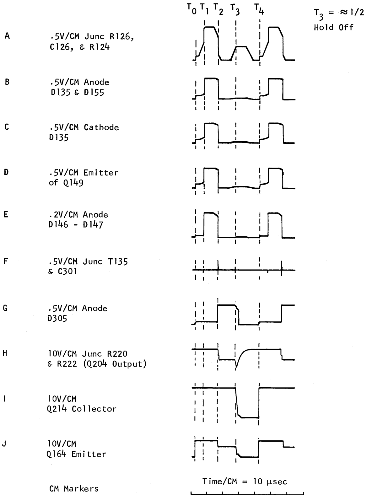
Pseudo Schmitt Waveforms fig 2-3
