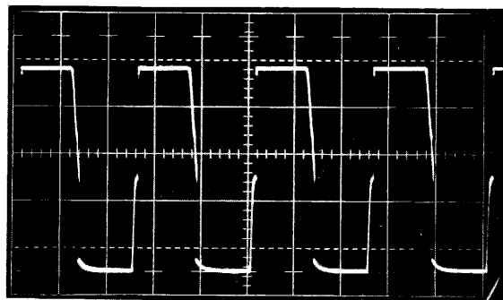
(Test scope display) When R172 is adjusted a slight rotation CW of the STABILITY control should free run the instrument.
