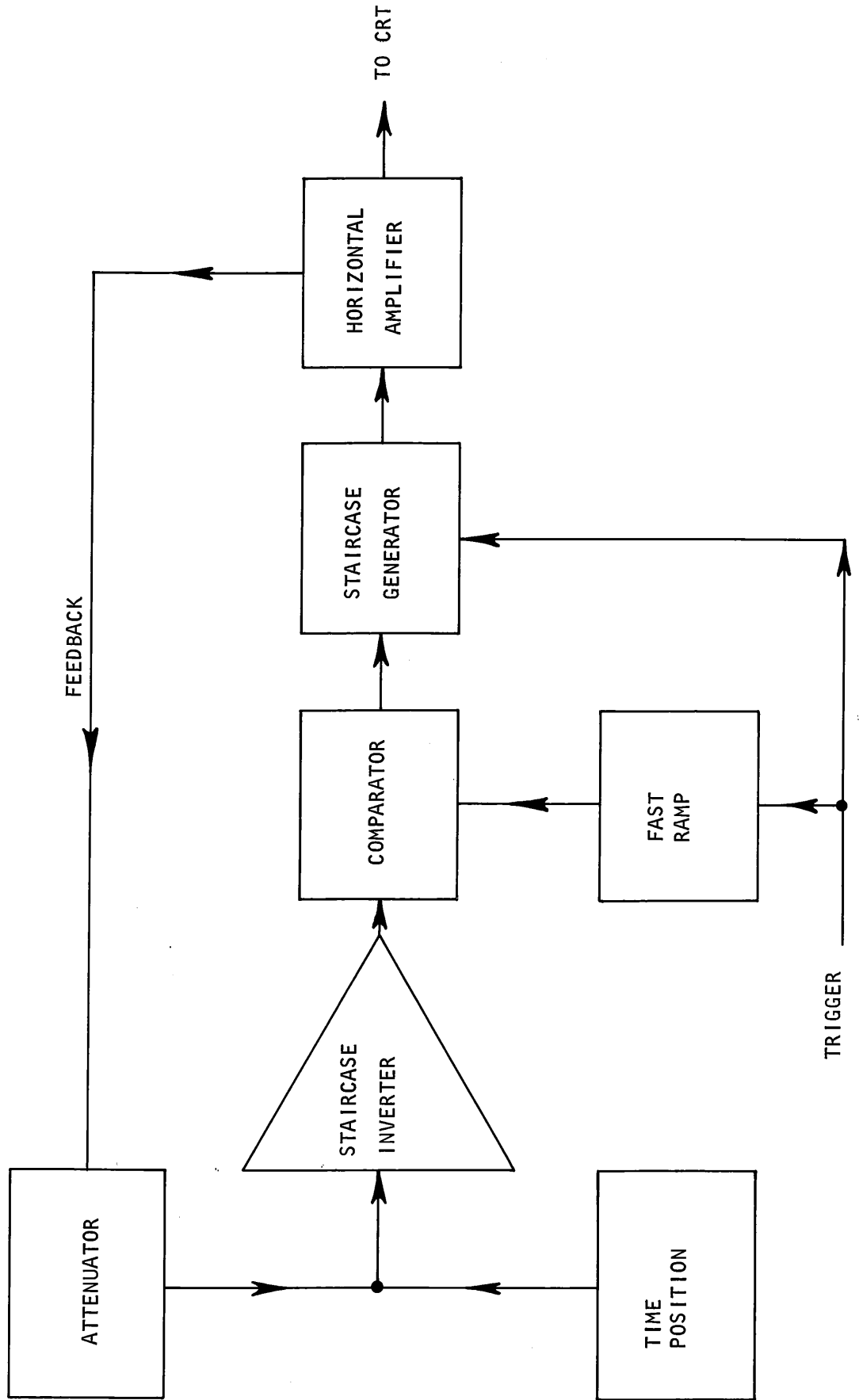
SAMPLING TIME BASE BASIC BLOCK DIAGRAM
