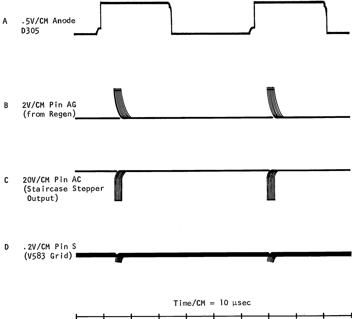
Staircase Stepper Circuit fig 3-18
