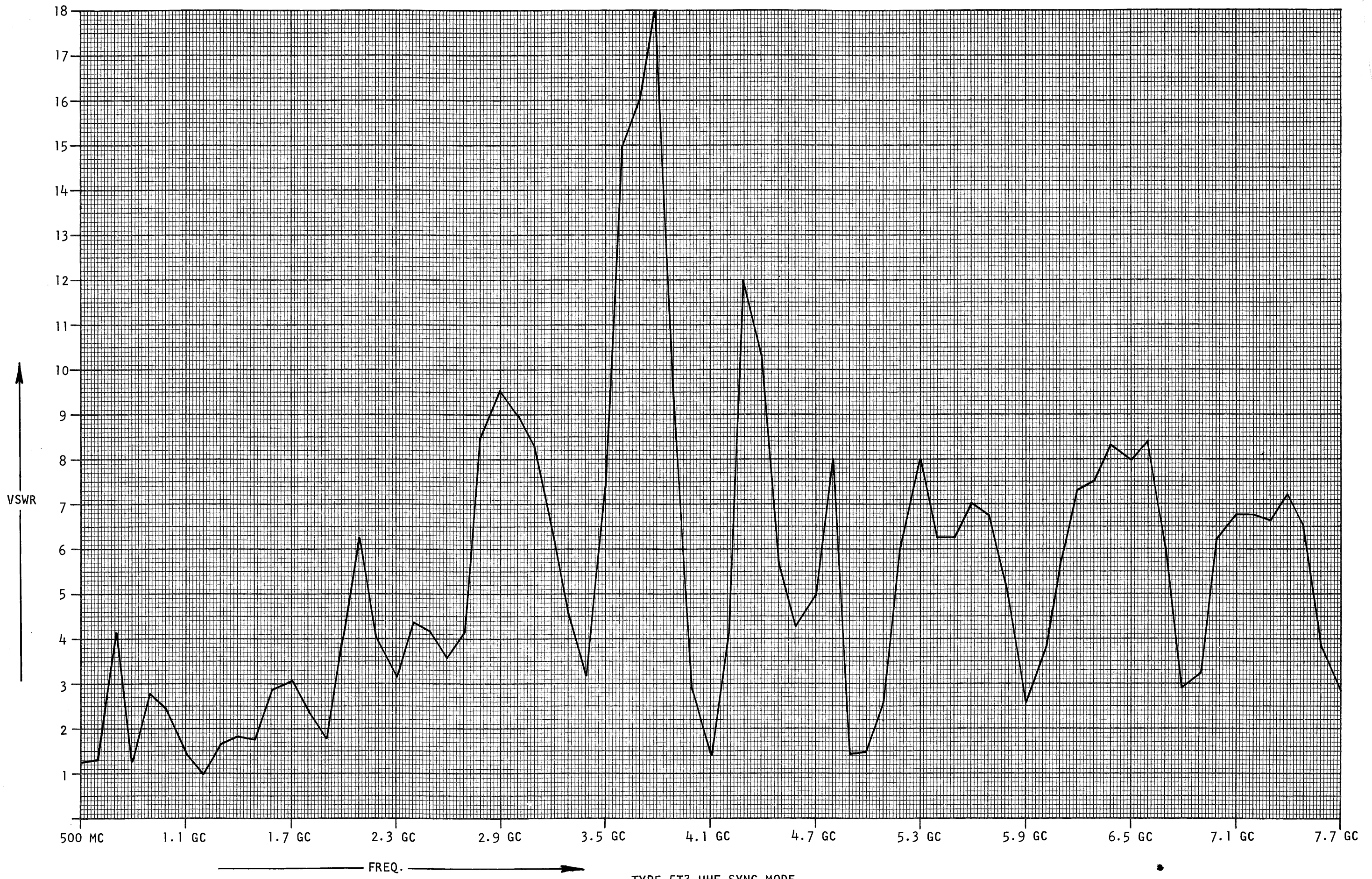
TYPE 5T3 UHF SYNC MODE
