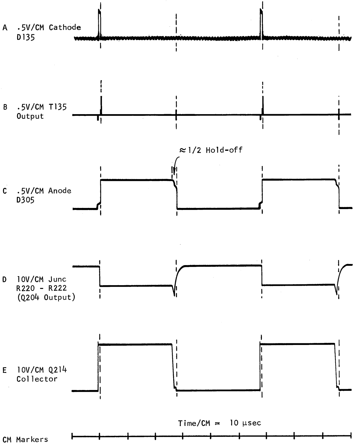
Pseudo Schmitt Loop fig 3-6
