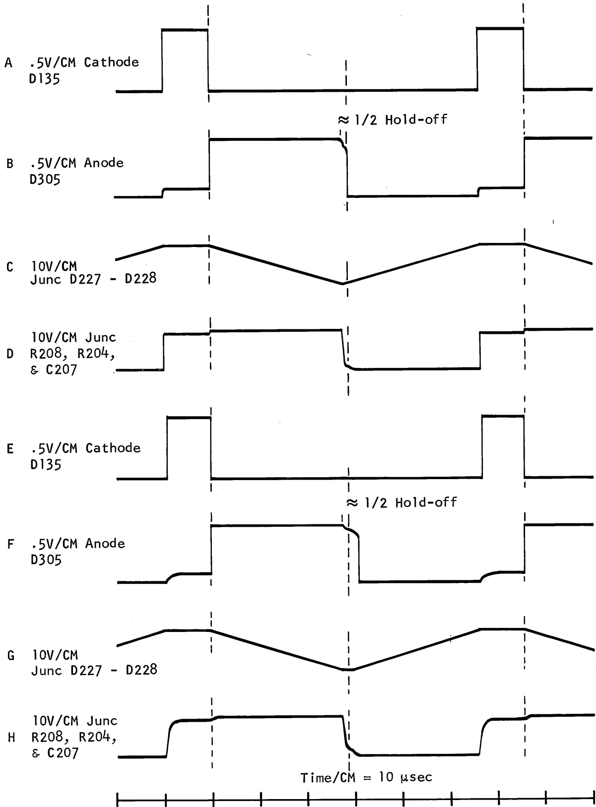
Pseudo Schmitt and Auto Recovery Comparison fig 3-7
