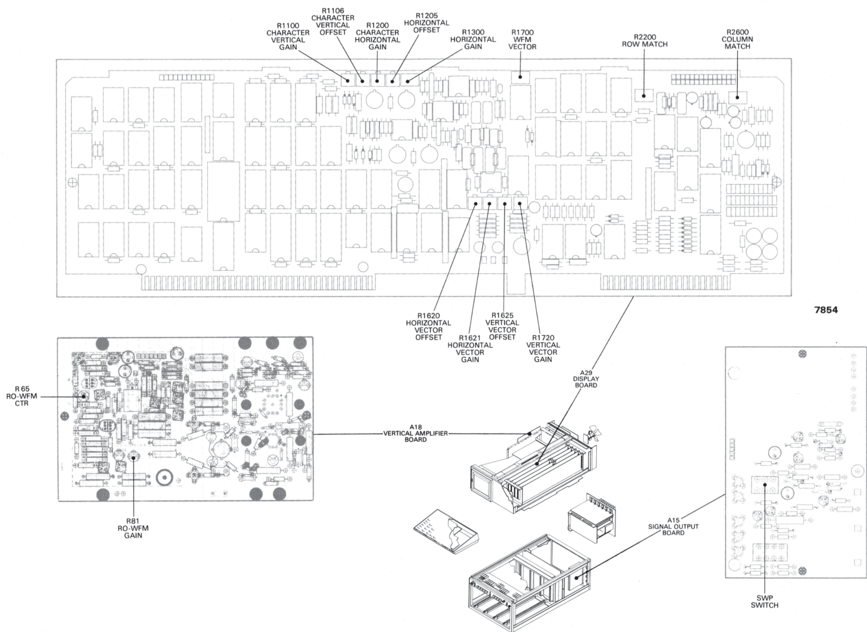
Figure 7-62. Test Point and Adjustment Locations G.
