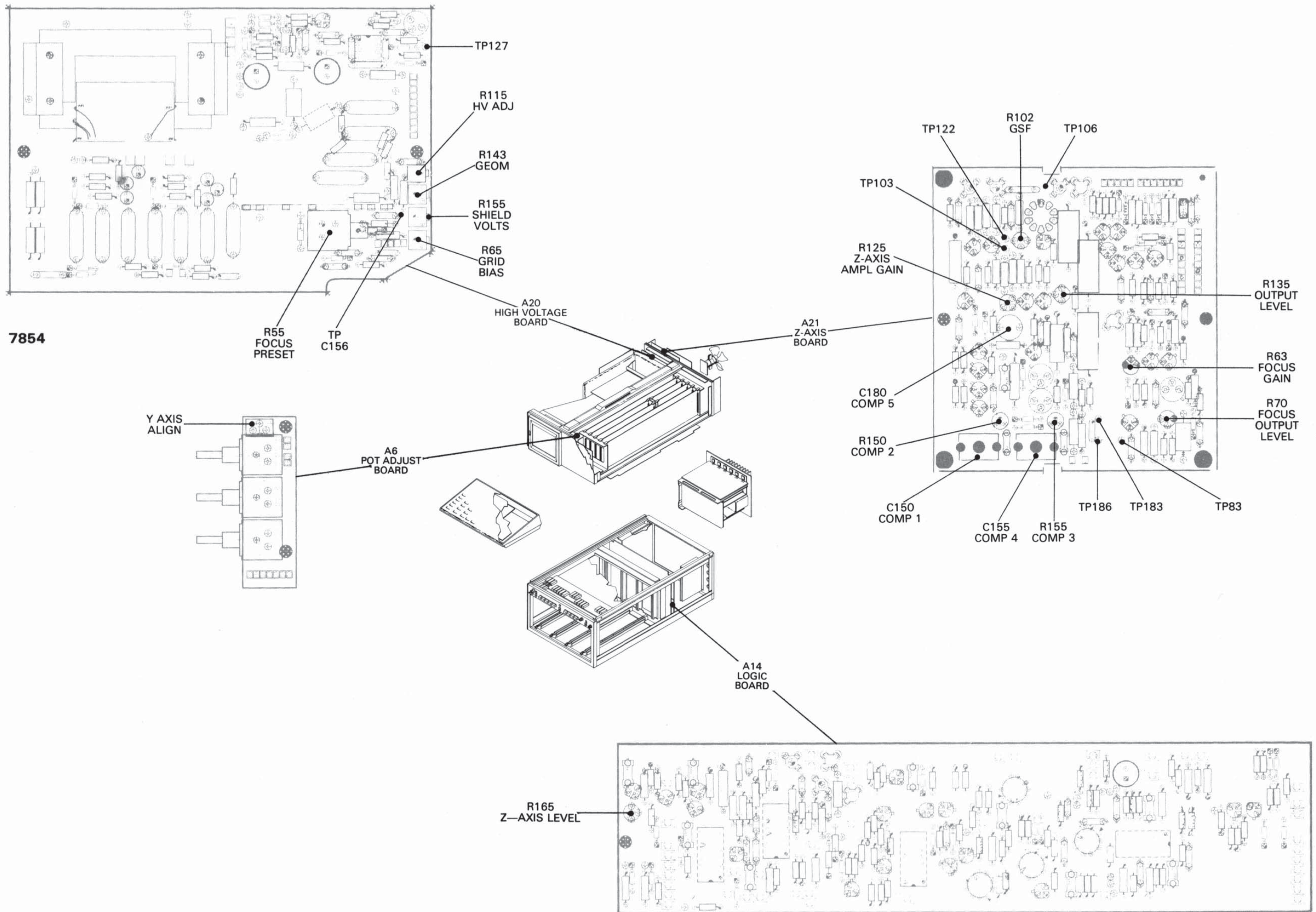
Figure 7-57. Test Point and Adjustment Locations B.
