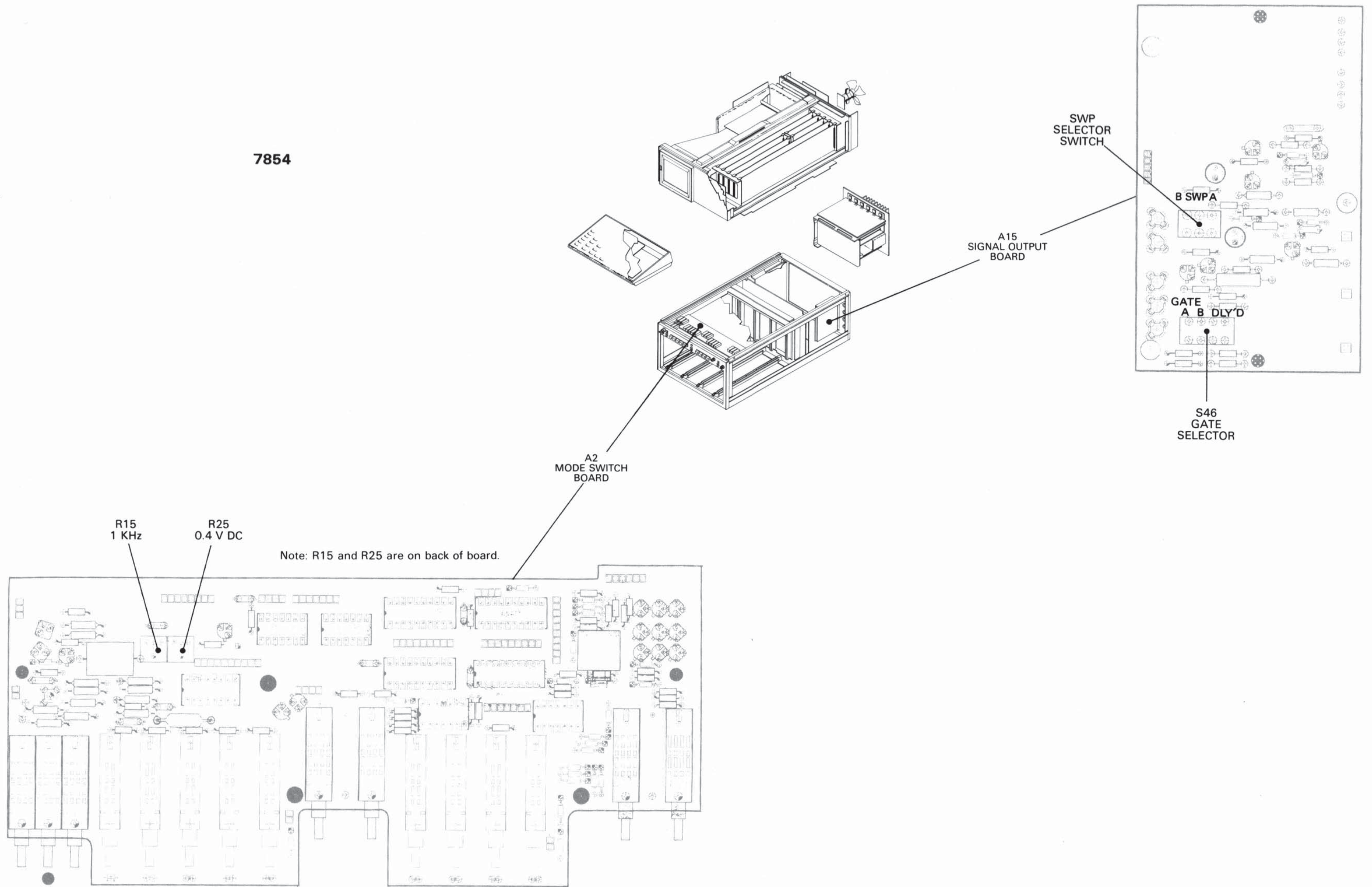
Figure 7-58. Test Point and Adjustment Locations C.
