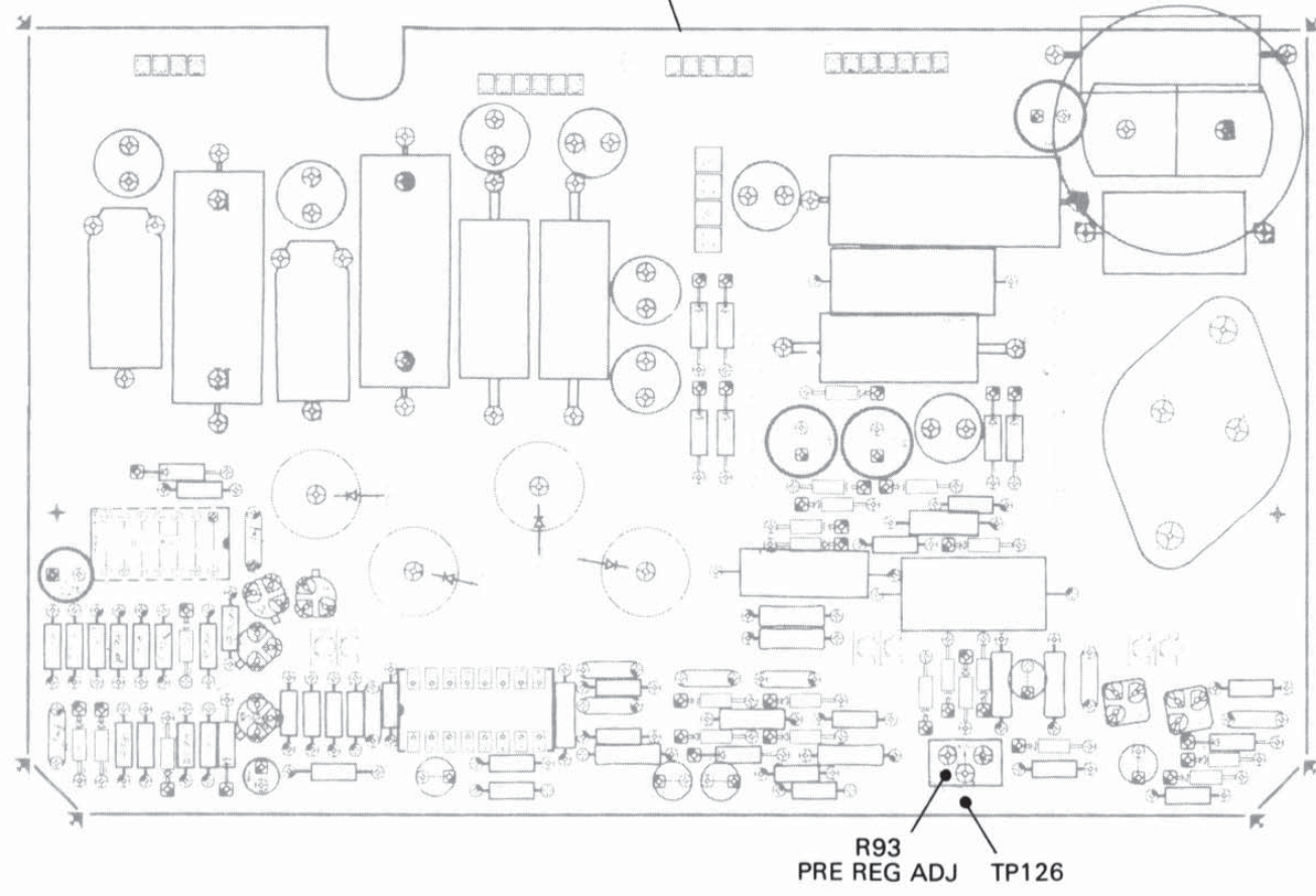
Figure 7-56. Test Point and Adjustment Locations A.
