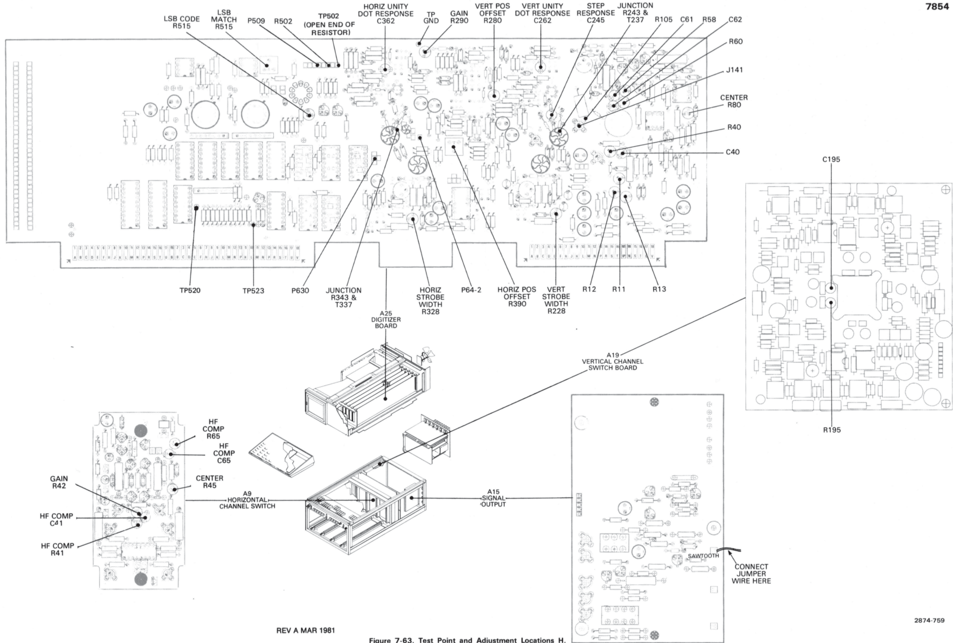
Figure 7-63. Test Point and Adjustment Locations H.
