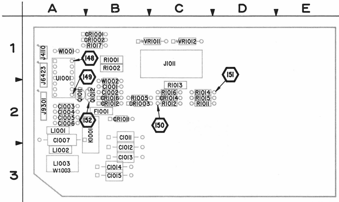
Figure 9-21. A20—X-Y Plotter board.
