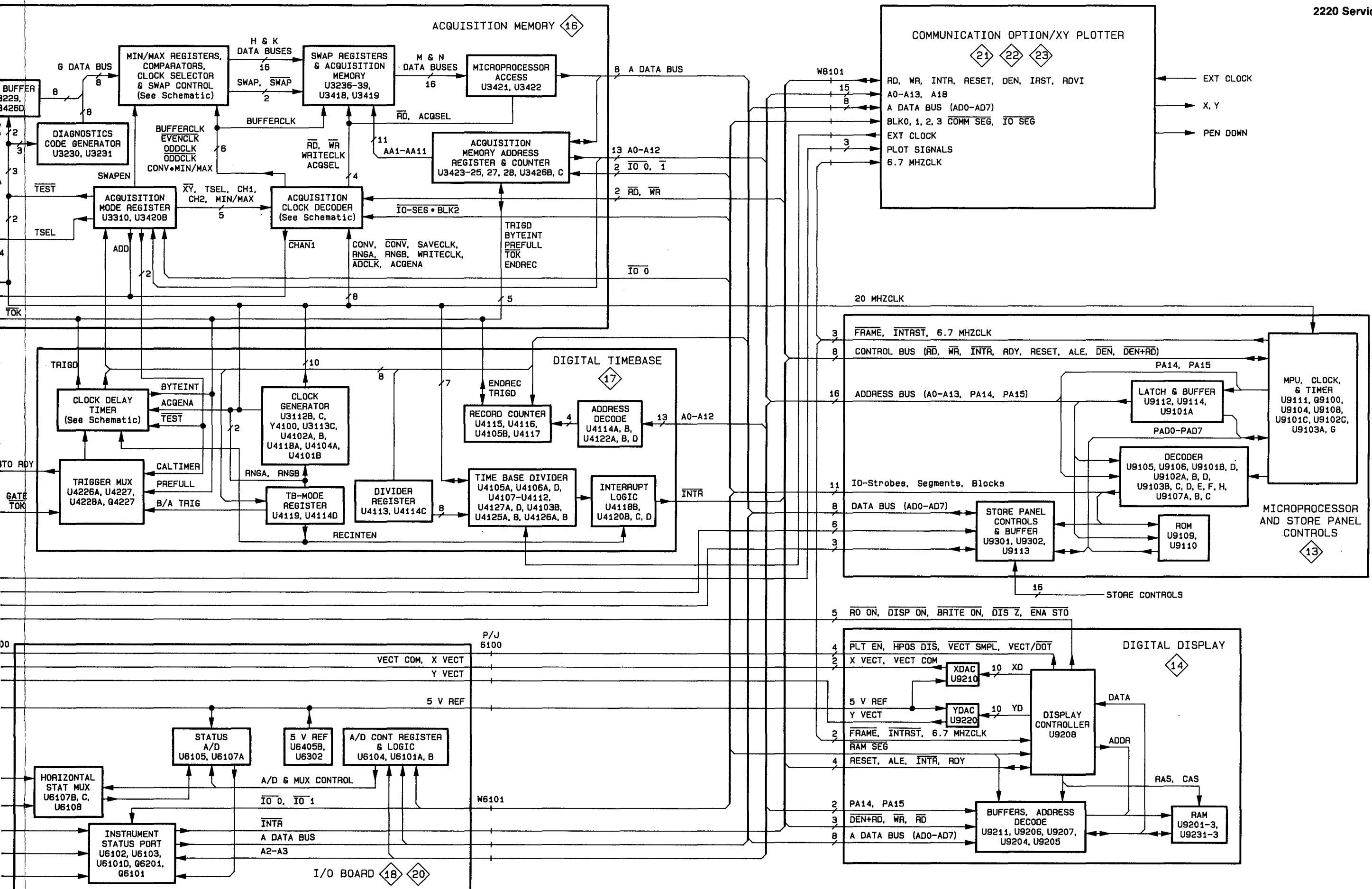
Figure 9-5. Detailed storage block diagram.
