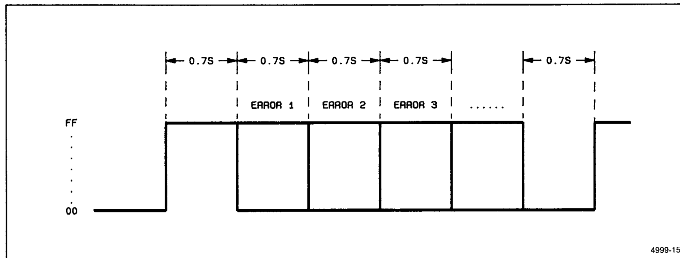
Figure 6-4. Error code timing (U4119).
