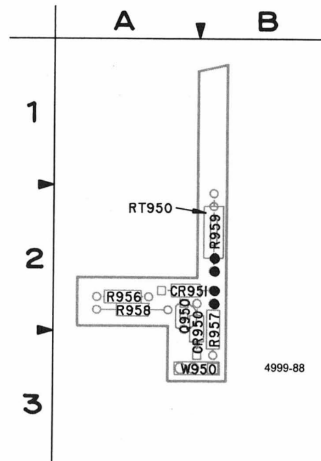
Figure 9-16. A18—Thermal Shutdown board.
