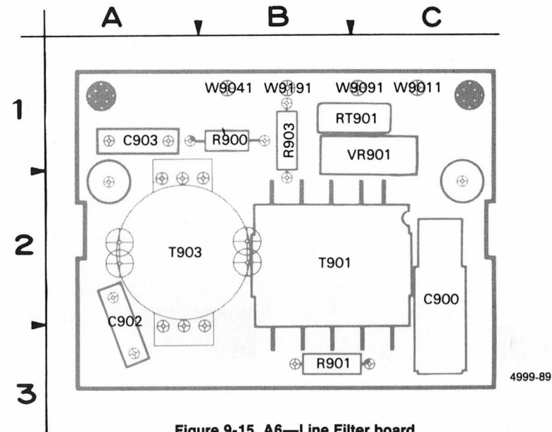
Figure 9-15. A6—Line Filter board.
