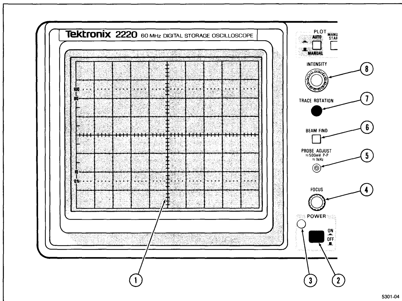
Figure 2-4. Power and display controls and power-on indicator.
