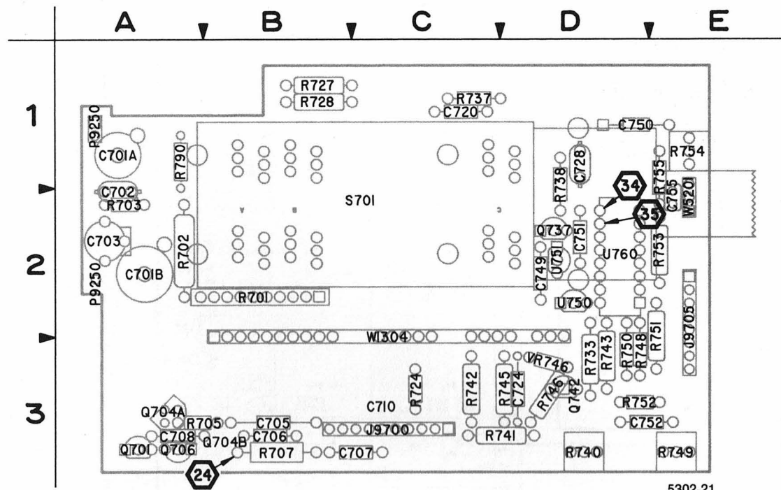
Figure 9-12. A4—Timing board.
