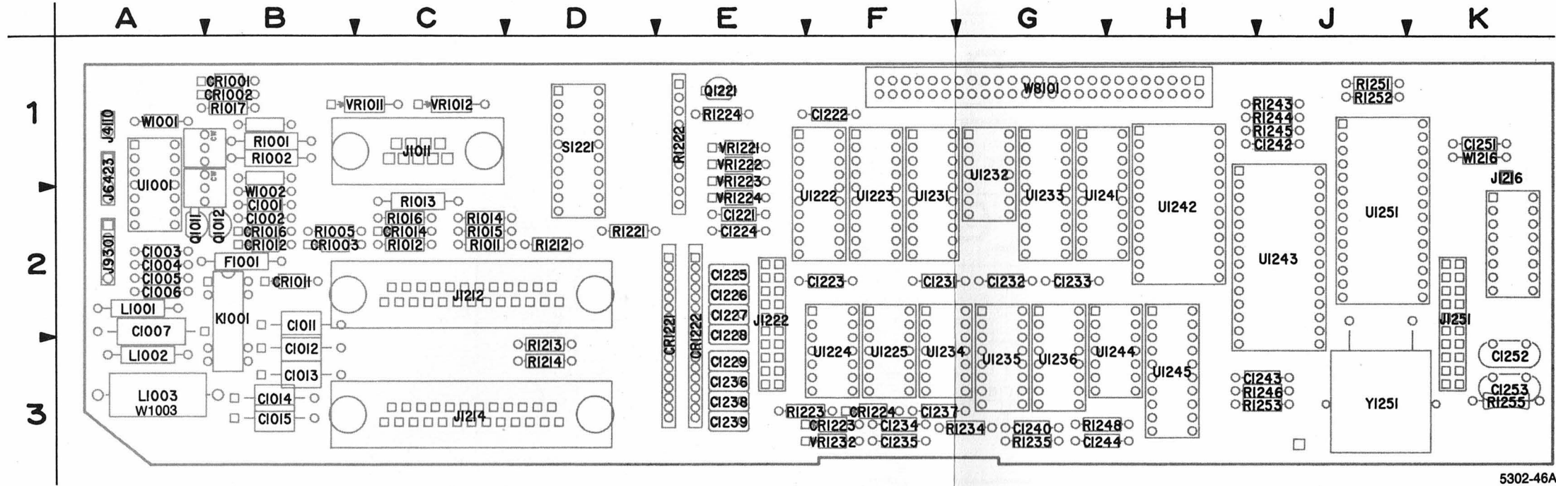
Figure 9-22. A21—RS-232 Option board.
