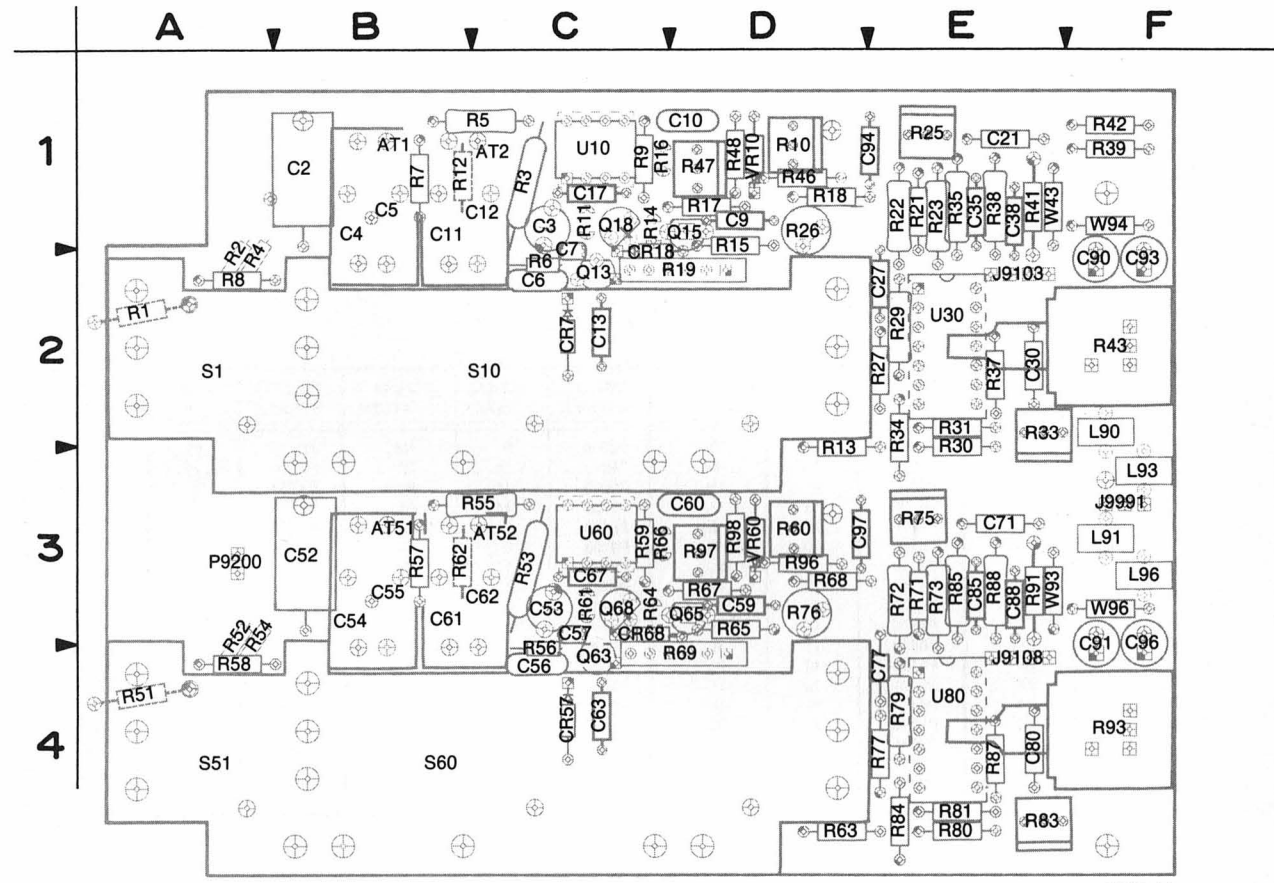
Figure 9-6. A2—Attenuator board.
