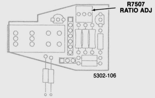
A16—SWEEP REFERENCE ADJUSTMENT LOCATIONS
