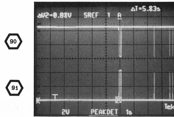
TEST SCOPE TRIGGERED ON U4118 PIN 6 FOR WAVEFORMS 90 THROUGH 93.
