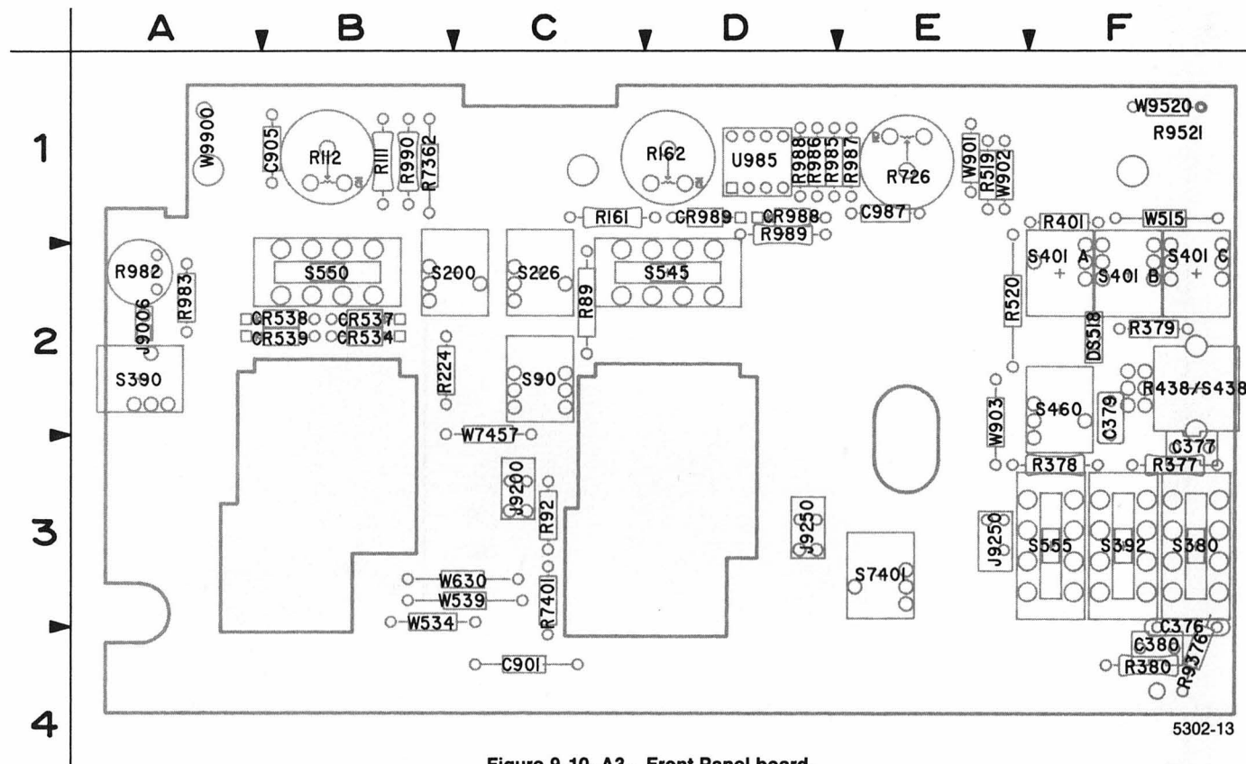
Figure 9-10. A3—Front Panel board.
