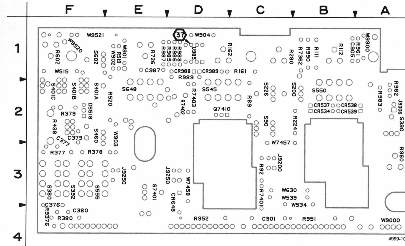
Figure 9-11. Circuit view of A3—Front Panel board.
