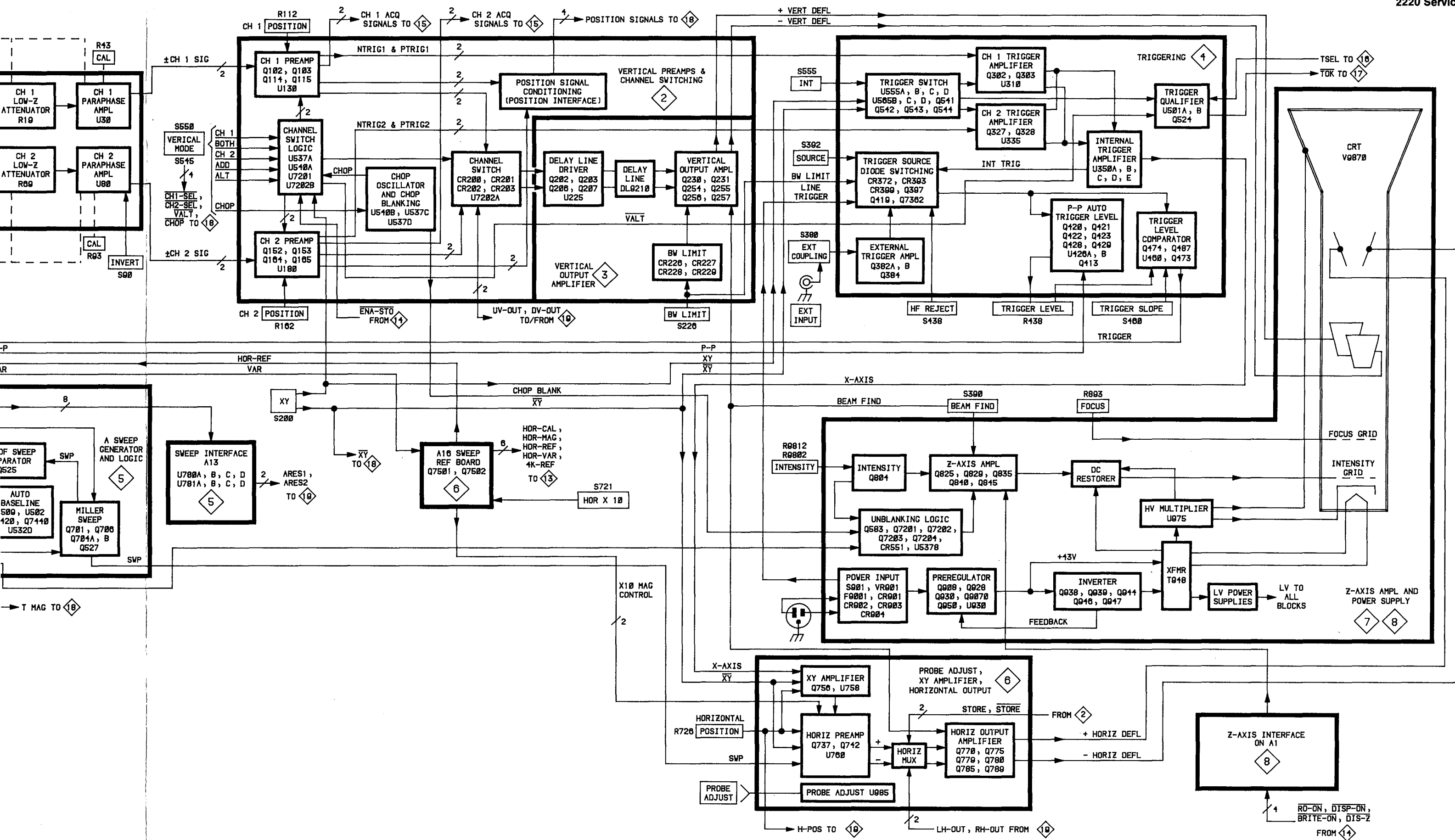
Figure 9-4. Detailed analog block diagram.
