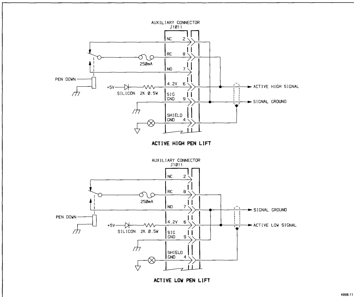
Figure 2-11. X-Y Plotter interfacing.
