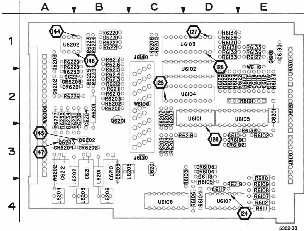
Figure 9-19. A11A1—Input/output board.
