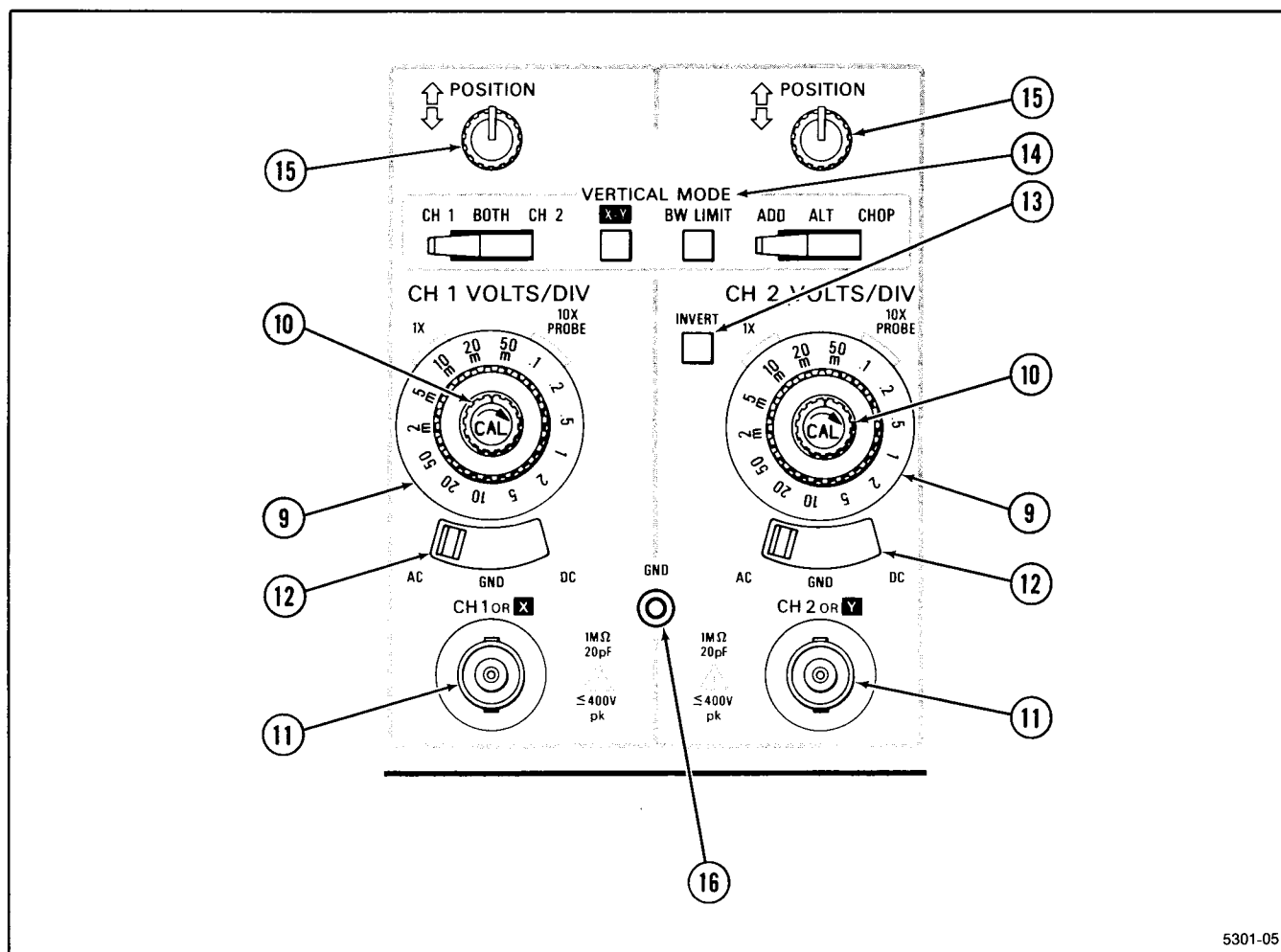
Figure 2-5. Vertical controls and connectors.
