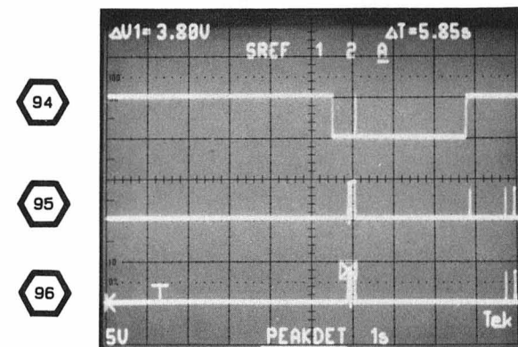
TEST SCOPE TRIGGERED ON U9111 PIN 21 FOR WAVEFORMS 94 THROUGH 99.
