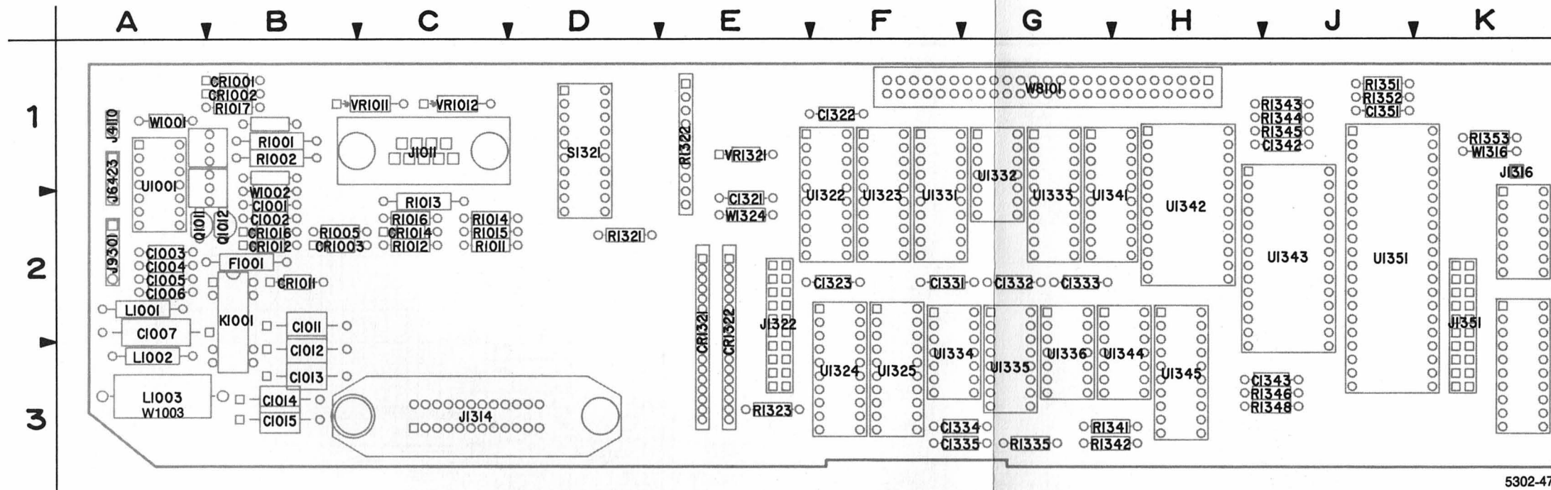
Figure 9-23. A22—GPIB Option board.
