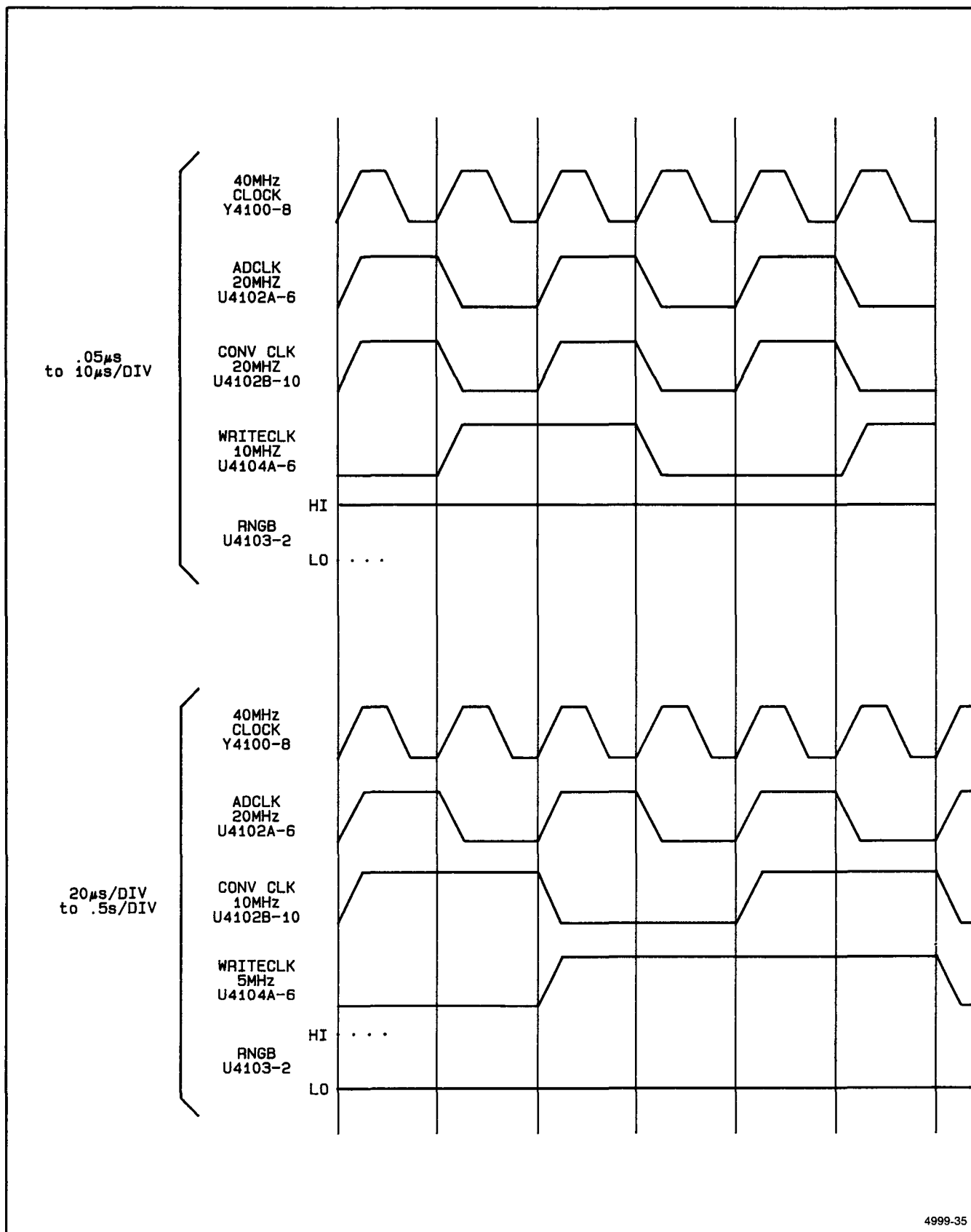
Figure 3-10. Clock timing.
