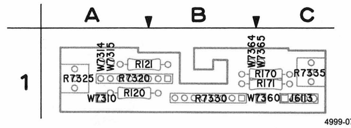
Figure 9-9. A17—Position Interface board.
