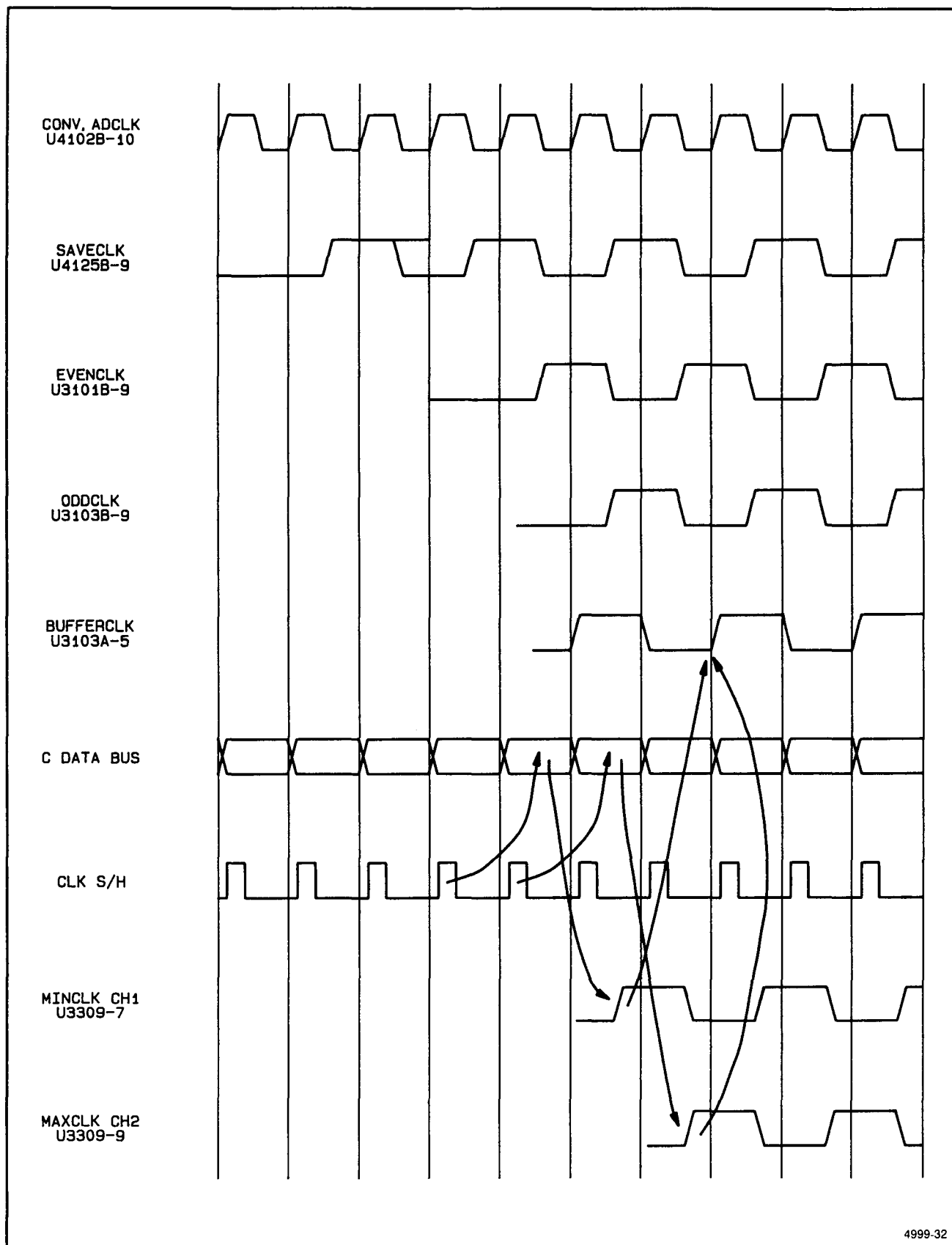
Figure 3-7. Sampling mode acquisition timing at 0.05 μs per division (ADCLK=CONV=20 MHz).
