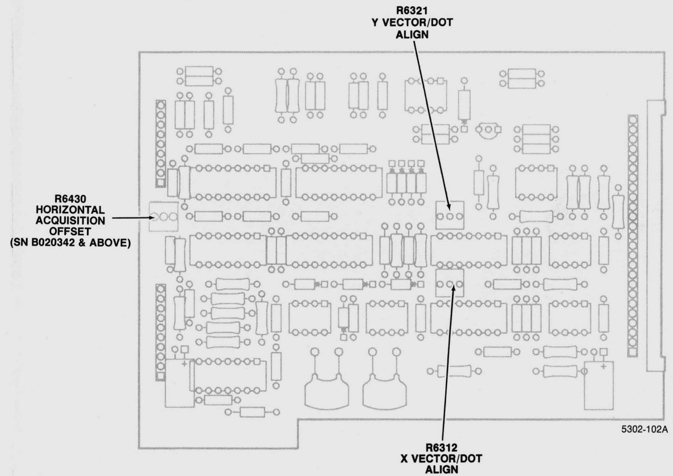
A11A2—VECTOR GENERATOR ADJUSTMENT LOCATIONS
