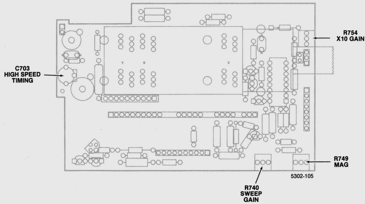
A4—TIMING BOARD ADJUSTMENT LOCATIONS
