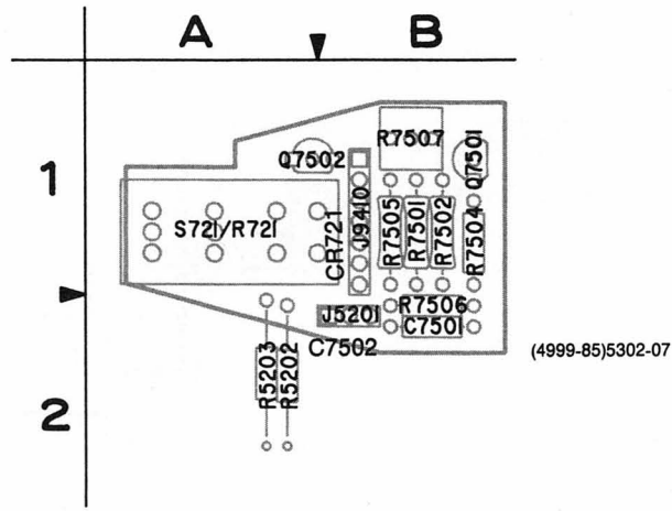
Figure 9-14. A16—Sweep Reference board.
