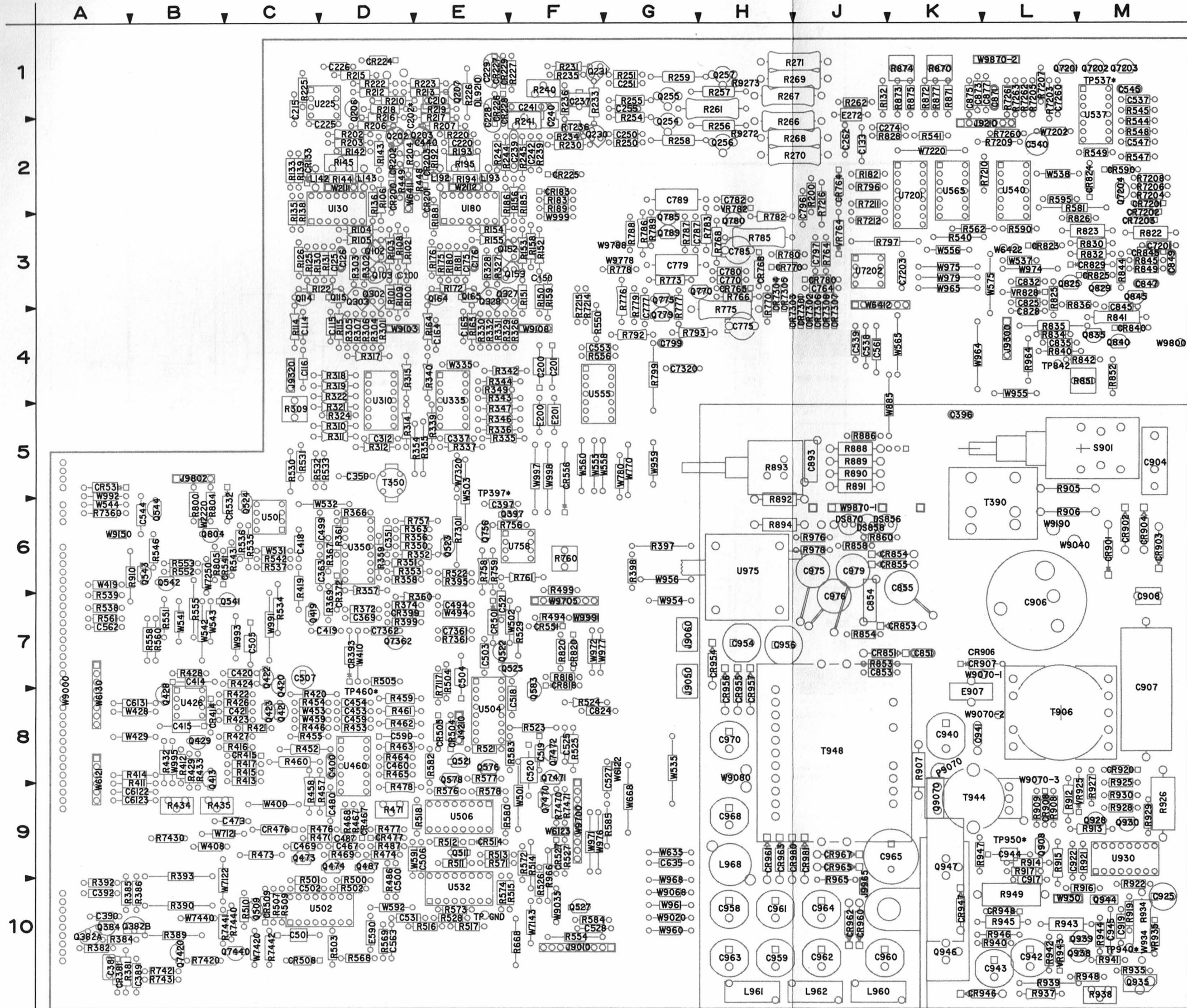
Figure 9-7. A1—Main board.
