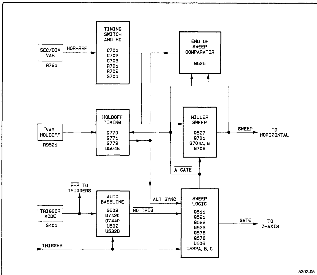
Figure 3-5. Sweep Generator and Logic circuitry.
