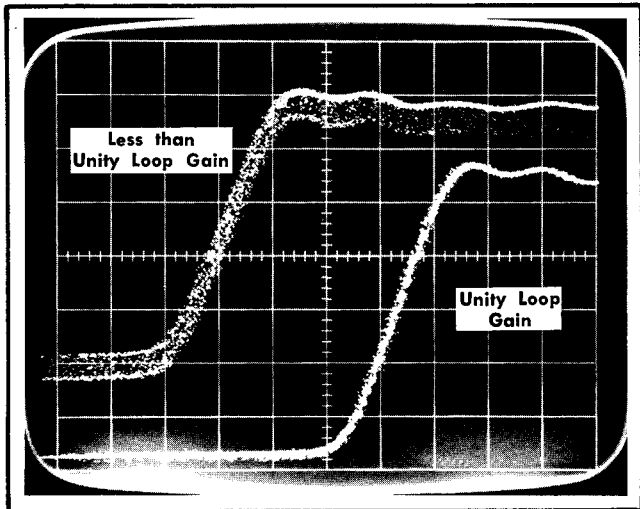
Fig. 5-9. Loop gain check in random sampling, before Trigger operation of the Type 3T2.
