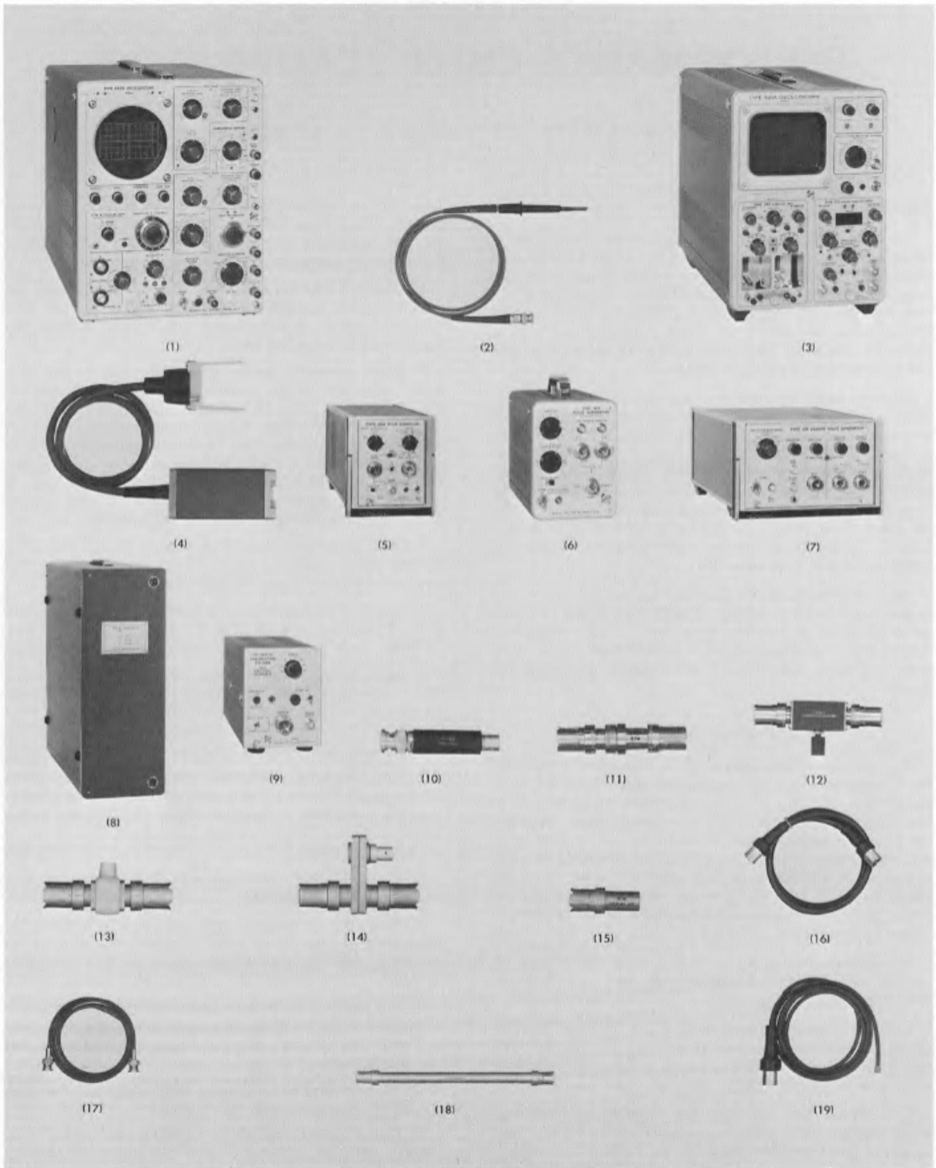
Fig. 5-1. Calibration Equipment.
