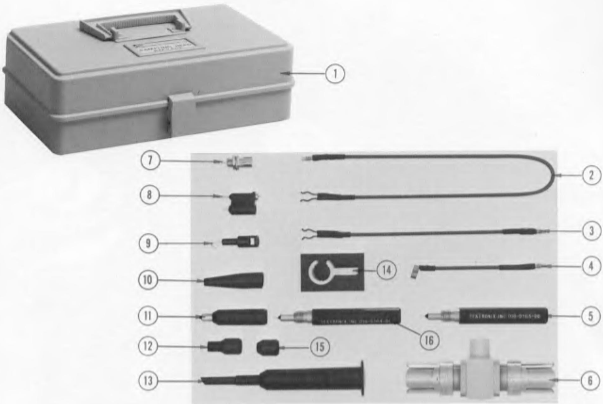
FIG. 2 STANDARD ACCESSORIES
