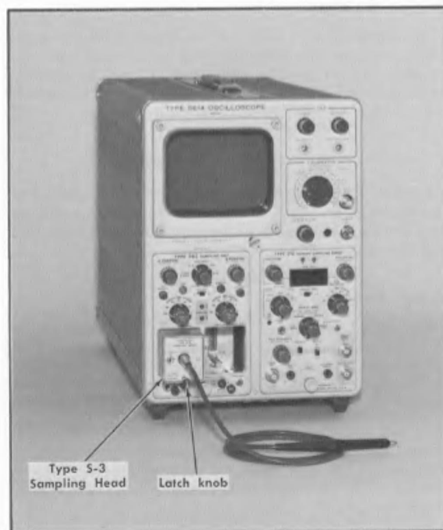
Fig. 2-1. Installation Information.
