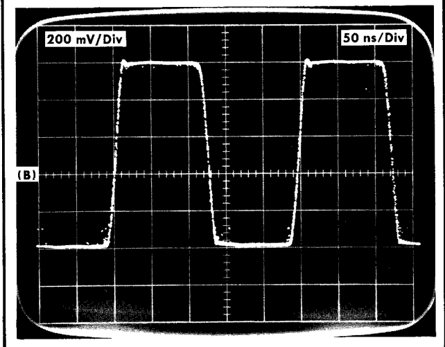
Fig. 2-6. Typical display for unity loop gain adjustment in random sampling operation.
