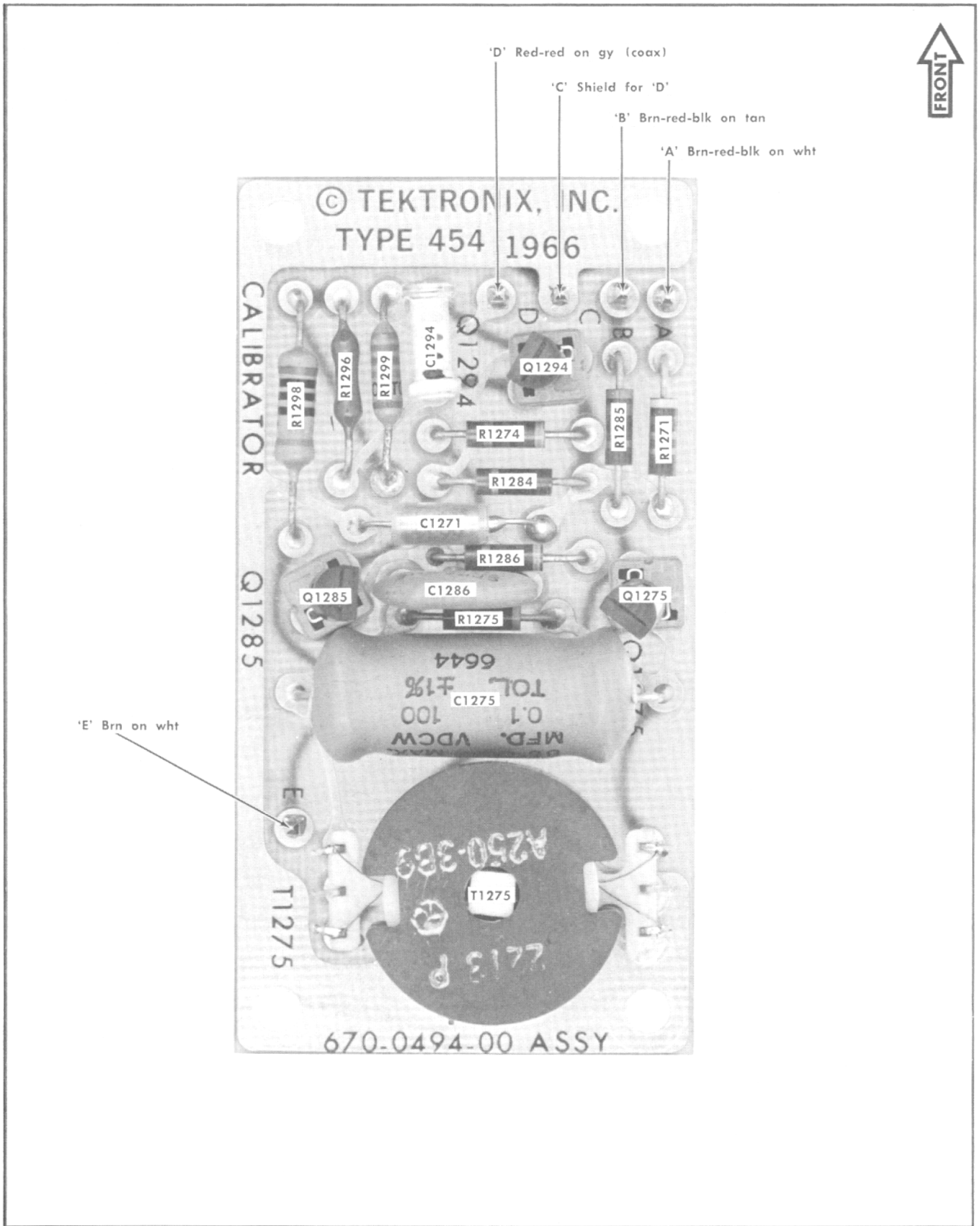
Fig. 4-18. Calibrator circuit board.
