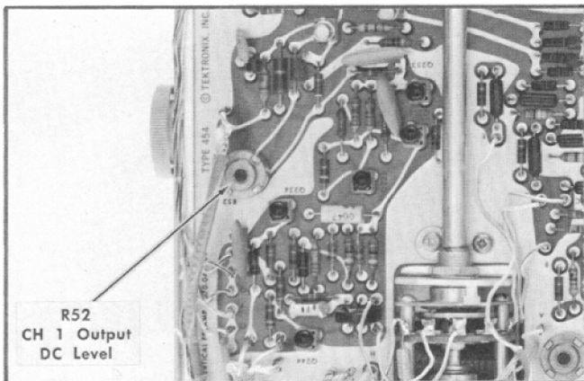
Fig. 6-34. Location of CH 1 output DC level adjustment (Vertical Preamp circuit board).
