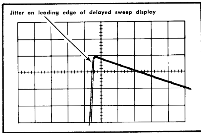
Fig. 5-22. Typical CRT display when checking delay-time jitter.
