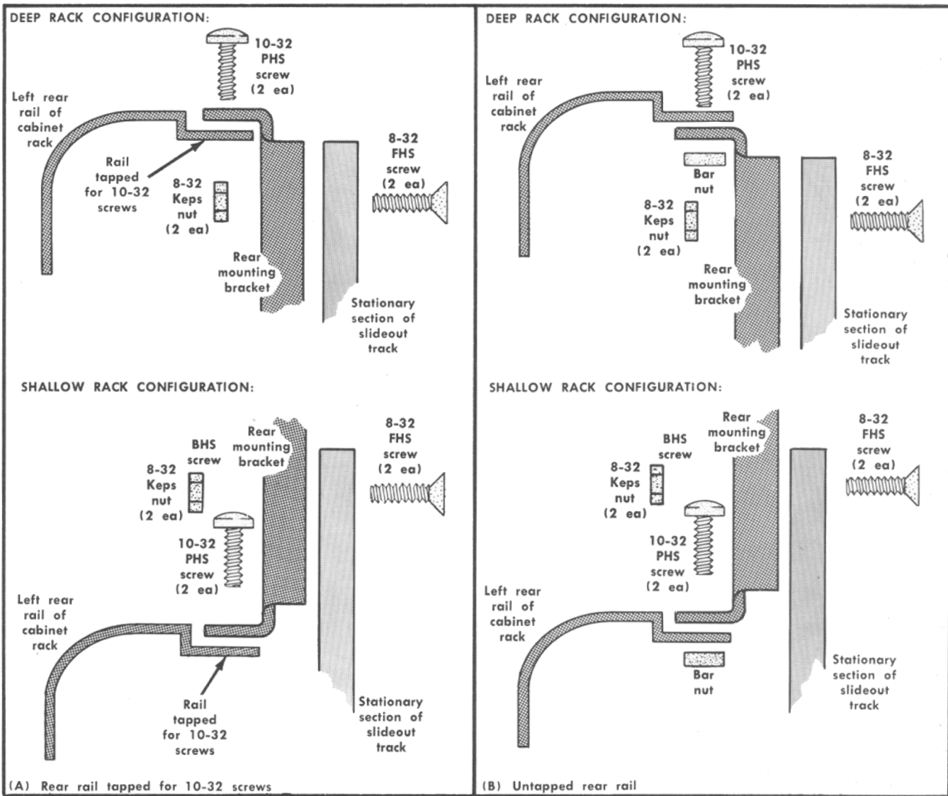
Fig. 10-11. Alternative method of installing the instrument using rear support brackets.
