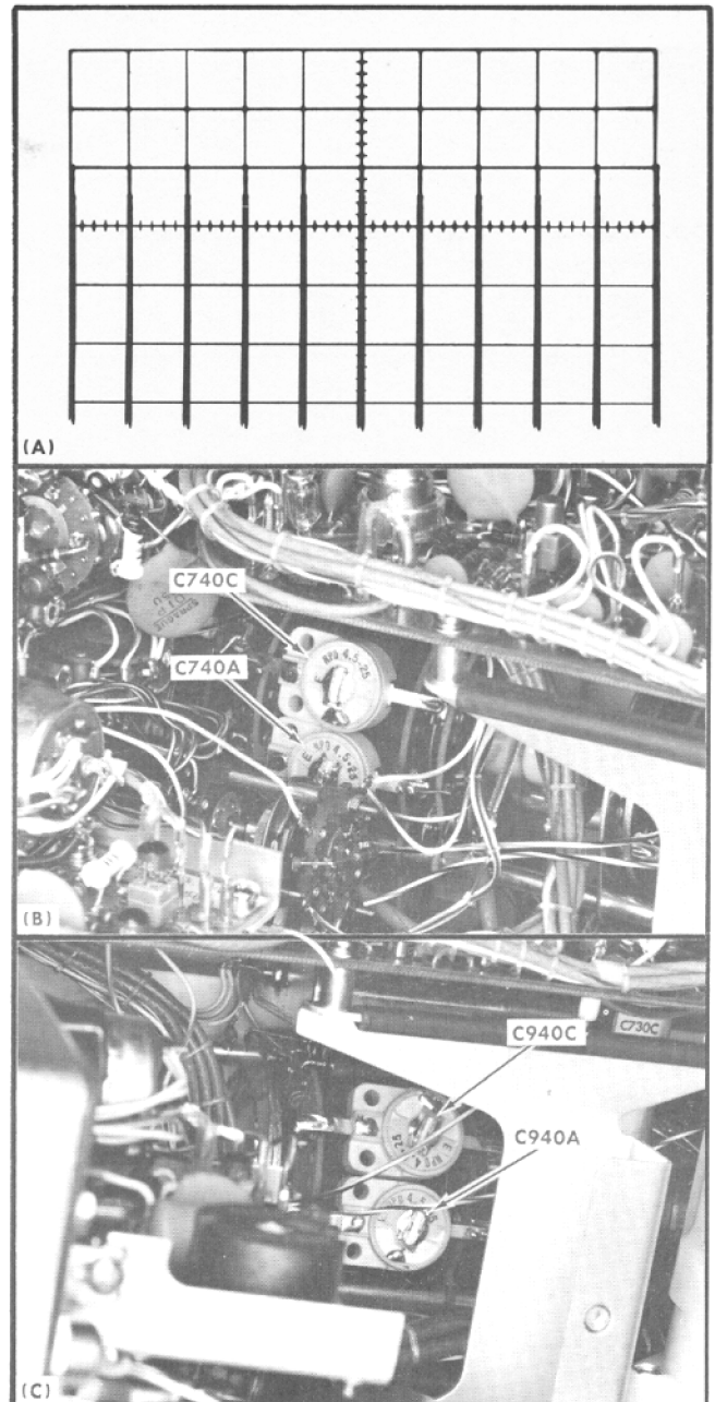
Fig. 6-51. (A) Typical CRT display showing correct one-microsecond timing, (B) location of C740A and C740C (behind swing-out side panel), (C) location of C940A and C940C (behind swing-out side panel).
