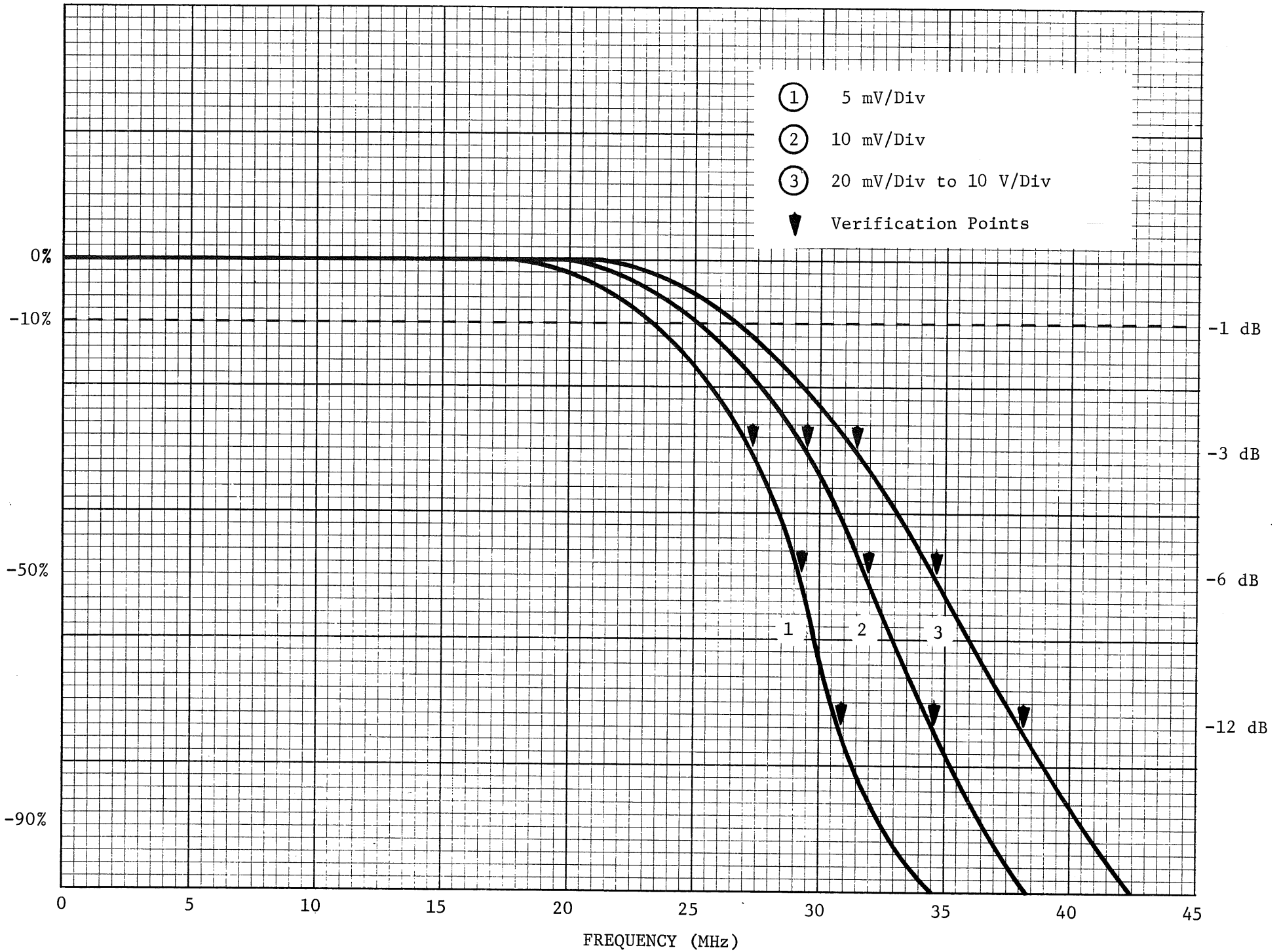
Fig. 1-1 Overall Frequency Response With P____ 1-5
