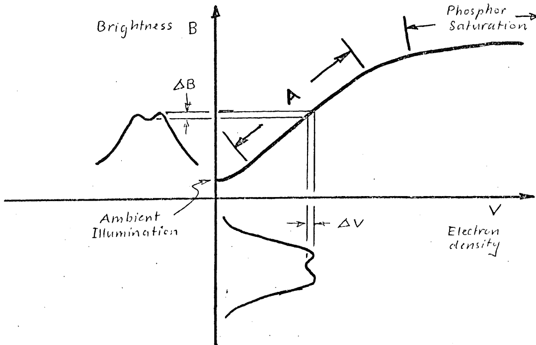
FIGURE 3. Phosphor Transfer Characteristic
