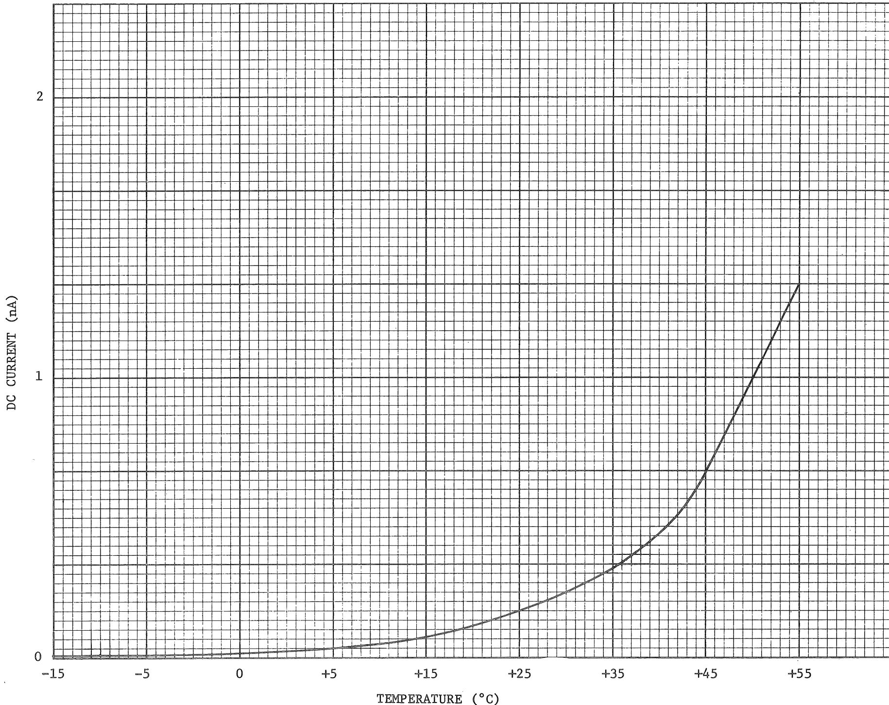
Fig. 1-5 Maximum DC Current vs Temperature
