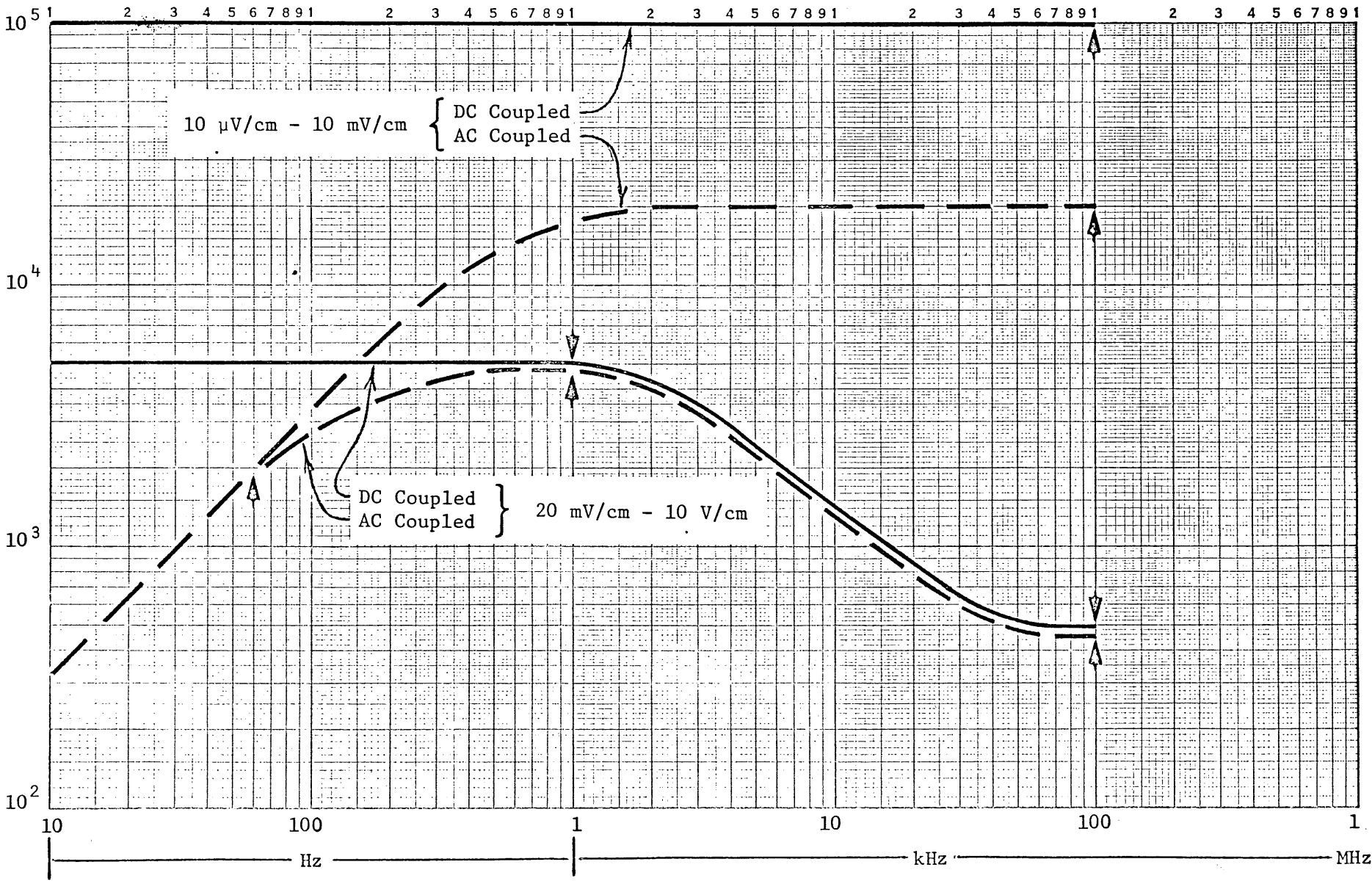
Fig. 1-3 CMRR vs Frequency
