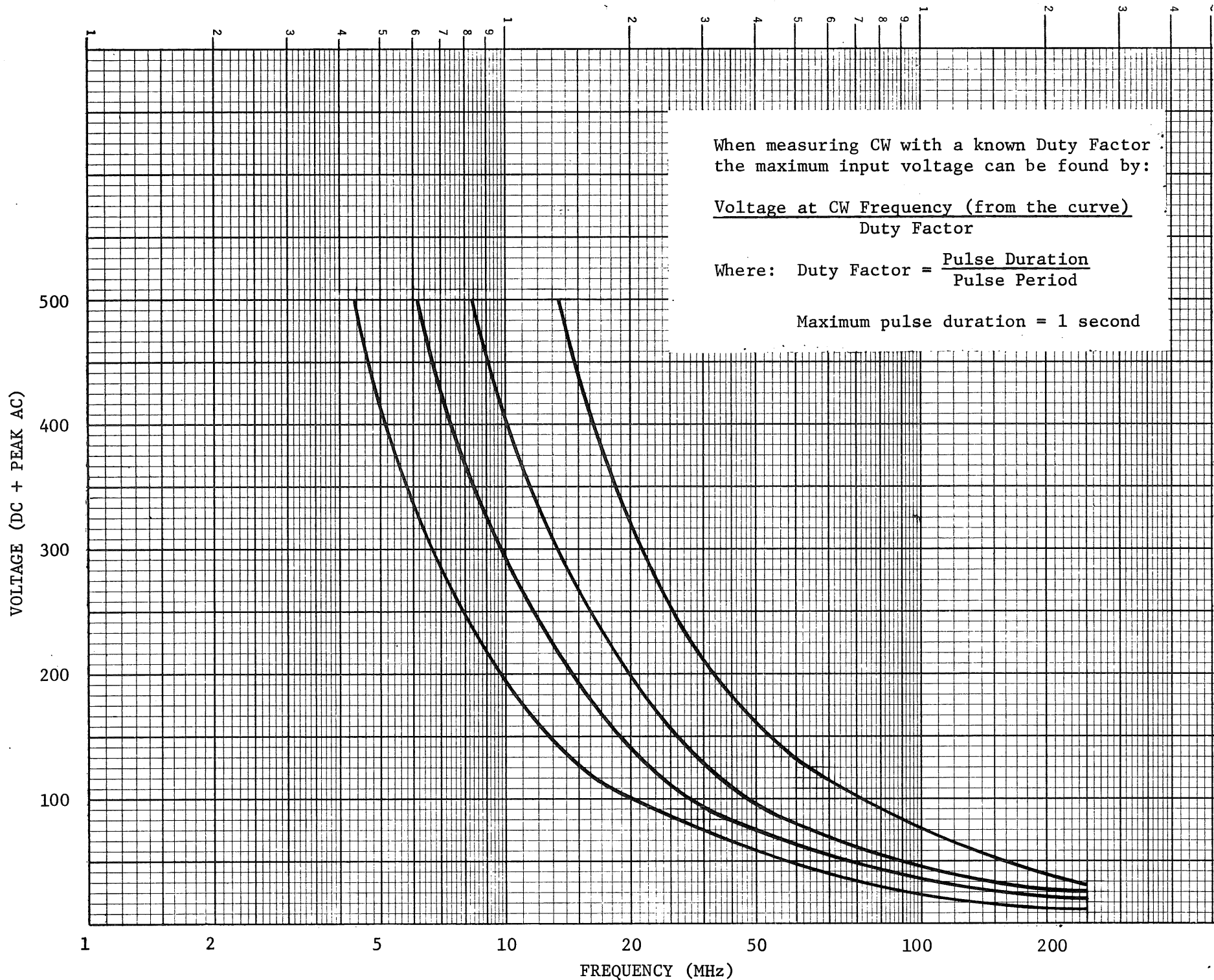
Fig. 1-4 Maximum Input Voltage Derating 1-11
