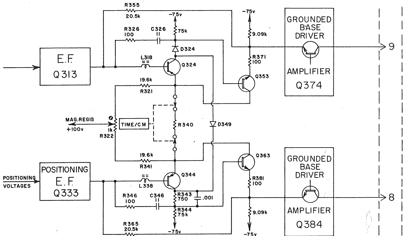
TYPE 11B1 HORIZONTAL PREAMPLIFIER PARAPHASE AMPLIFIER
