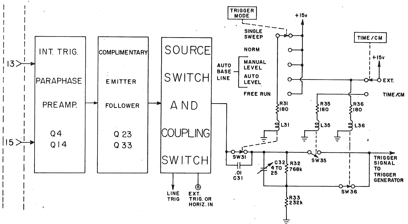
TYPE IIBI INTERNAL TRIGGER PREAMPLIFIER AUTO SELECTION
