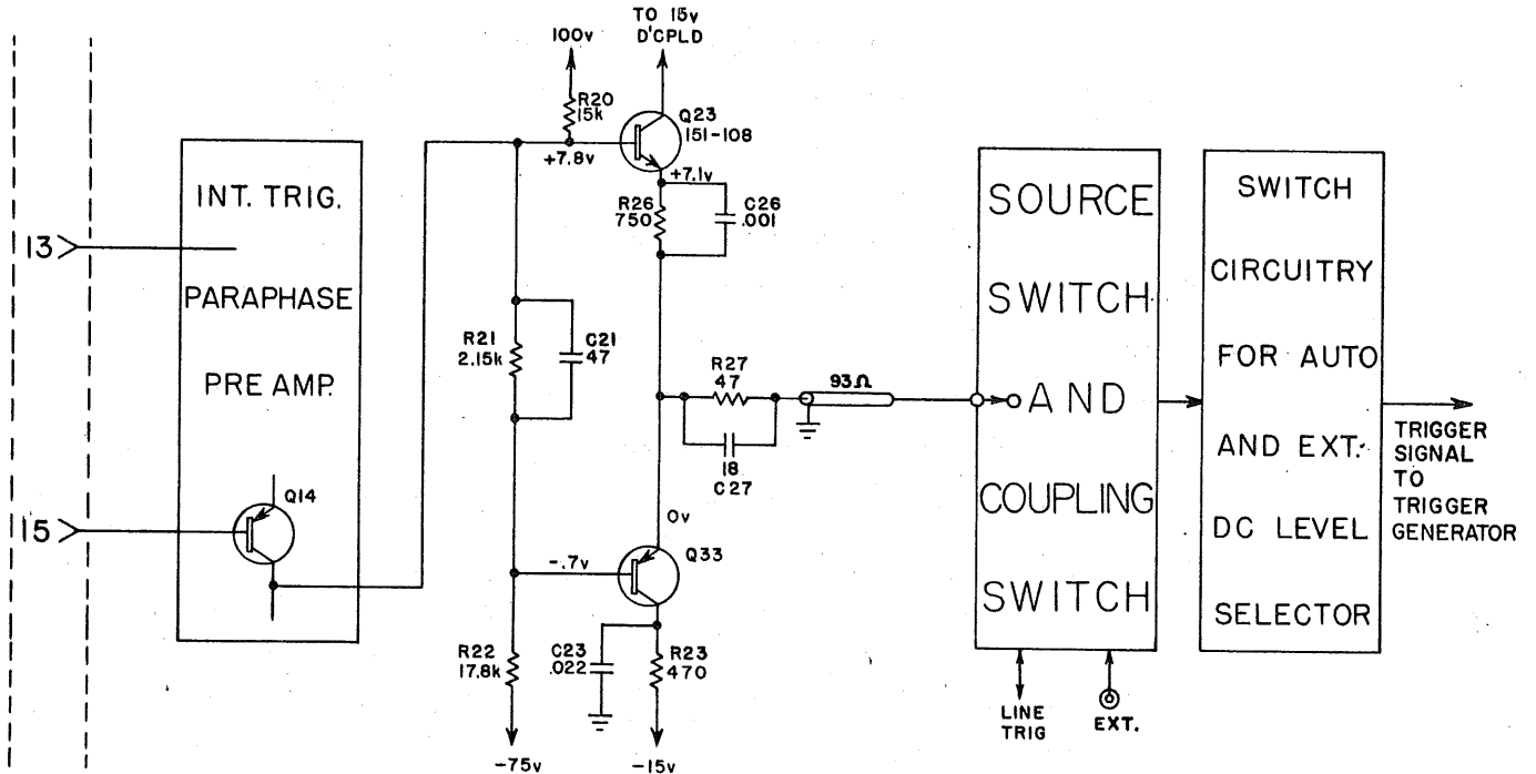
TYPE IIB1 INTERNAL TRIGGER PREAMPLIFIER COMPLIMENTARY EMITTER FOLLOWER
