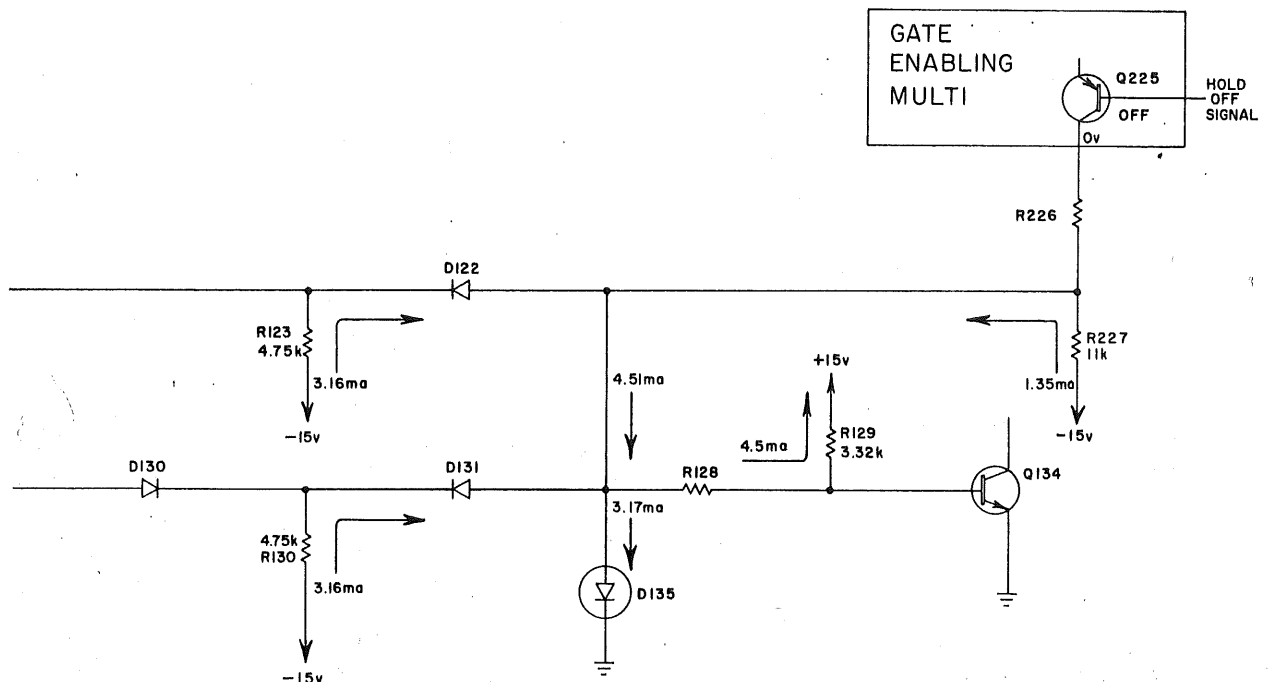
TYPE IIBI SWEEP GENERATOR CURRENT DISTRIBUTION
