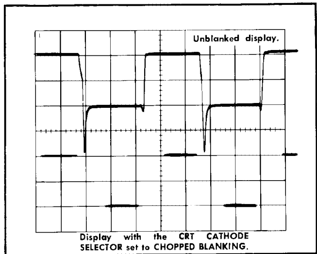
Fig. 2-6. Double-exposure photograph showing the effect of setting the CRT CATHODE SELECTOR to CHOPPED BLANKING. (The waveform was moved from the upper to the lower portion of the graticule area for the second exposure.)
