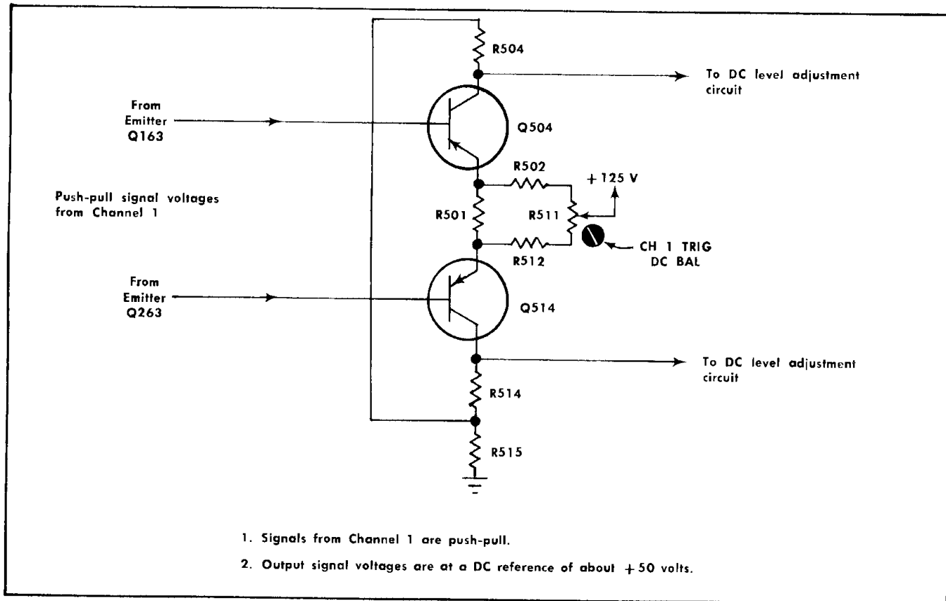
Fig. 3-13. Partial diagram showing the Channel 1 Trigger Amplifier.
