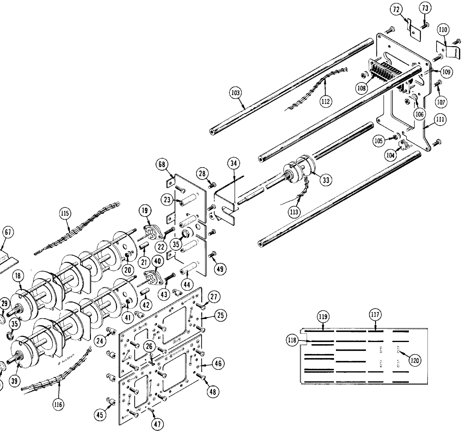
FIG. 1 EXPLODED VIEW
