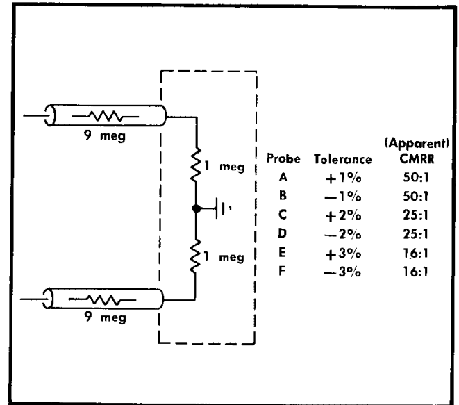
Fig. 2-9. Simplified input circuit and table to show the change in CMRR (apparent) due to 10X probes that are within 1, 2, and 3% of their attenuation values (with matched 1 meg resistors).
