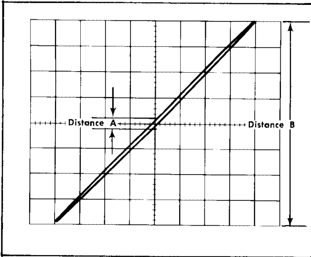
Fig. 2-16. Photograph of the lissajous pattern produced when a common sine-wave is applied to two Type 3A3 Plug-In Units that have approximately 2° of phase difference.
