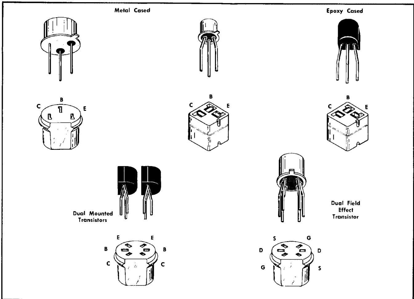
Fig. 4-3. Transistor socket and transistor lead configuration top view.
