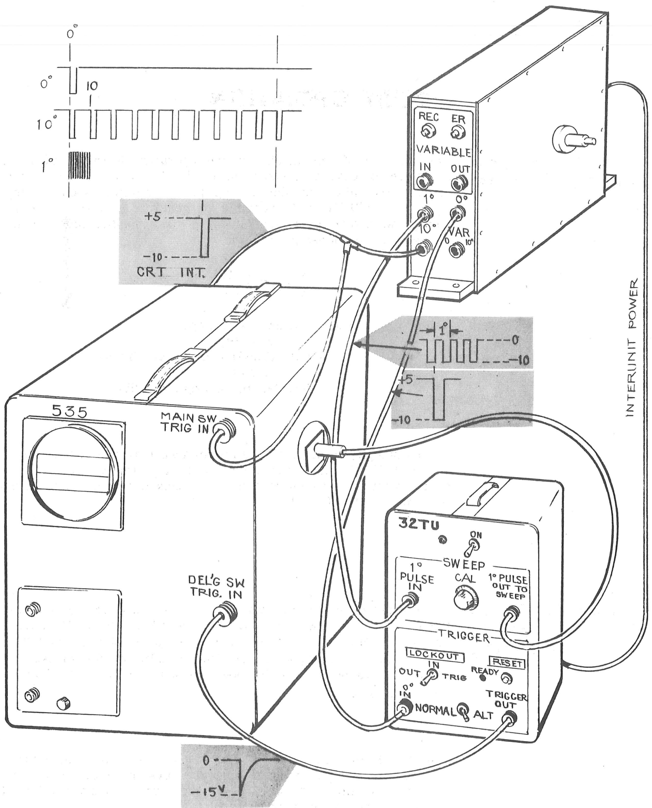
Fig. 10 ROTAN Cabling.
