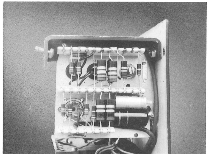
Trigger Chassis
