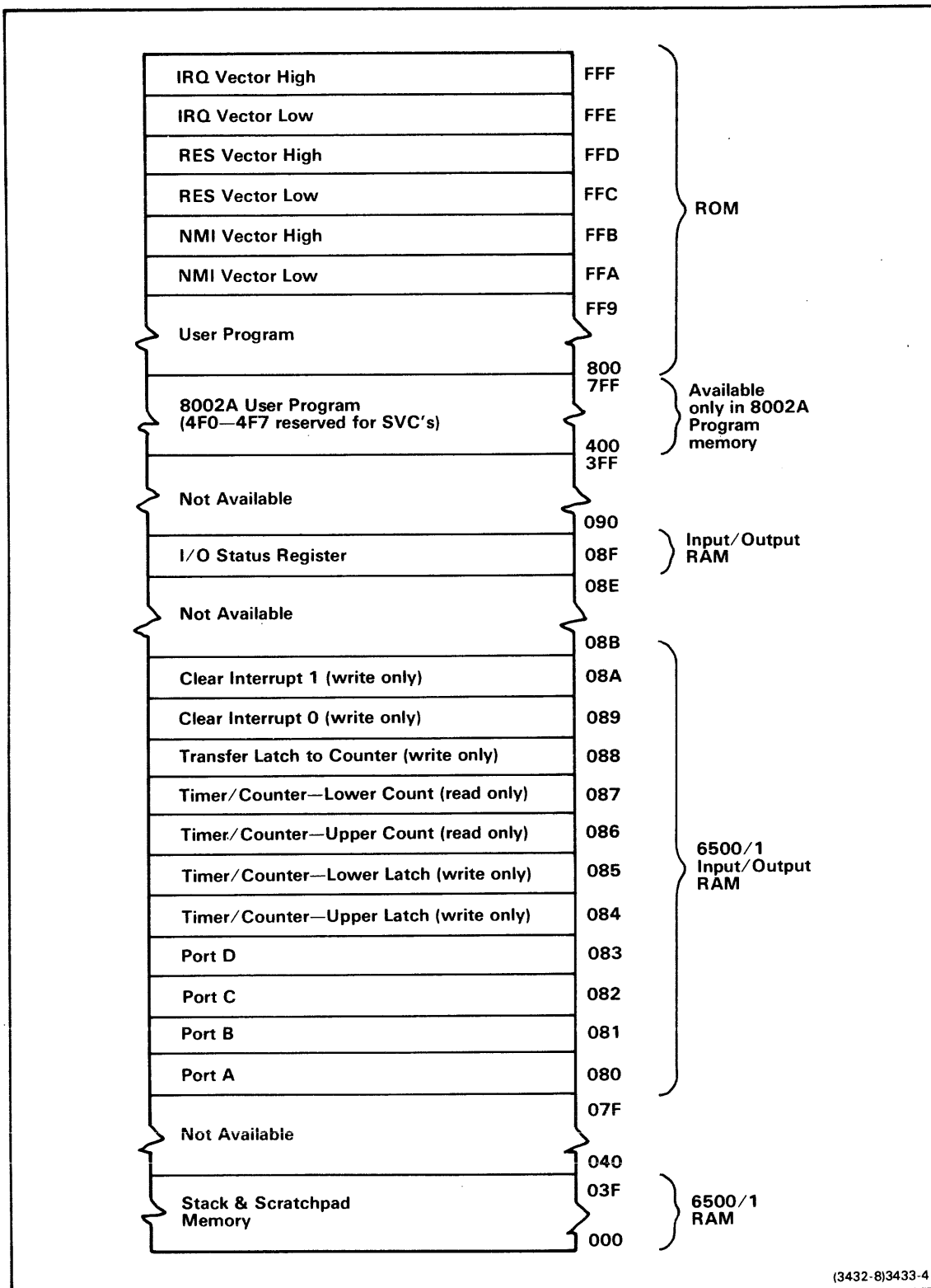
Fig. 9-18. 6500/1 Memory Allocation.
