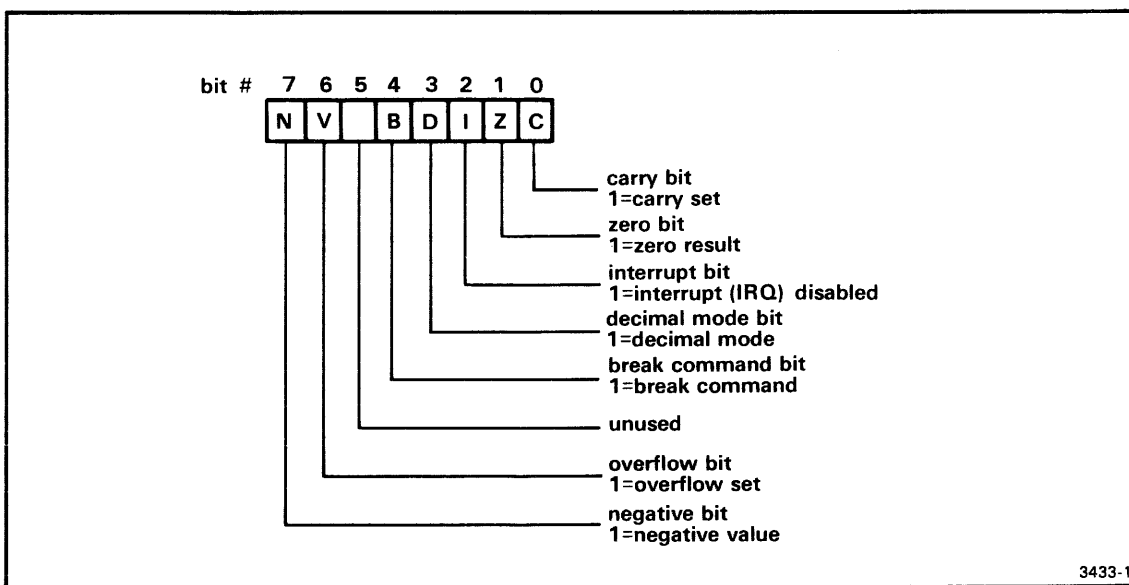
Fig. 9-15. 6500/1 Status Register.
