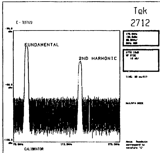
Figure 6-10. 2712 plot with title and plot labels.
