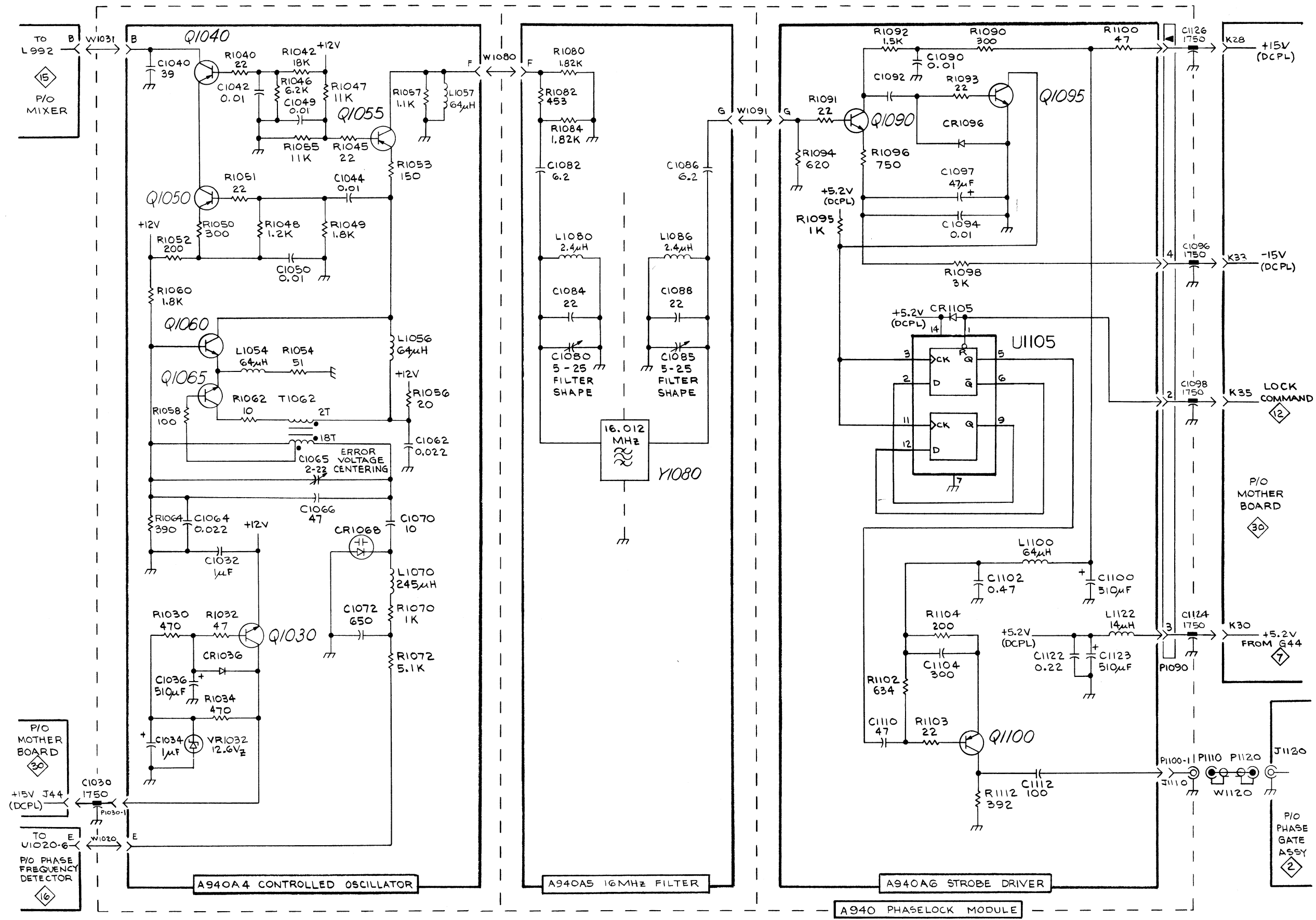
CONTROLLED OSCILLATOR, 16MHz FILTER & STROBE DRIVER
