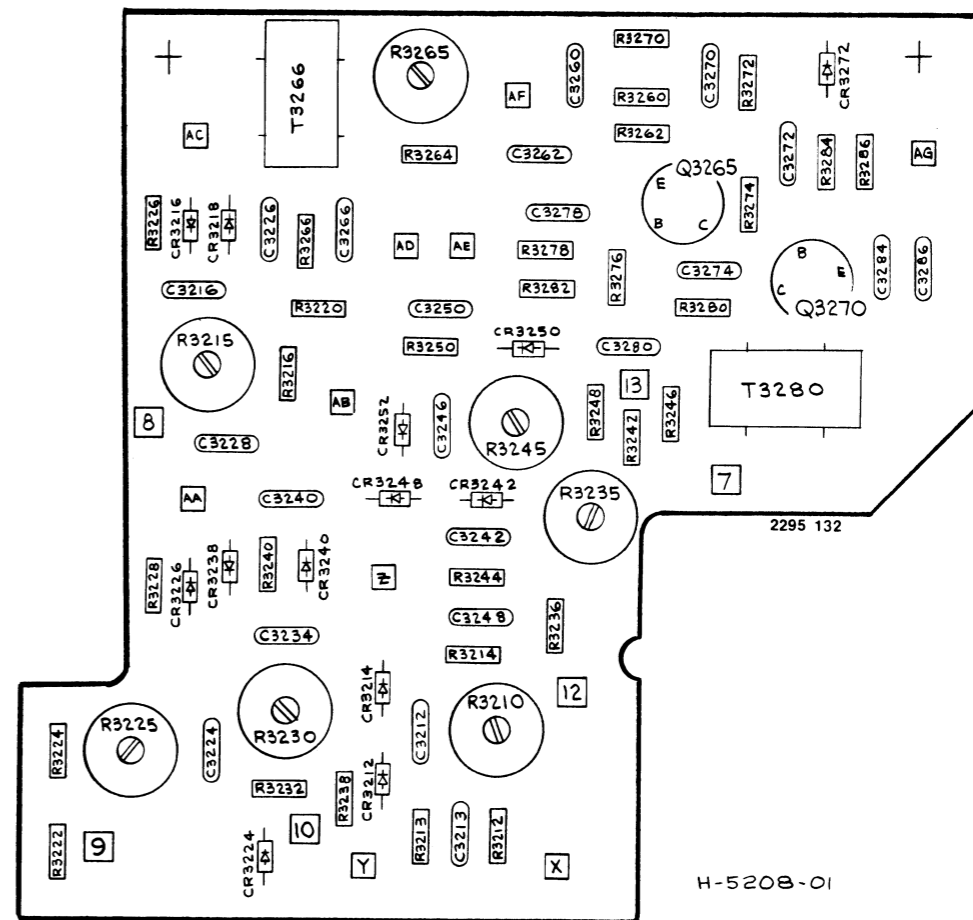
7L18 A3000A5 POST VARIABLE RESOLUTION AMPLIFIER 2295 132
