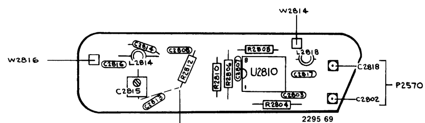
H-5039-01 J2816 7L18 A2690A2 WAVEGUIDE BAND RESONATOR
