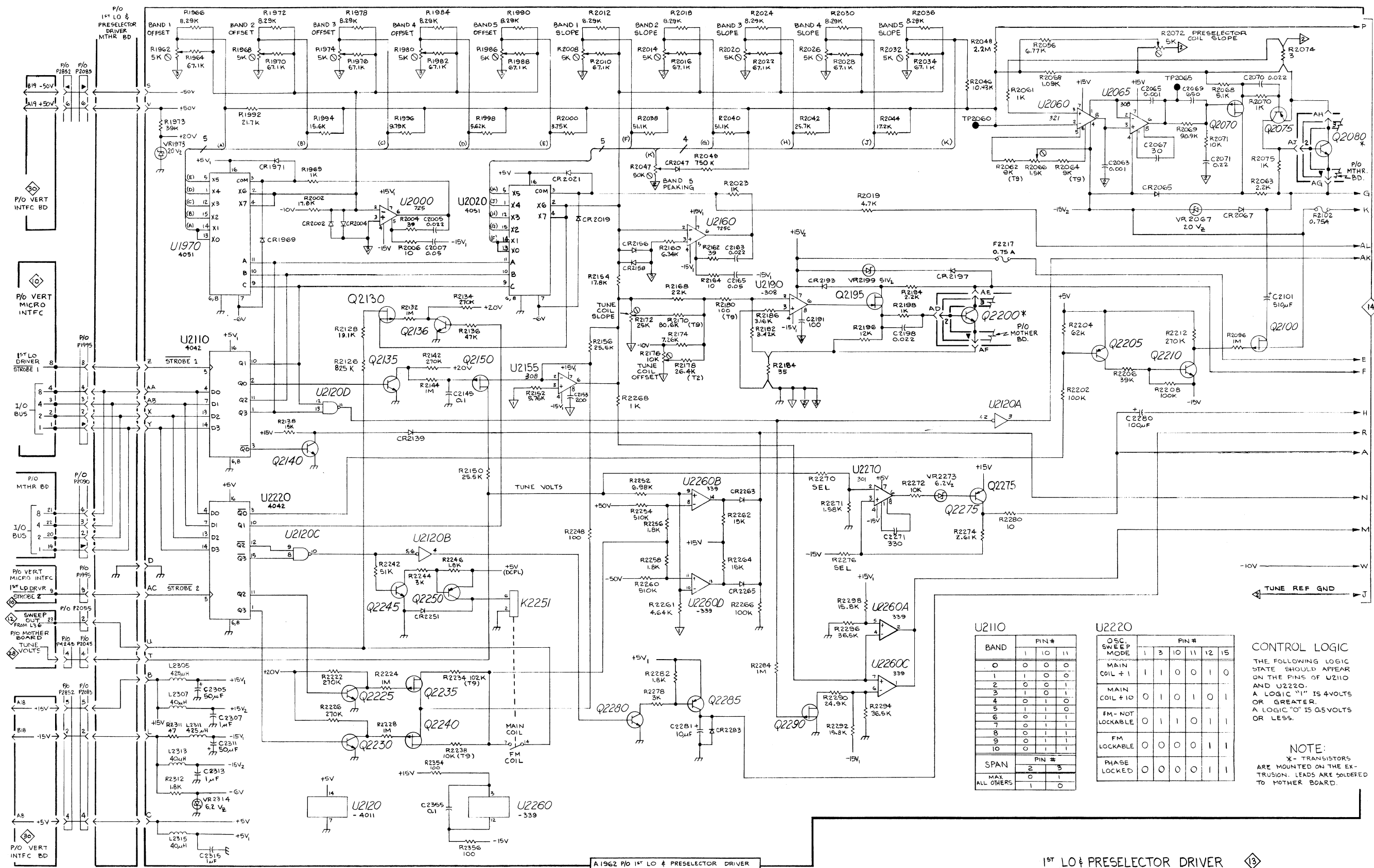
A1962 P/O 1ST LO & PRESELECTOR DRIVER
