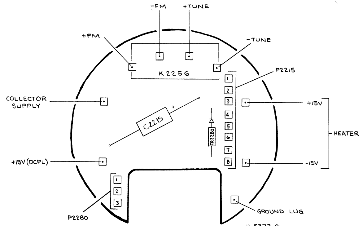
7L18 A60A1 1ST LO BOARD
