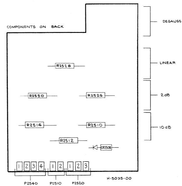
7L18 A2500 DISPLAY MODE SWITCHES (BOTTOM) H-5035-00
