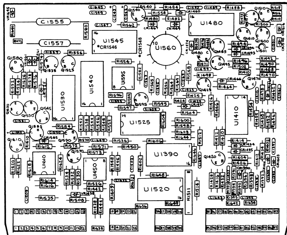
7L18 H-5022-01 A1390 HORIZONTAL SWEEP 2295 88
