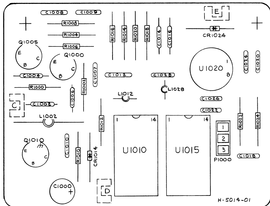
7L18 A940A3 PHASE/FREQUENCY DETECTOR
