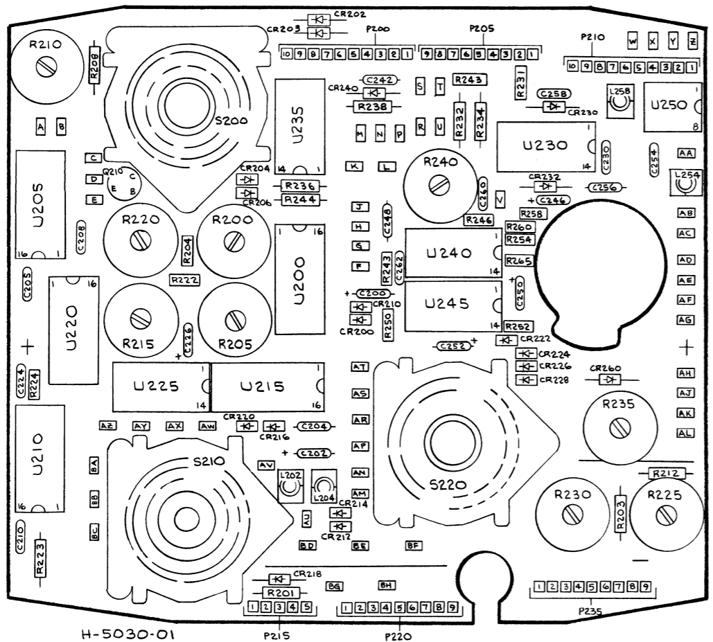
7L18 A100A2 FRONT PANEL BOARD # 2
