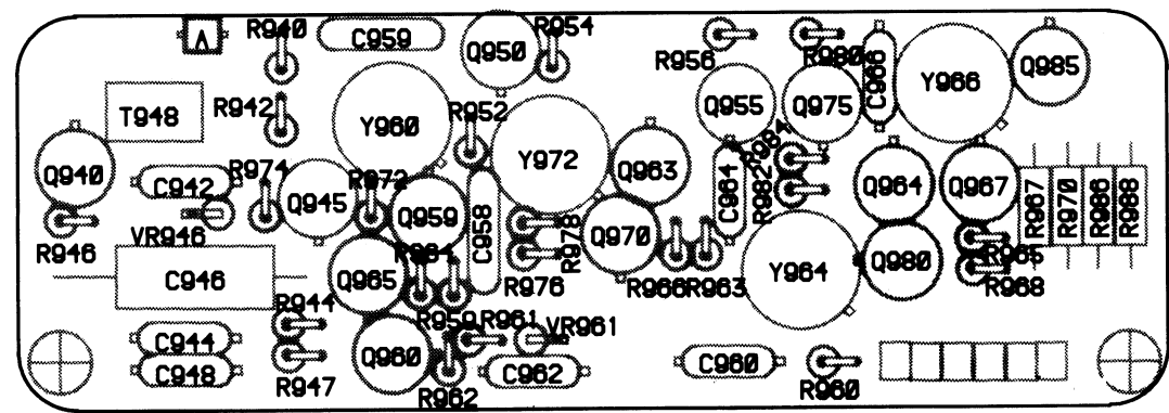
2295 97 A940A1 H-5013-02 REFERENCE OSCILLATOR
