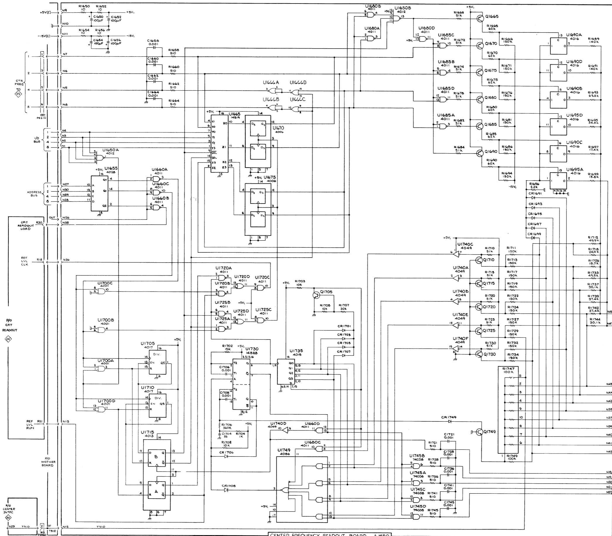
CENTER FREQUENCY READOUT BOARD A1650
