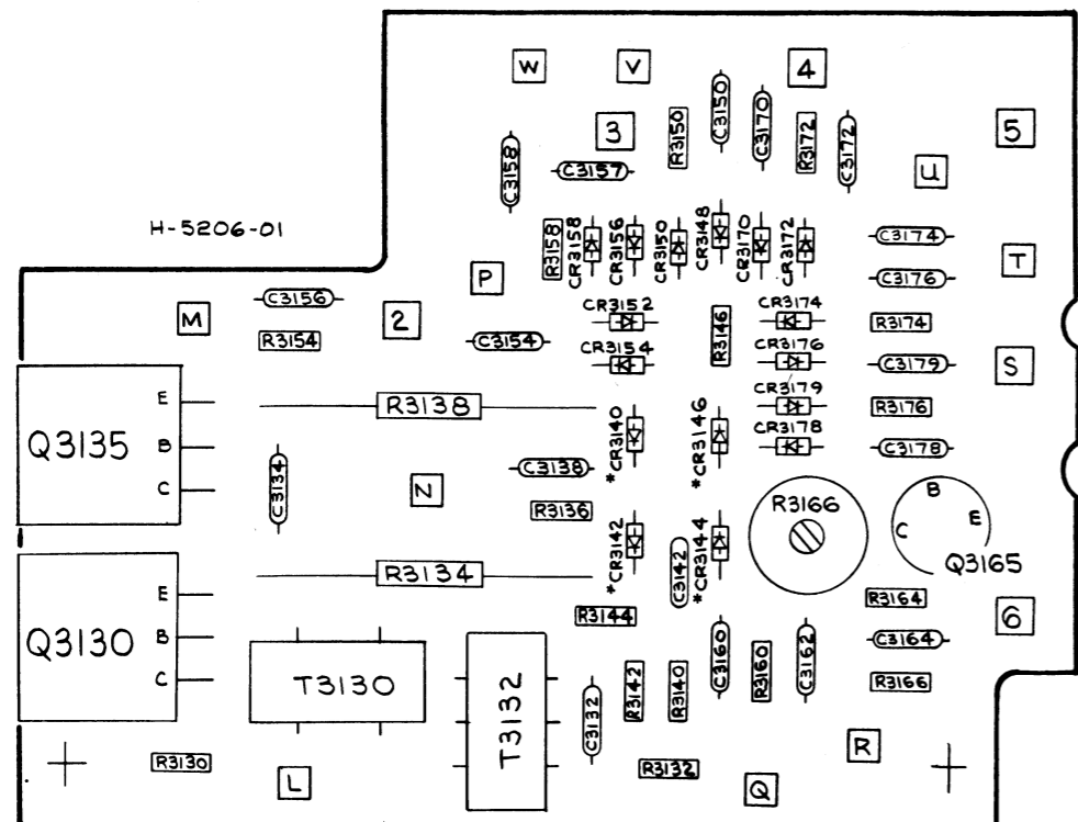
7L18 A3000A3 VARIABLE RESOLUTION AMPLIFIER 2295 77
