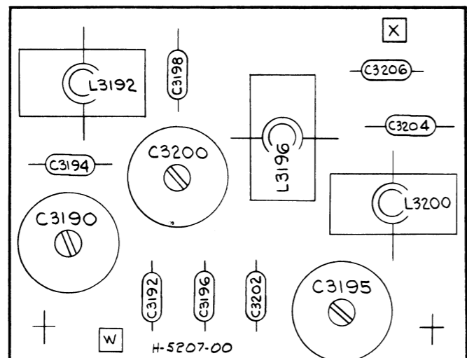
7L18 A3000A4 300kHz FILTER 2295 78
