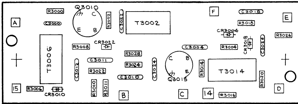
7L18 A3000A1 VARIABLE RESOLUTION INPUT H-5204-01
