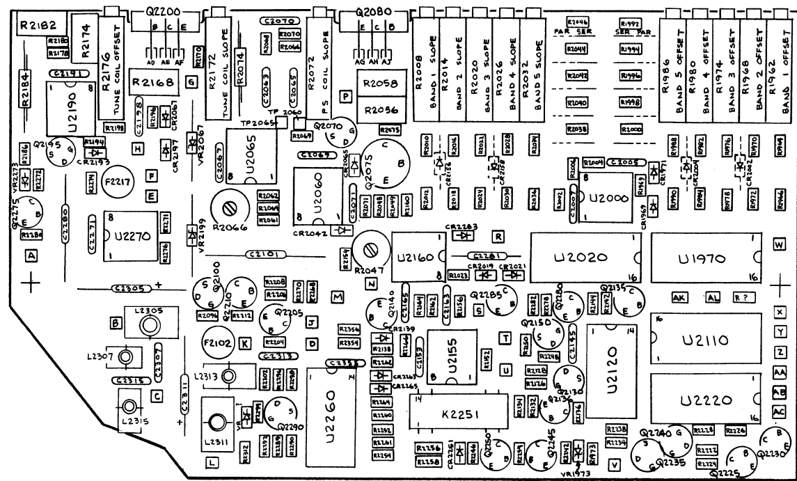
7L18 H-5032-01 A1962 1 ST LO/PRESELECTOR DRIVER
