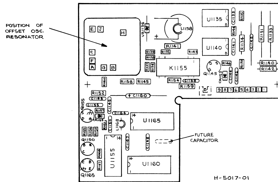
7L18 A940A7A1 OFFSET OSCILLATOR
