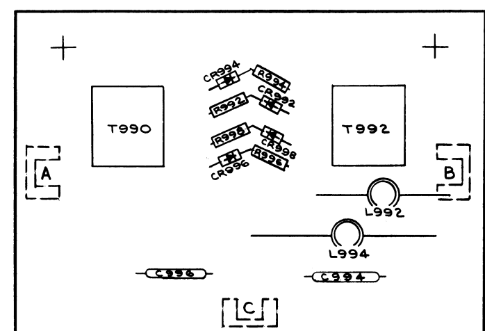
2295 98 H-5013-01 A940A2 MIXER
