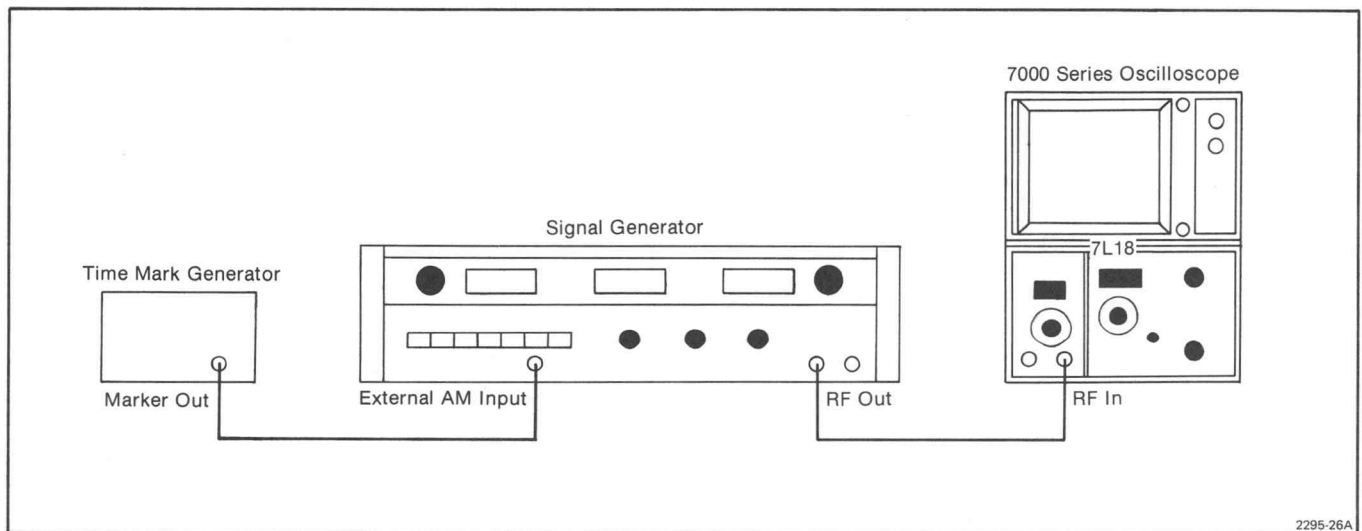
Fig. 4-18. Sweep Rate Test Setup.
