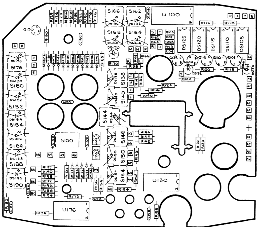
7L18 H-5025-01 A100AI FRONT PANEL BOARD #1
