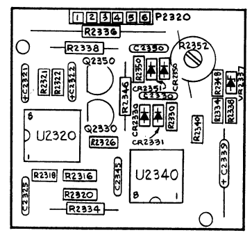
H-5026-01 7L18 A2316 REFERENCE VOLTAGES
