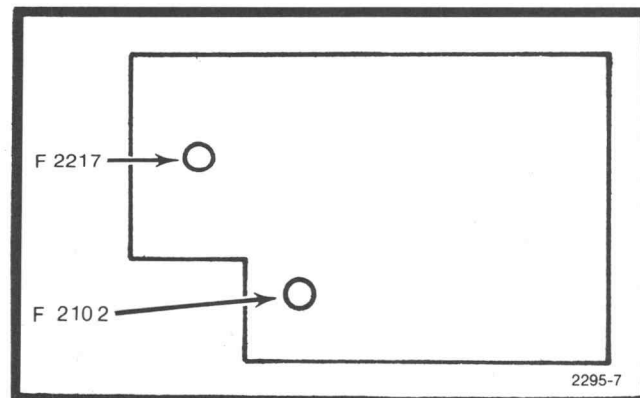
Figure 3-3. Location of F2217 and F2102 on First LO and Preselector Driver Board.
