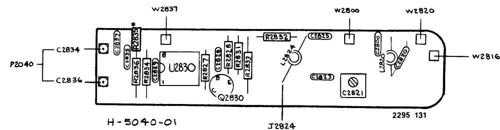
H-5040-01 J2824 7L18 A2690A3 COAXIAL BAND RESONATOR
