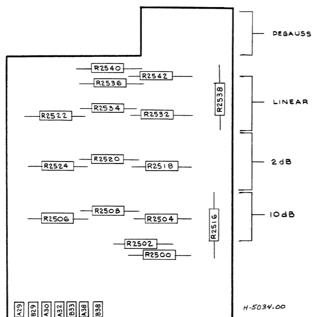
7L18 A2500 DISPLAY MODE SWITCHES (TOP) H-5034-00
