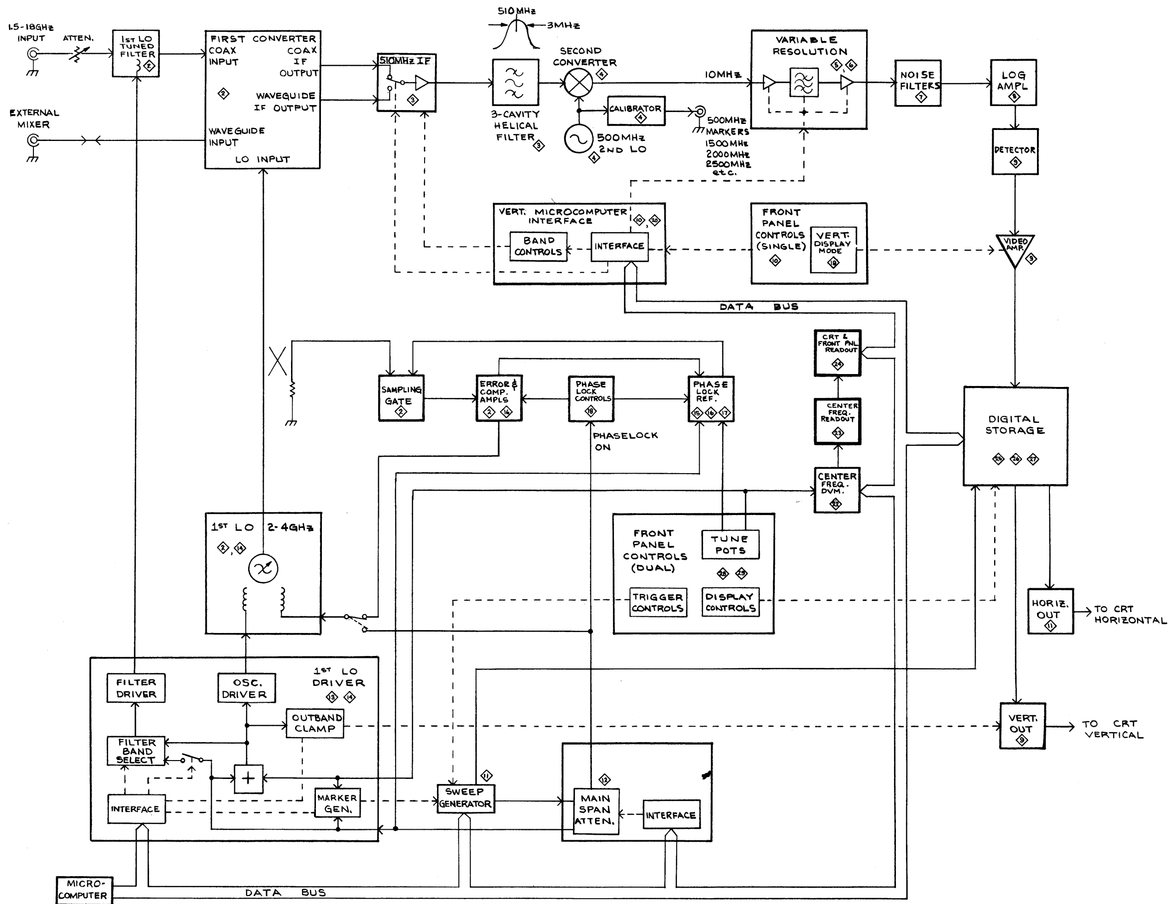
7L18 SIMPLIFIED BLOCK DIAGRAM
