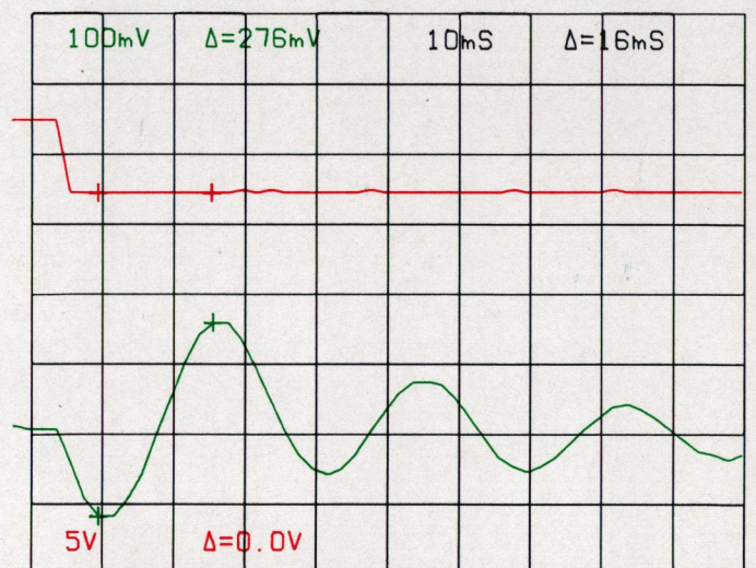
Figure 3. A 10X magnification of the waveforms shown in Figure 2. Magnification is referenced to cursor number one.
