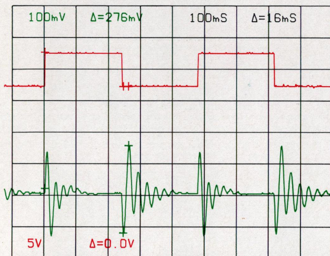
Figure 2. Example of dual channel output with cursor positions indicated by + mark. (See Figure 3 for magnification of this waveform.)
