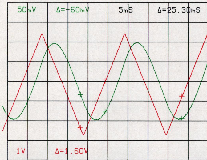
Figure 1. X-Y Recorder Output of two signals captured simultaneously. Channel one is shown in green, channel two in red.
