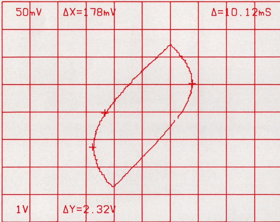
Figure 4. X-Y display. Channel one shown as X data, channel two; Y data.
