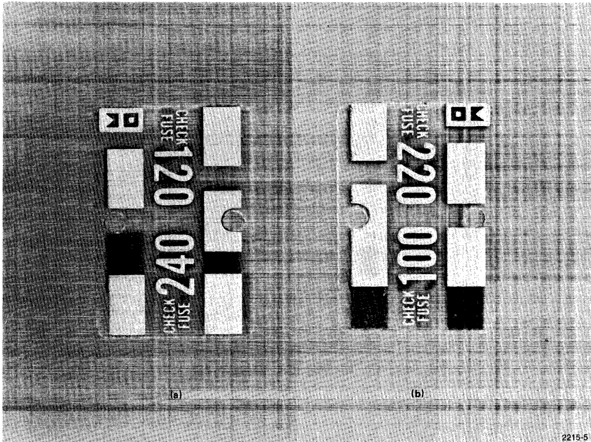
Fig. 2-3. Circuit Card.
