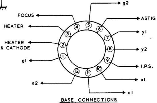
POWER SUPPLY & C.R.T. - D61
