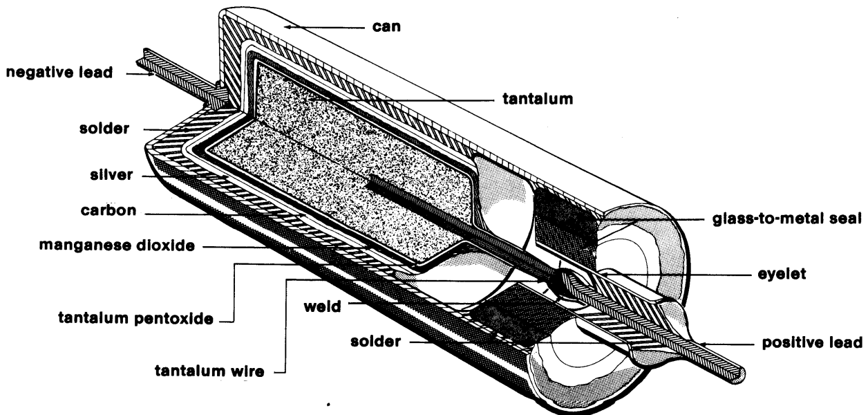
Figure 1 Hermetically sealed, axial lead tantalum capacitor
