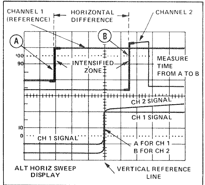
Figure 6-16. Time between two time-related pulses.
