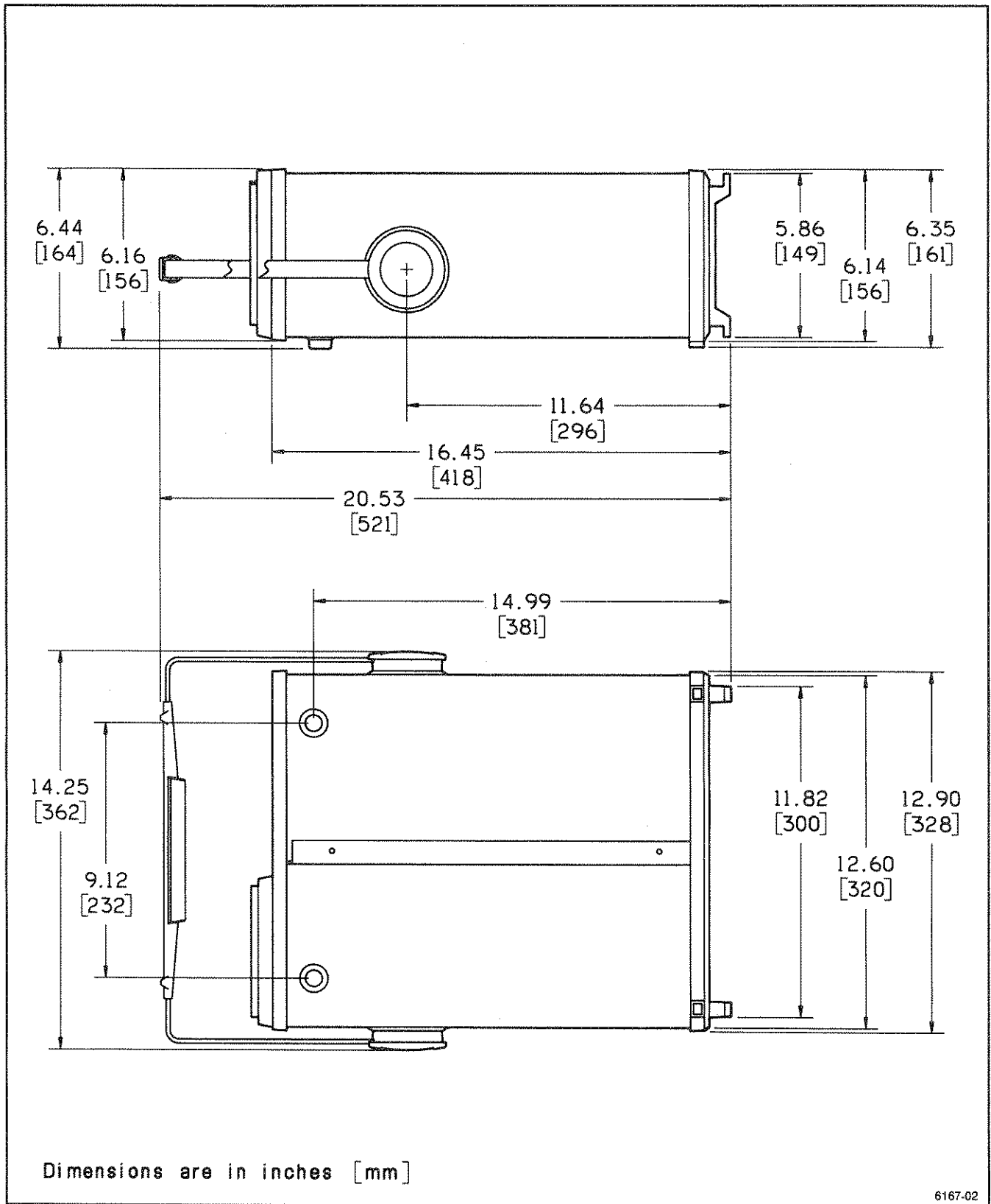
Figure 1-1. Dimensional drawing.
