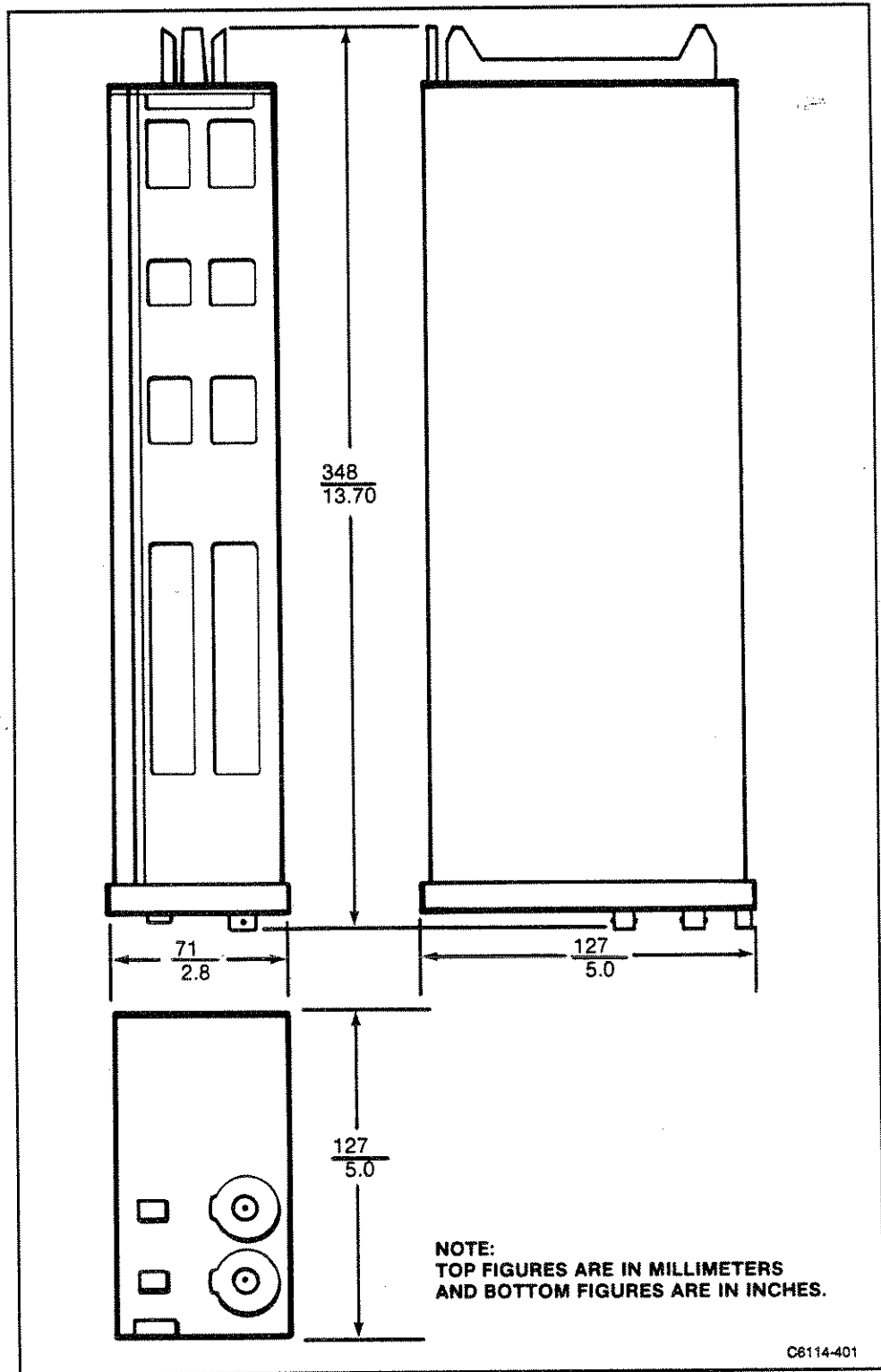
Figure 4-1. Dimensions of 11A52.
