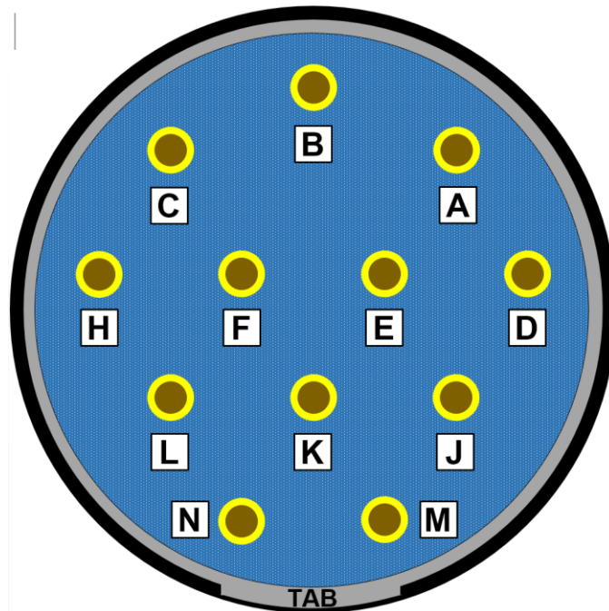
AM503B and AM5030 AMPHENOL 165-15 CONNECTOR FRONT VIEW
