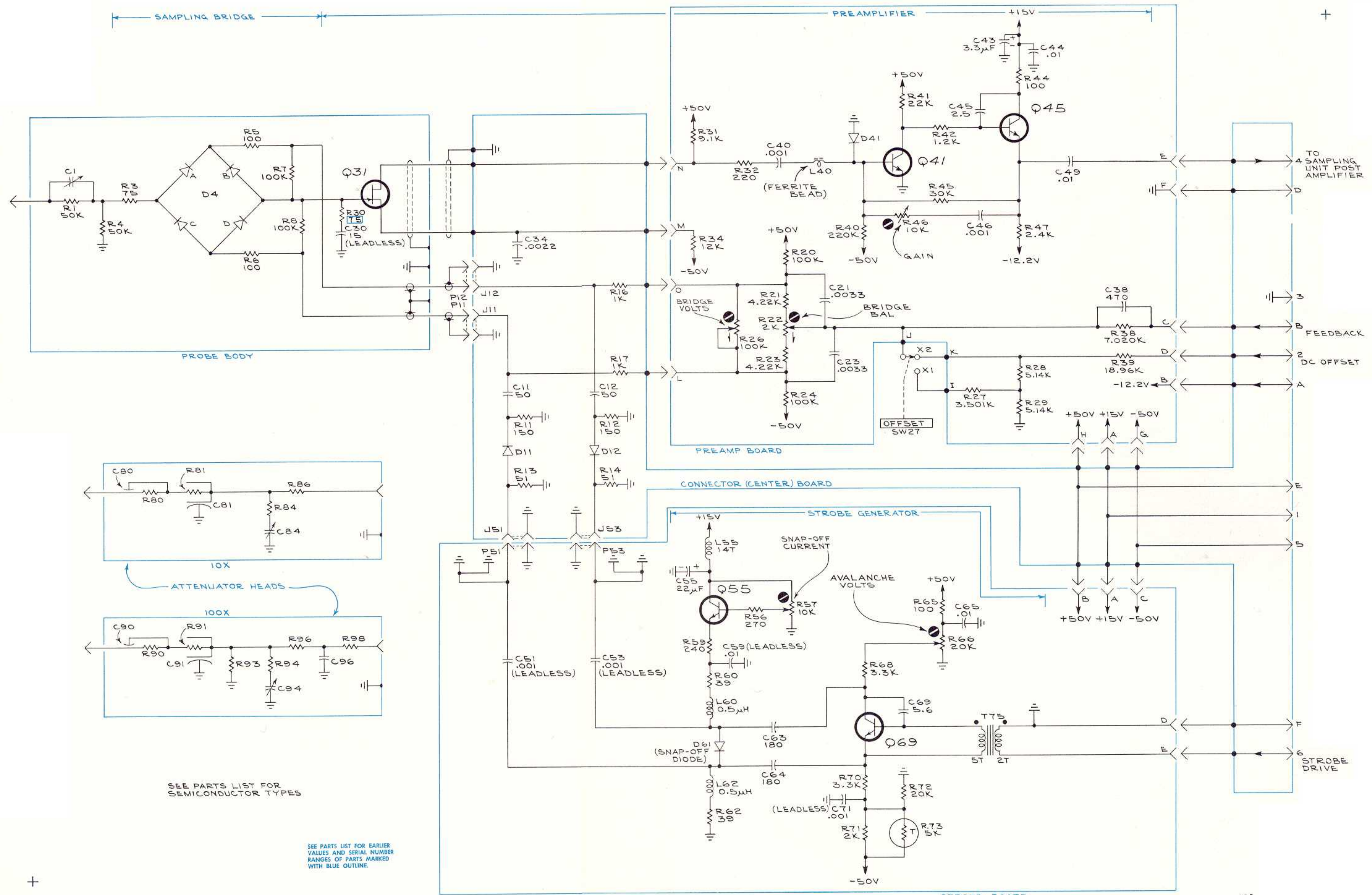
TYPE S-3 SAMPLING HEAD
