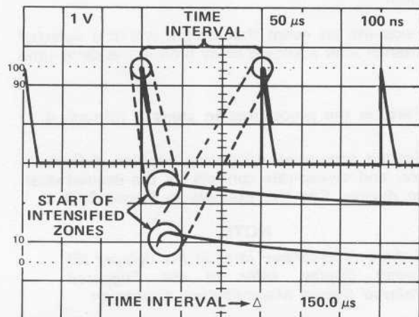
TIME-INTERVAL MEASUREMENT BETWEEN TWO PULSES IN THE \Delta (DIFFERENTIAL) TIME MODE.
