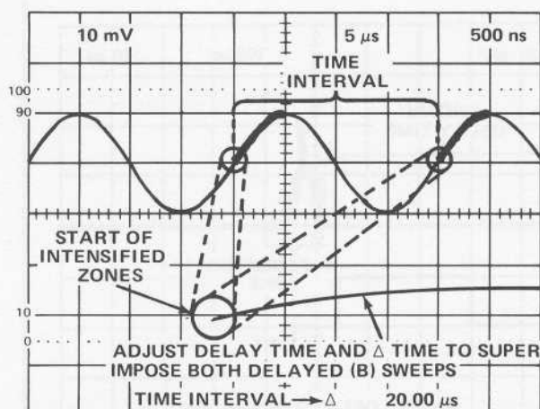
TIME INTERVAL MEASUREMENT BETWEEN TWO IDENTICAL POINTS ON A SINE WAVE IN THE \Delta (DIFFERENTIAL) TIME MODE.
