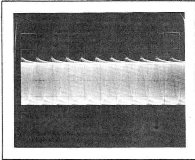
FIG. 2 10 \mu s/cm showing 10 beats in less than 10 cm. 3 MHz is approximately 100 kHz high.
