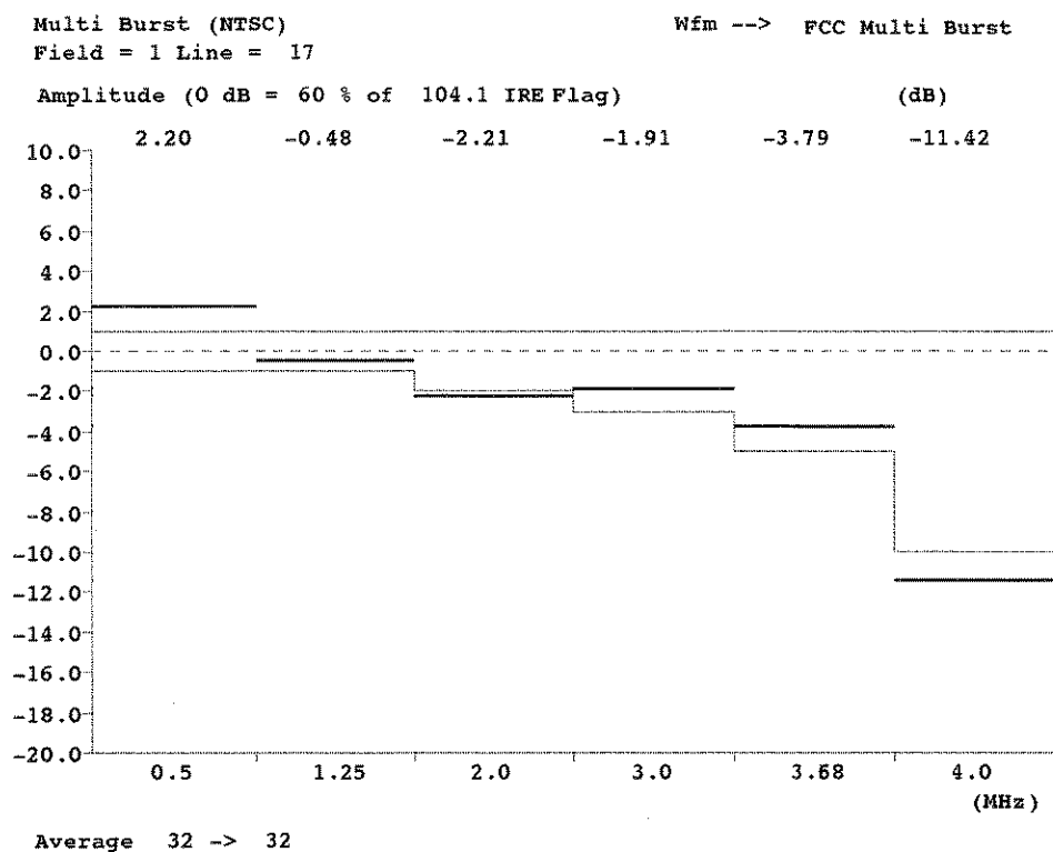
Figure 2-57: MultiBurst display
