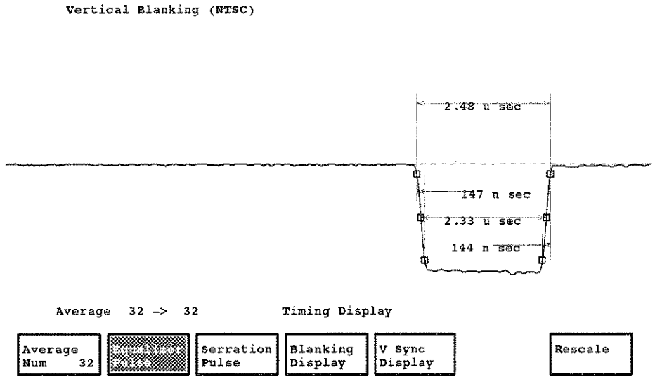
Figure 2-80: V_Blank equalizer pulse display
