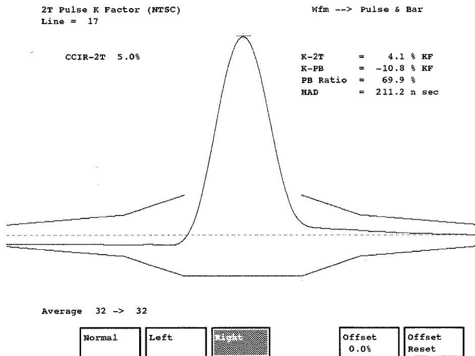
Figure 2-43: K_Factor measurement right reference clamped
