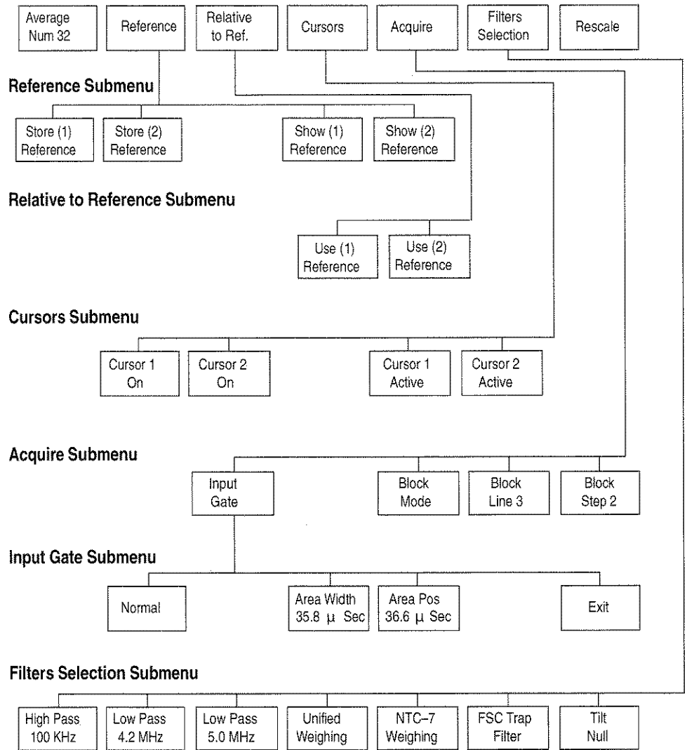
Figure 2-61: Noise Spectrum menu tree
