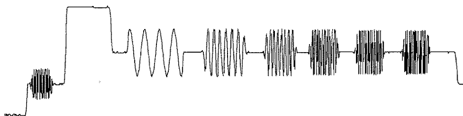
Figure 2-76: VITS_ID signal ID display
