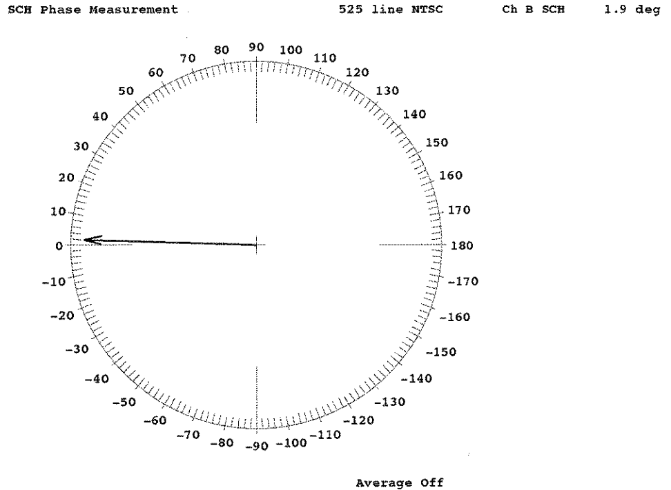
Figure 2-64: SCH_Phase display
