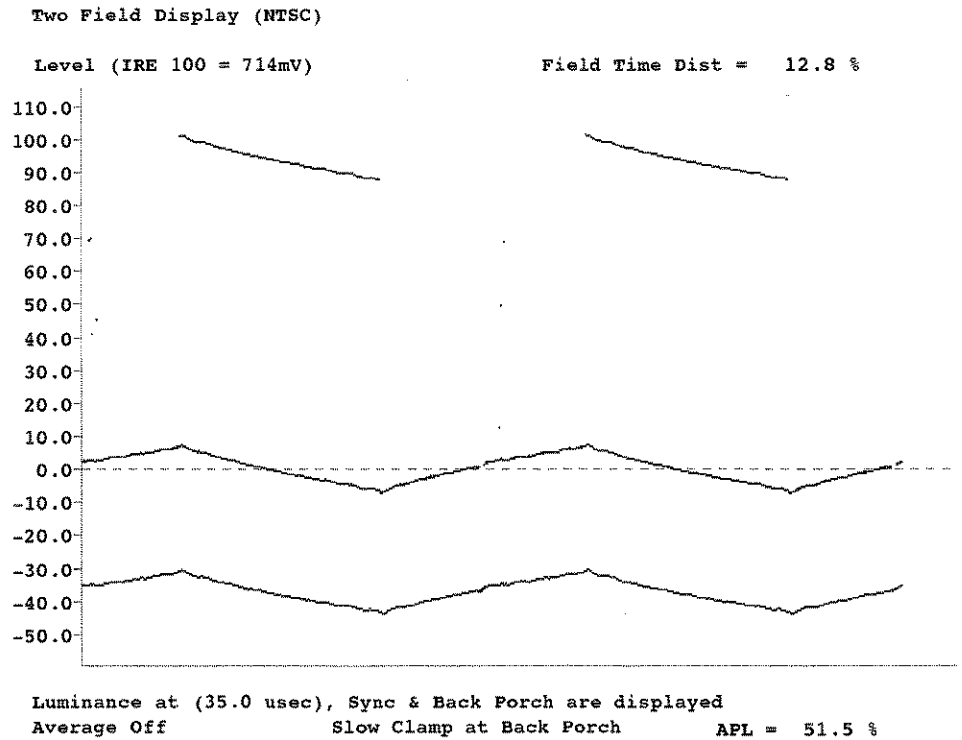
Figure 2-73: TwoField display
