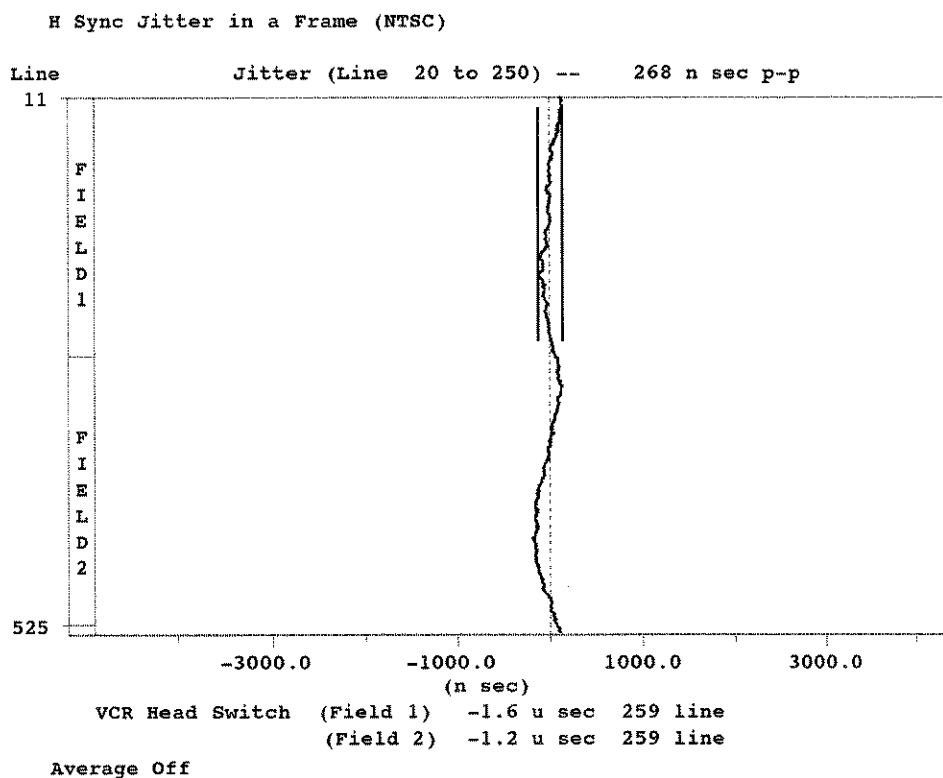
Figure 2-36: Jitter display
