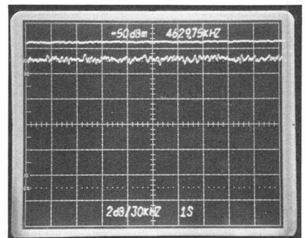
Figure 5. Noise and equal display cw signal in logarithmic display mode.
