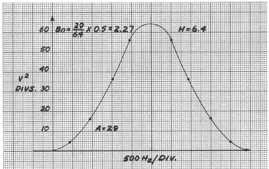
Figure 2. Power (voltage squared) resolution bandwidth response.
