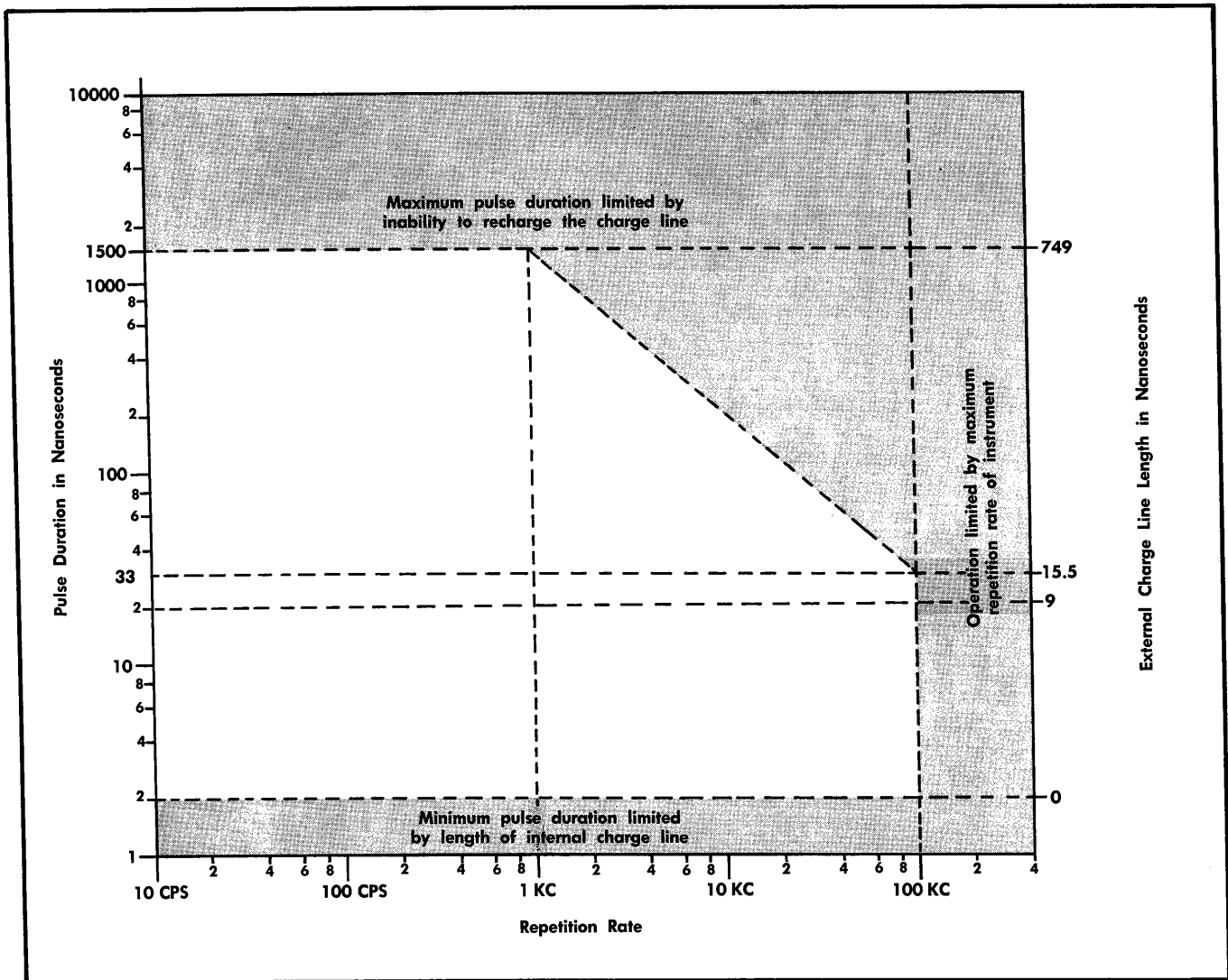
Fig. 2-3. Charge line selection guide (S/N 800-up). * White area represents normal operation. Pulse duration equals 2 nsec plus double-transit time of external charge line.
