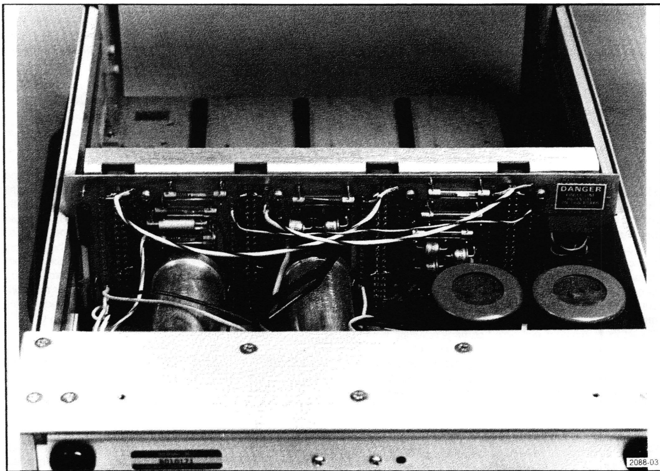
Fig. 2-2. Standard Mainframe soldered interconnections.
