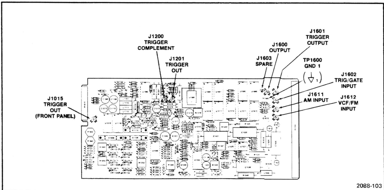
Fig. FG 5010-3. Sine Shaper board.
