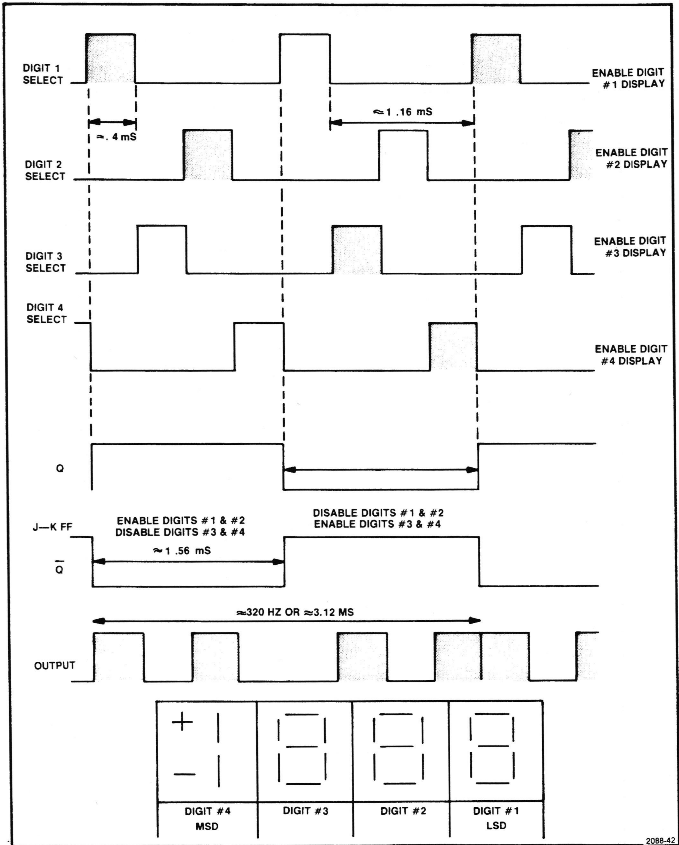
Fig. DM 502-6. Digit select waveforms.
