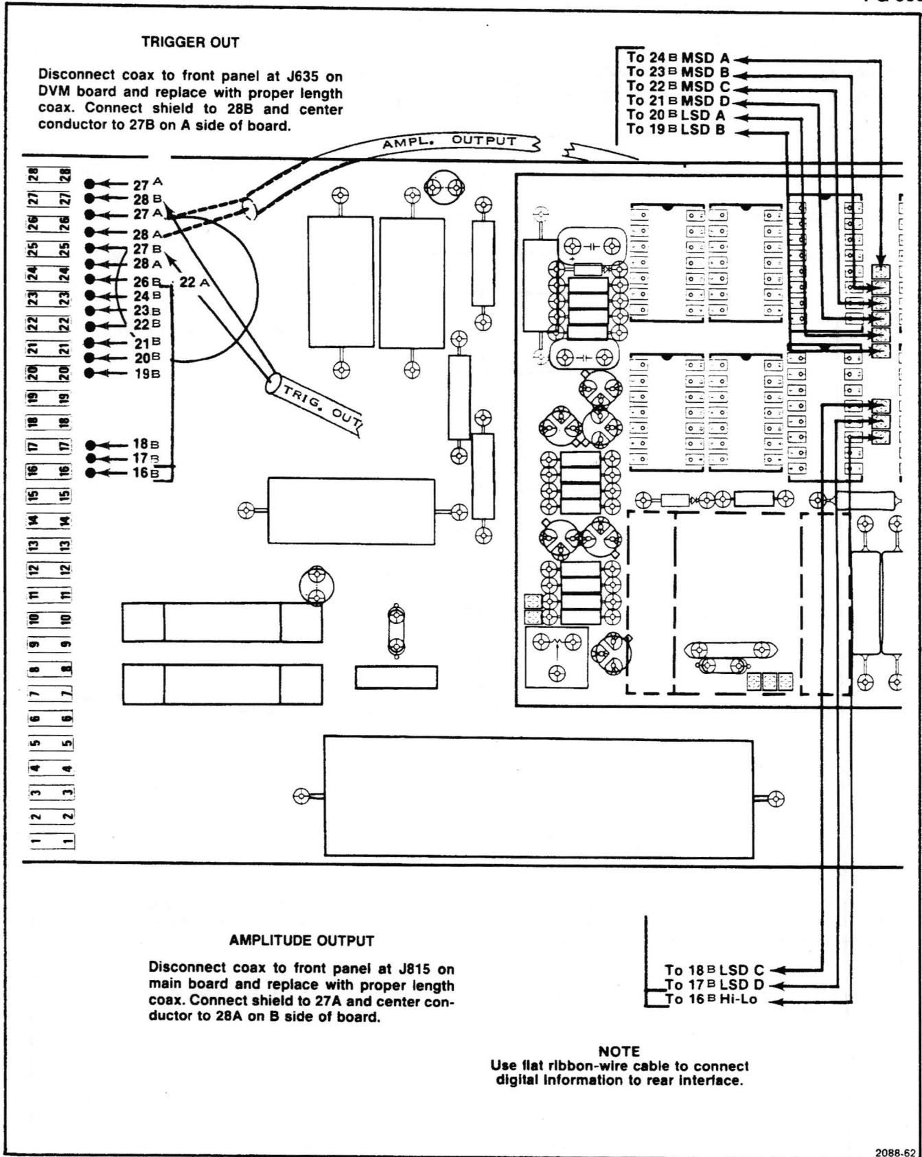
Fig. PG 506-2. Interface connection locations.
