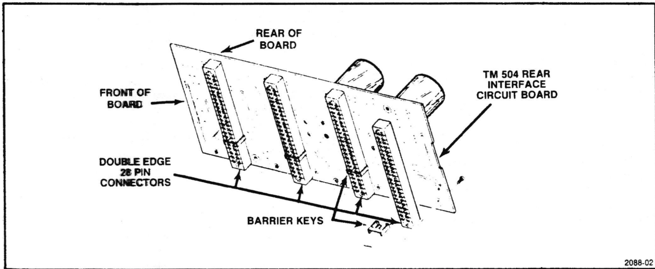
Fig. 2-1. Barrier Keys.
