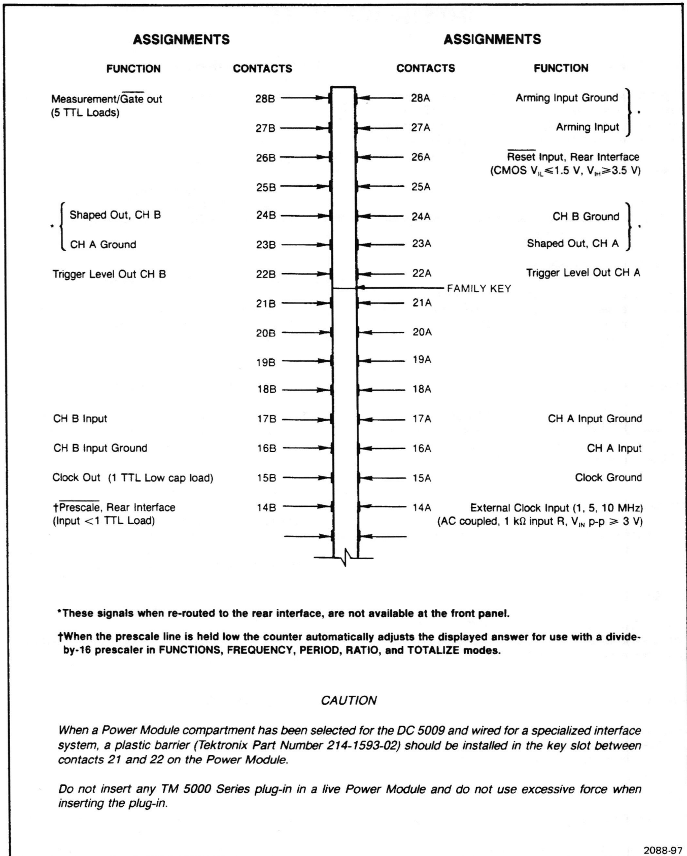
Fig. DC 5009-1. Connector rear view.
