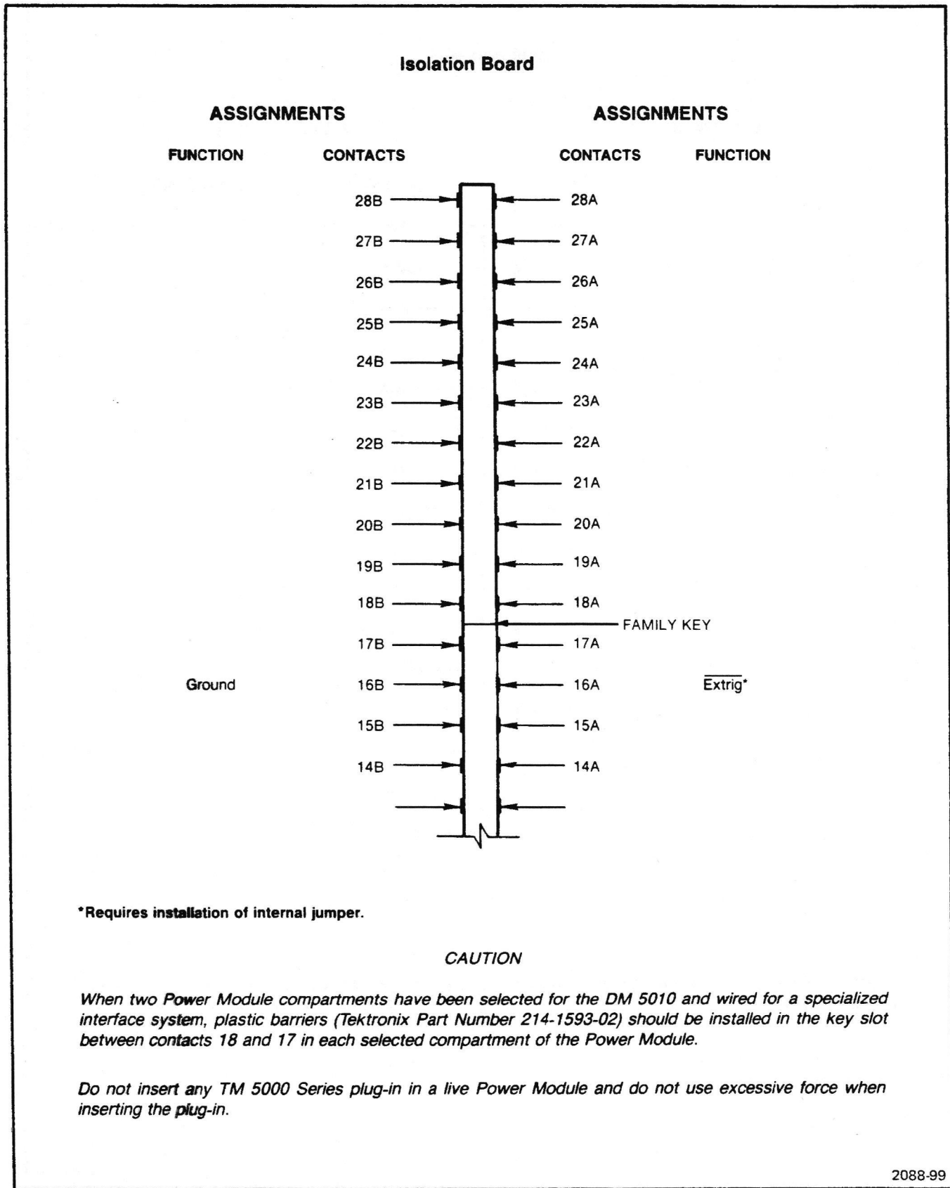
Fig. DM 5010-2. Middle rear (Isolation Board) interface connector rear view.
