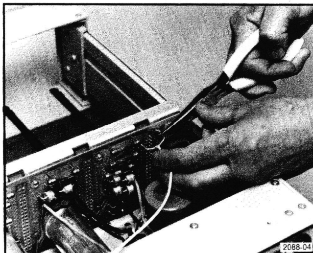
Fig. 2-3. Option 02 Mainframe Interconnections.
