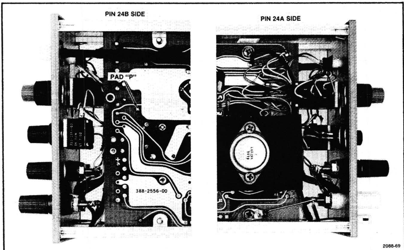
Fig. PS 501-3. Unsolder lead to pad "p" to open sense lead from J50.
