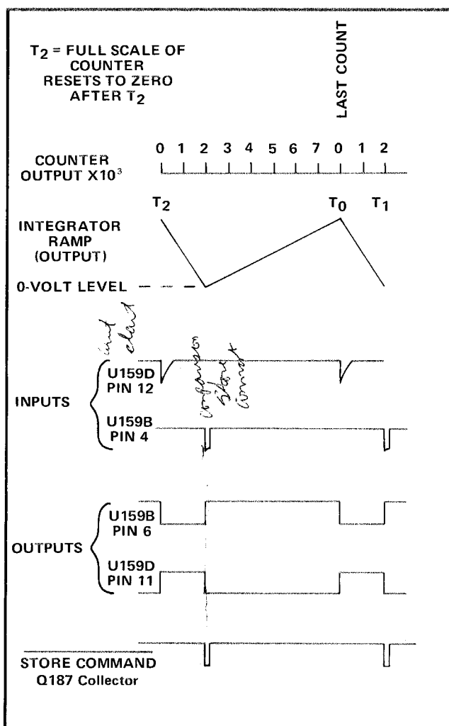
Fig. 3-2. Analog-to-Pulse-Width Converter circuit waveforms showing their relationship to the Counter output.
