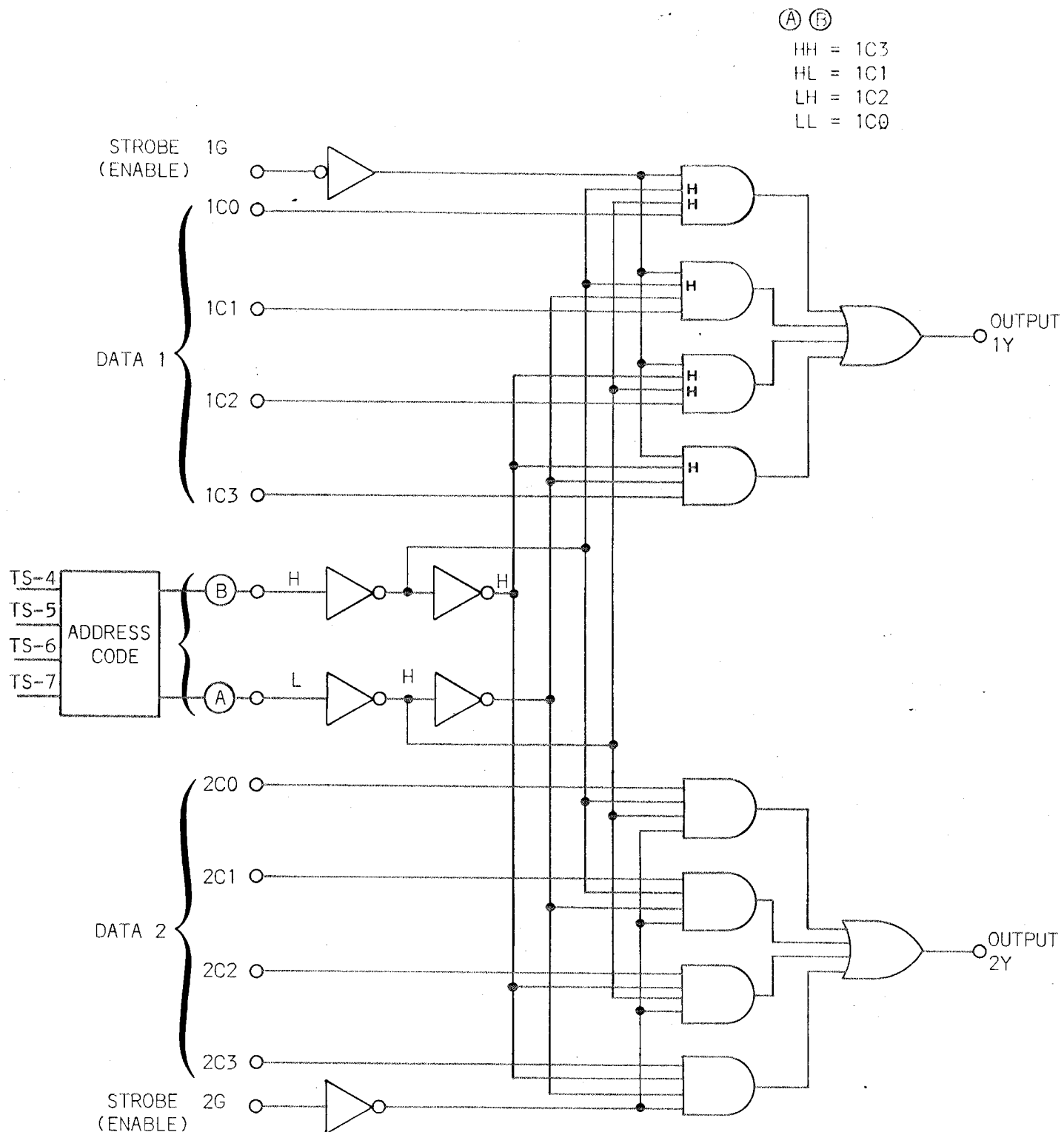
FIGURE 6 - 7D13 FUNCTIONAL BLOCK SN-74153
