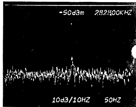
Fig. 6. Three tone intermodulation product at 2828 kHz.
