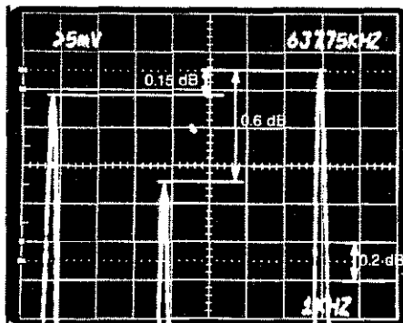
Fig. 8. Expanded amplitude measurement of three channel carriers at 0.2 dB/div.
