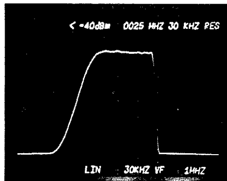
Fig. 6. A "textbook" Nyquist slope response is achieved by the SAW filters used in the 1450.
