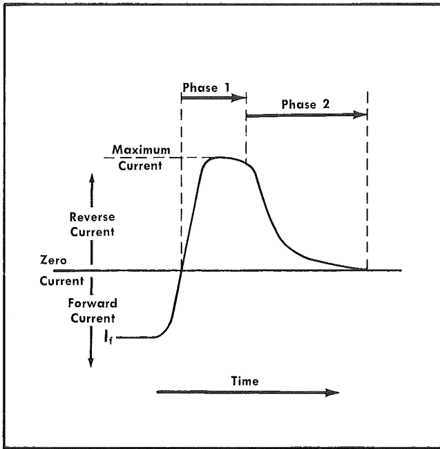
Fig. 2-6. Diode reverse recovery current.
