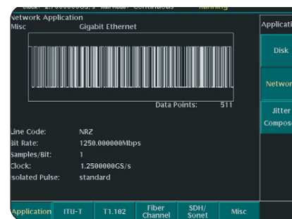
▶ Gigabit Ethernet Application Menu.
