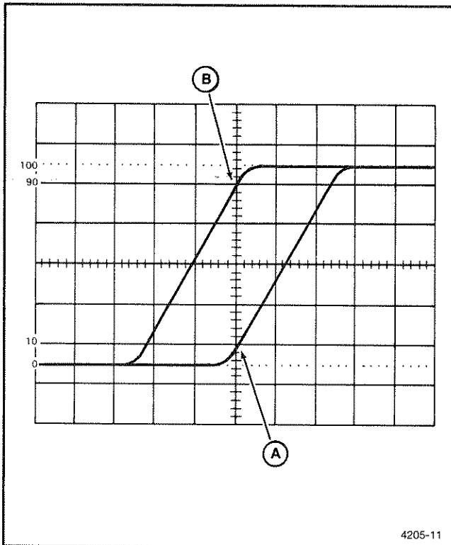
Figure 2-18. Rise time.
