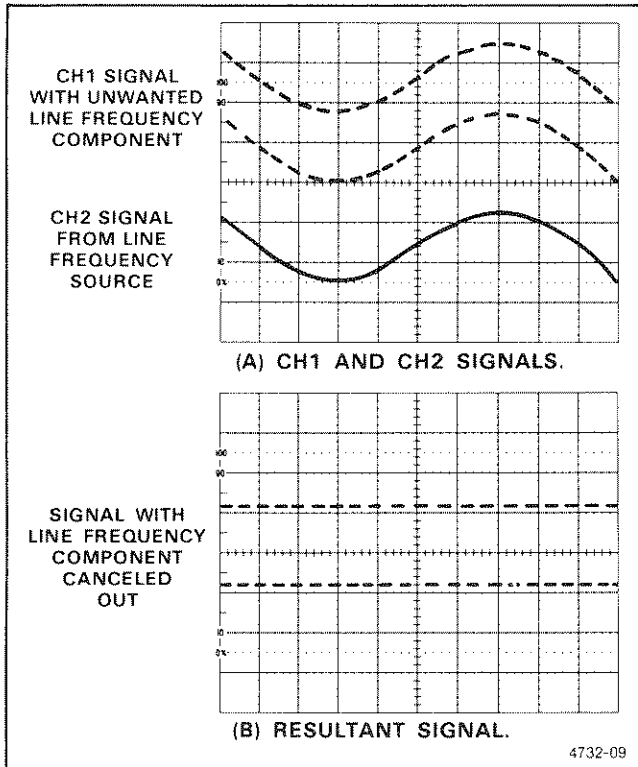
Figure 2-14. Common-mode rejection.
