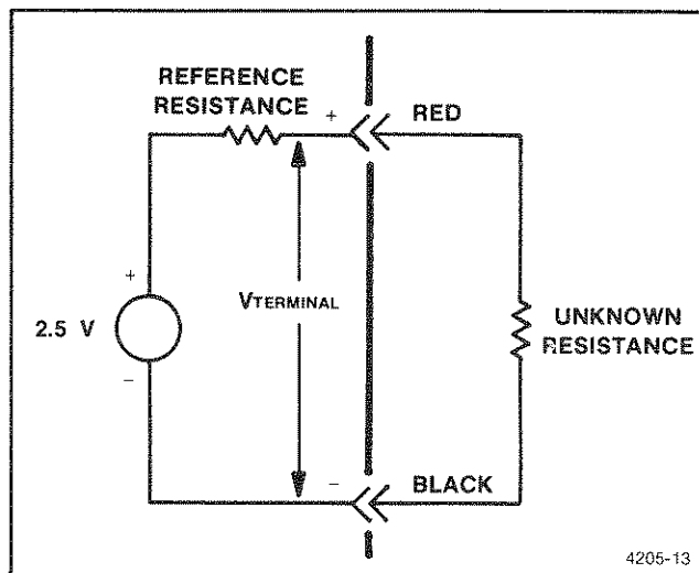
Figure 2-20. Resistance measurement technique.
