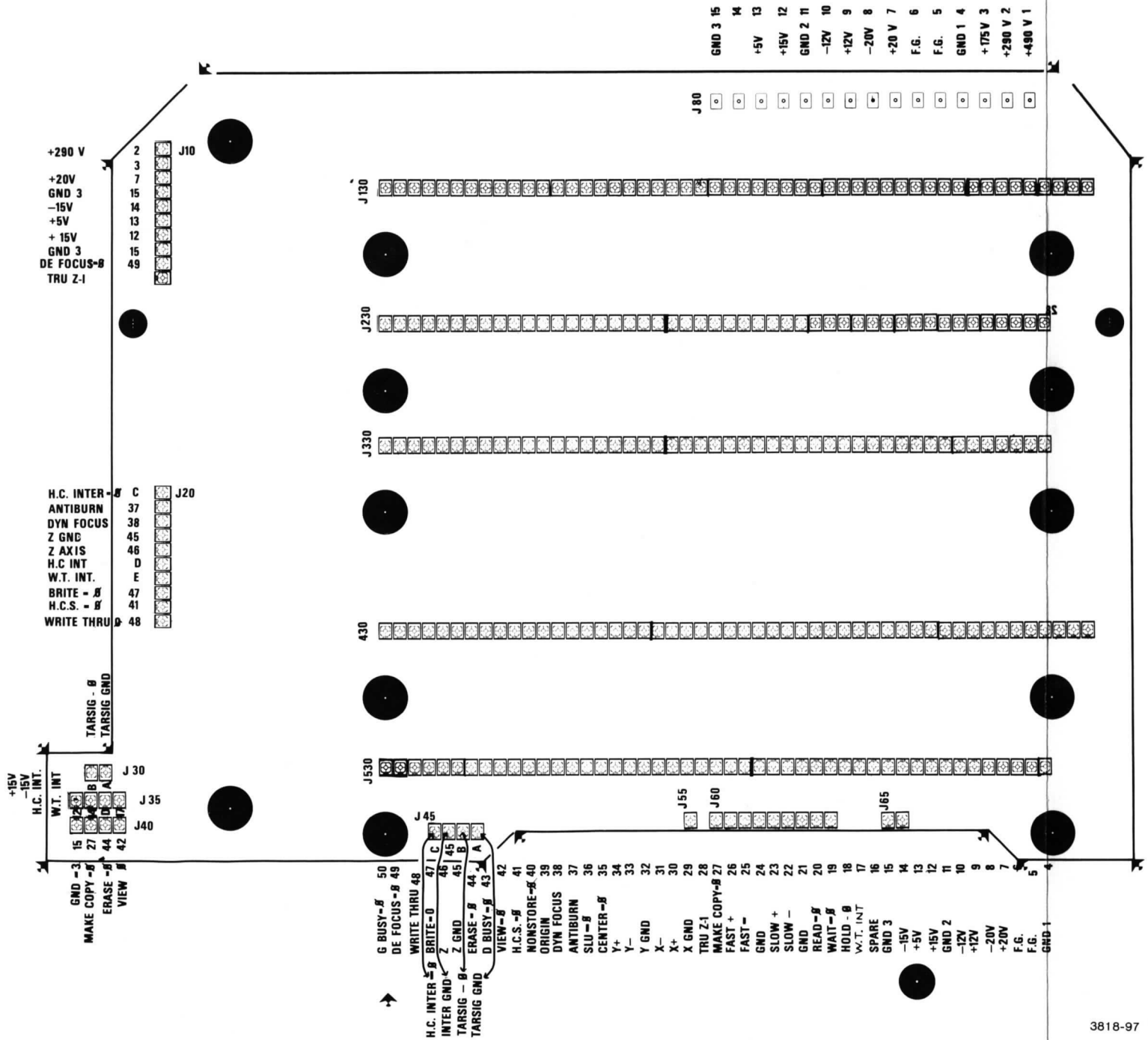
Interconnect (670-5163-01) Component Locations.
