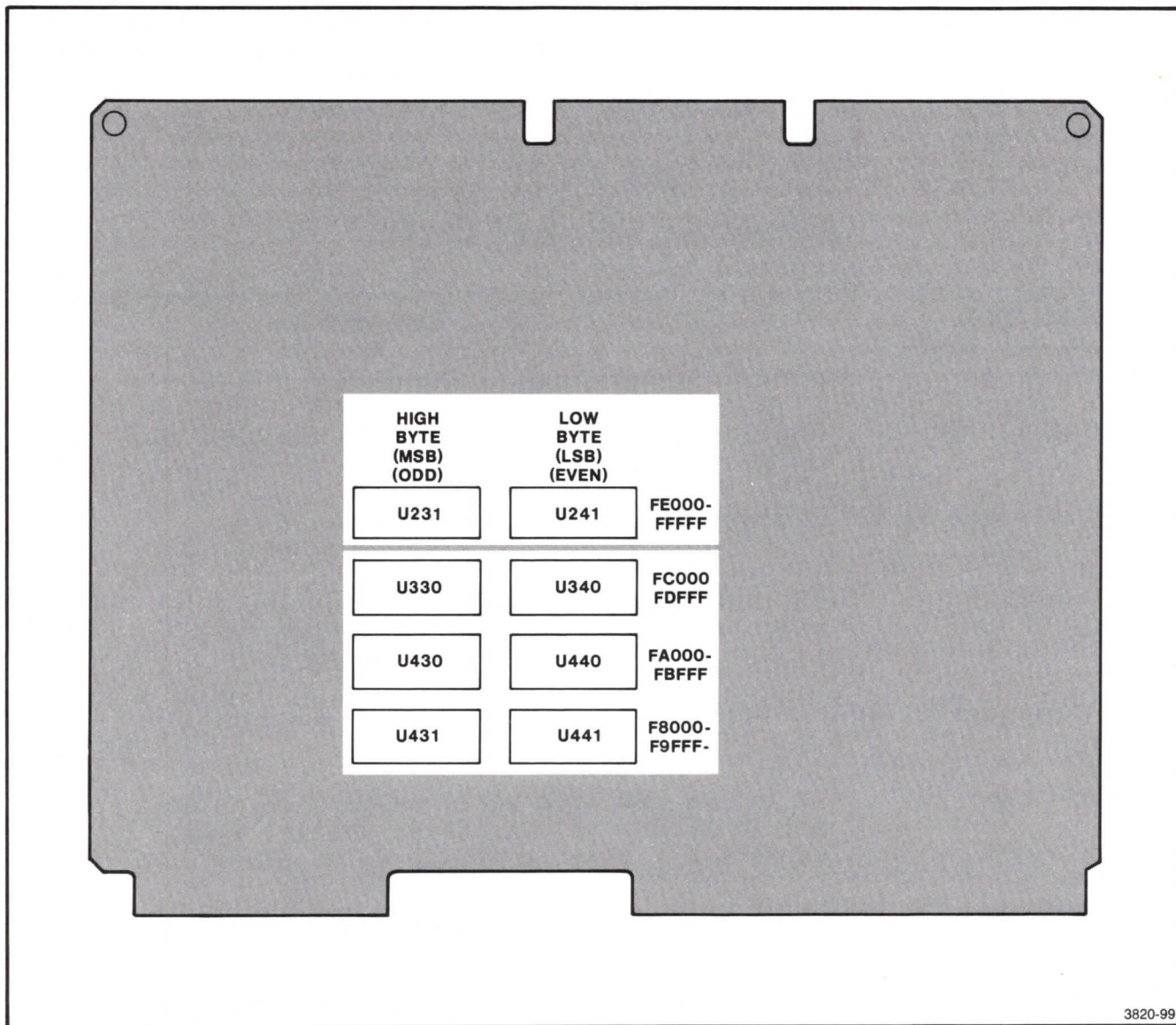
Figure 5-5. Processor Board ROMs.
