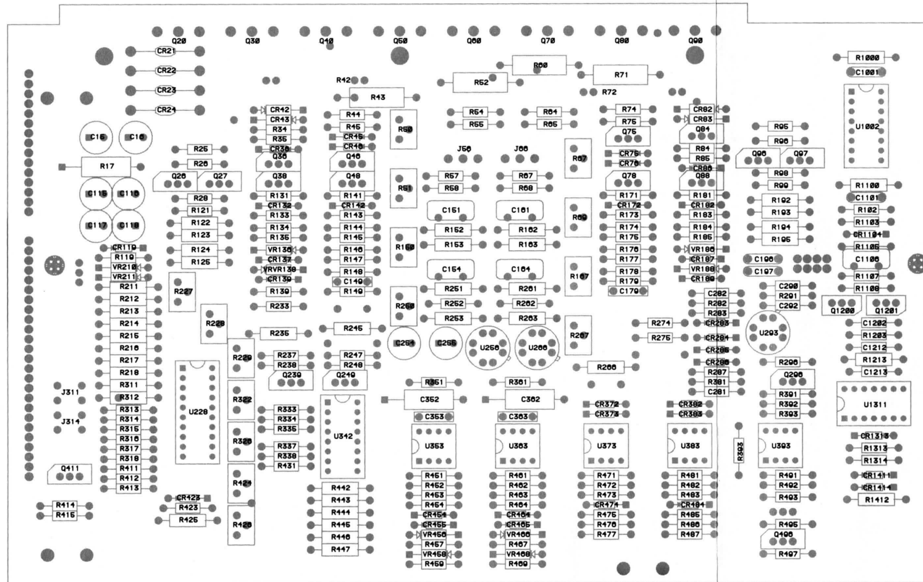
Deflection Amplifier (672-0901-01) Component Locations.
