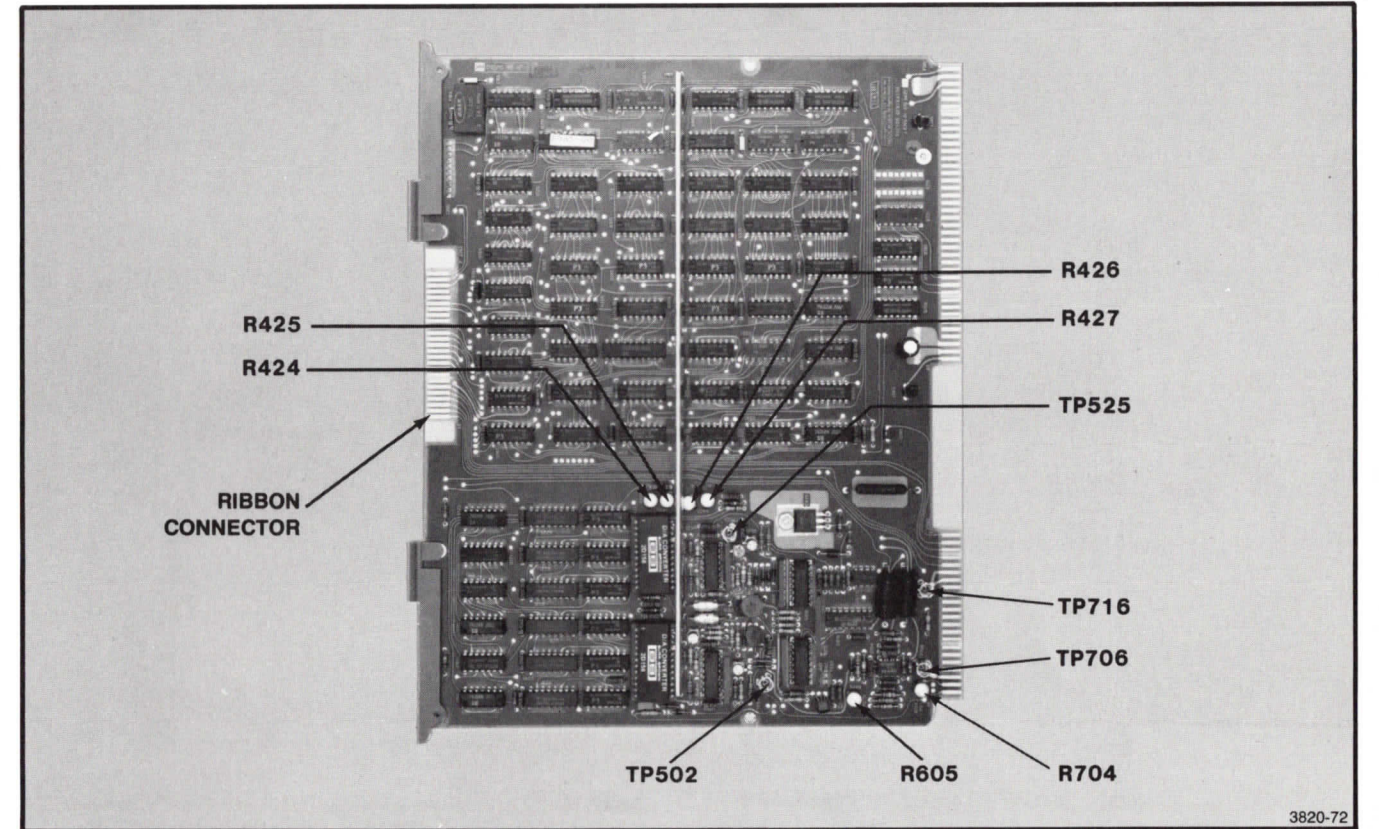
Figure 4-17. Vector Generator Board-A9.
