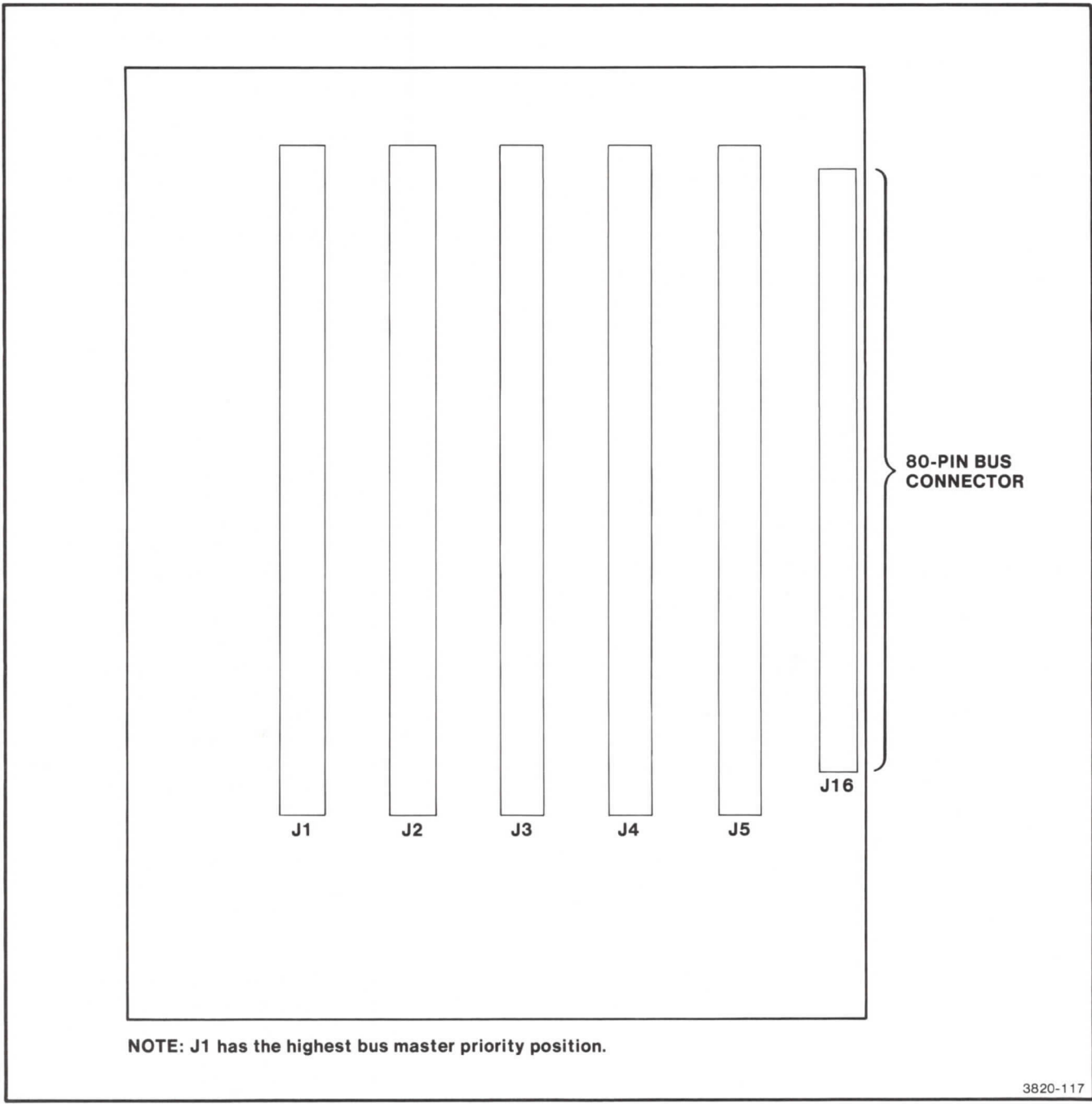
Figure 1-2. 4114 Motherboard.
