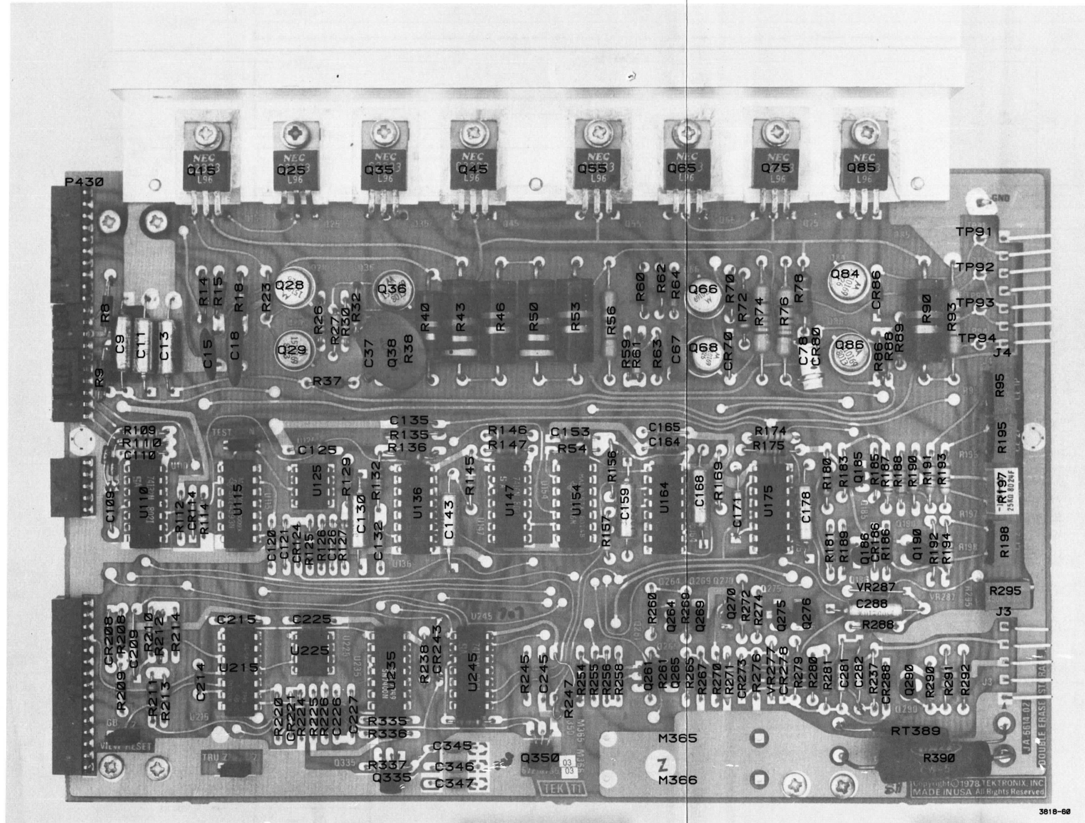
Double Erase Storage (672-0795-03,04) Component Locations.
