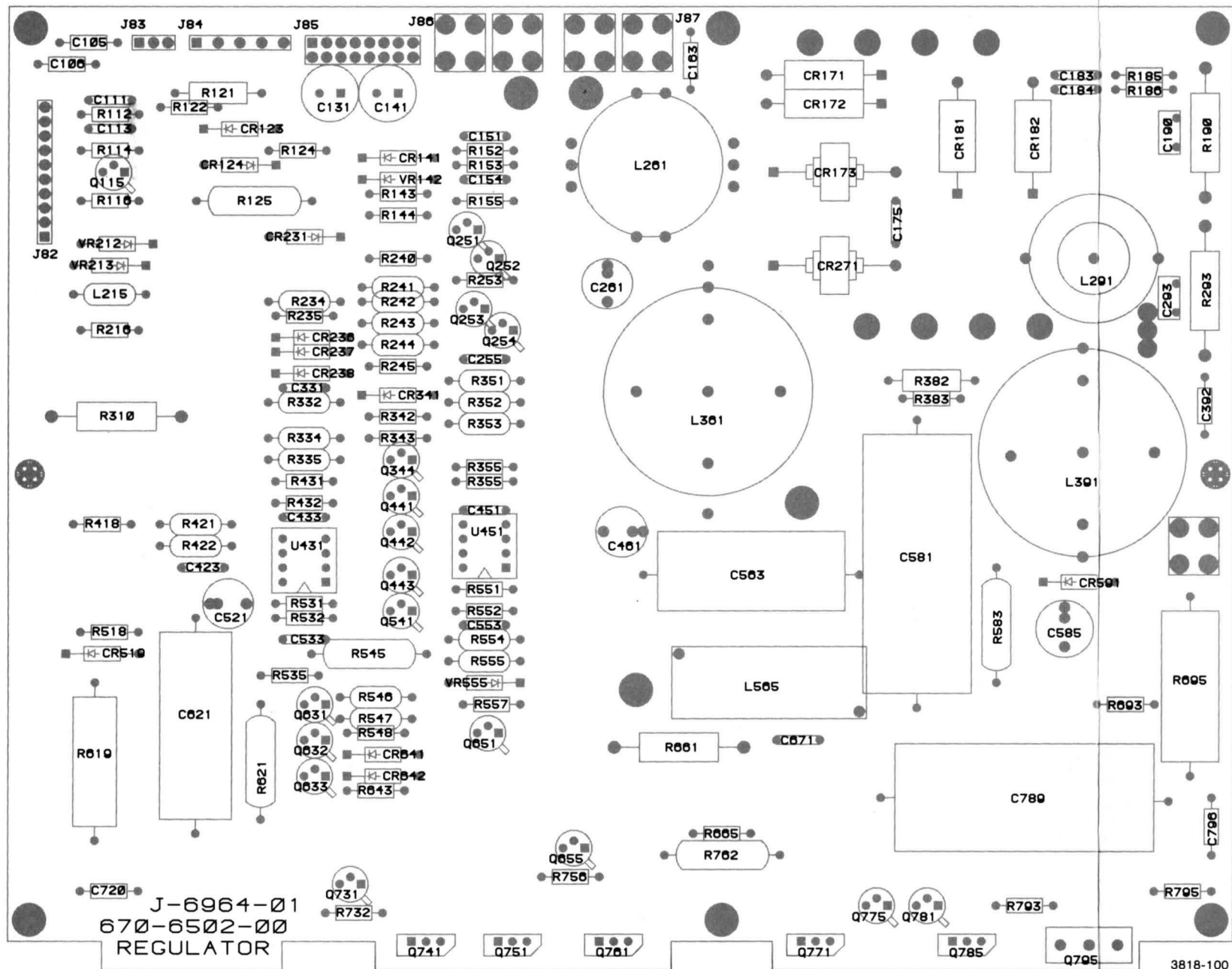
Regulator (670-6502-00,01) Component Locations.
