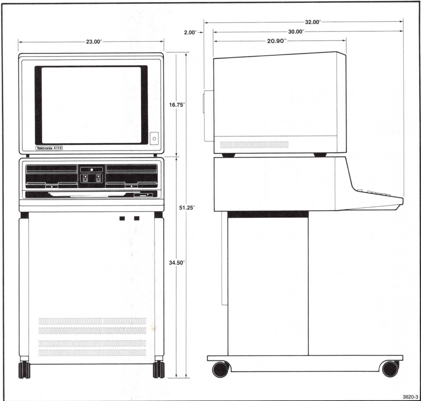
Figure 2-1. 4114 Dimensions.
