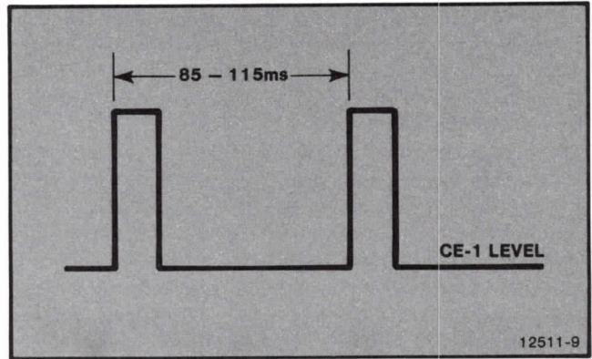
Figure 4-10. CE-1 Waveform.
