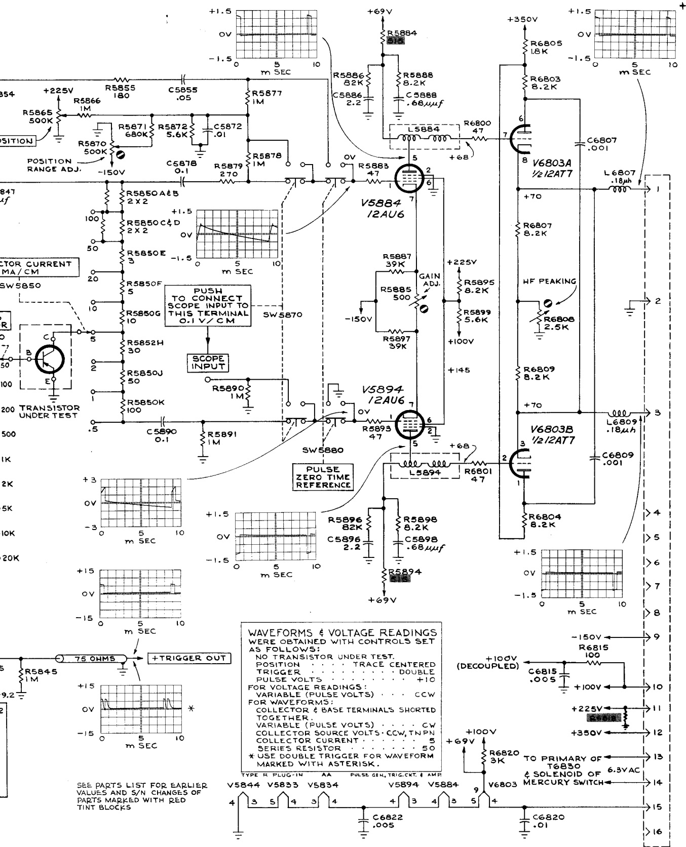
PULSE GENERATOR, TRIGGERING CIRCUIT, & AMPLIFIER
