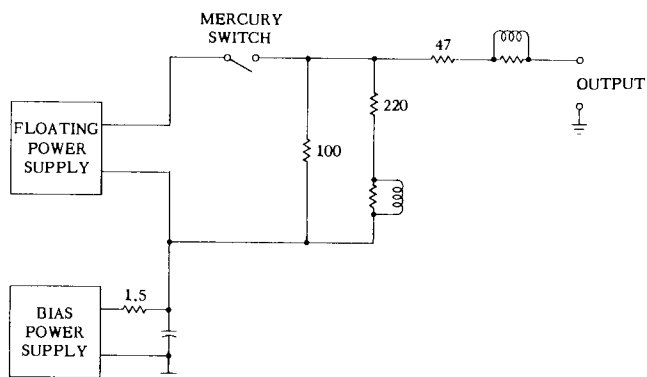
Fig. 3-1. Simplified diagram of the Pulse Generator.
