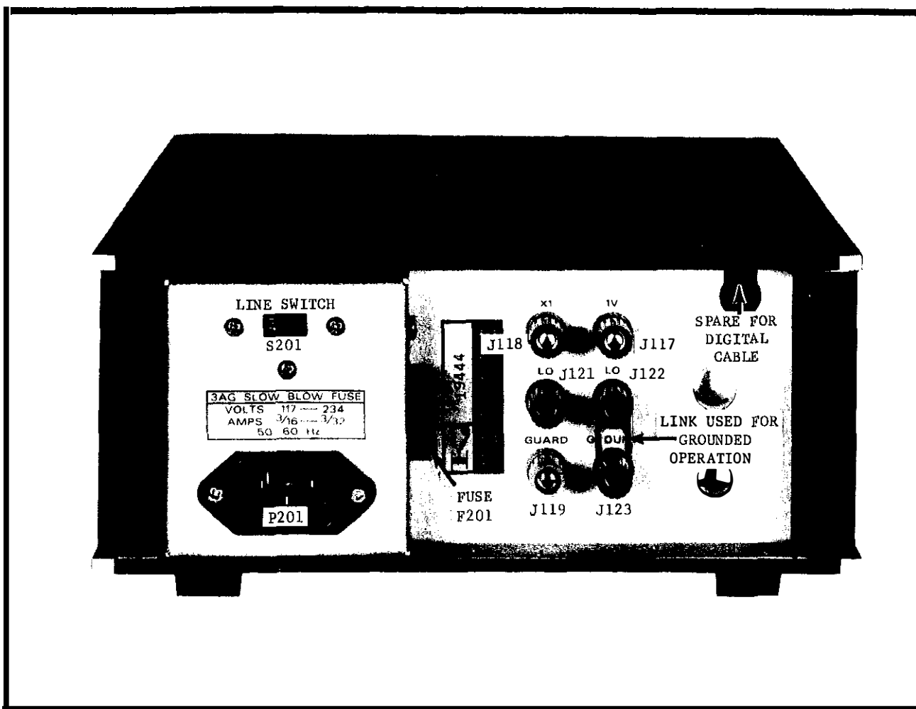
FIGURE 3. Rear Panel Connectors.
