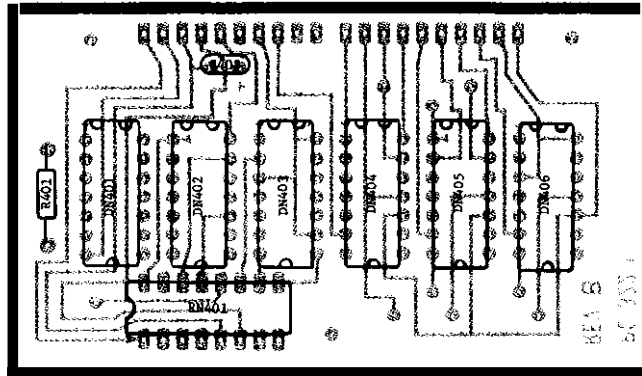
FIGURE 36. Component Layout, PC-322.
