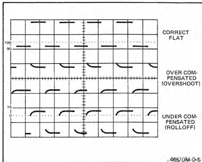
Figure 10. Probe compensation.
