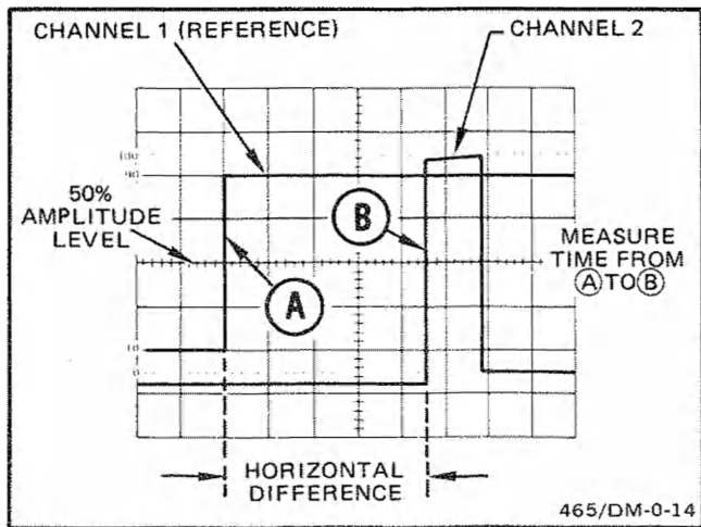
Figure 18. Time difference between two time-related pulses.
