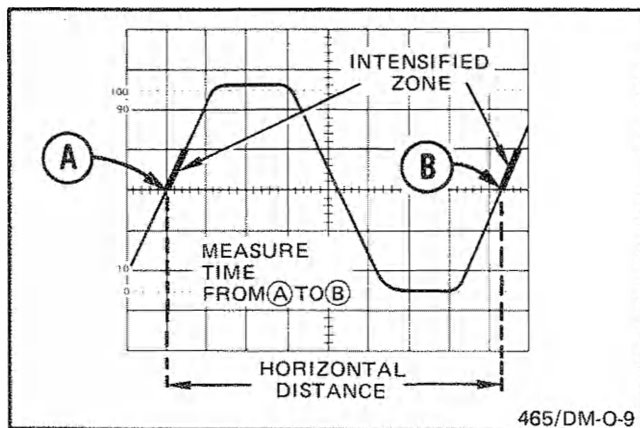
Figure 23. Time duration using delayed sweep.
