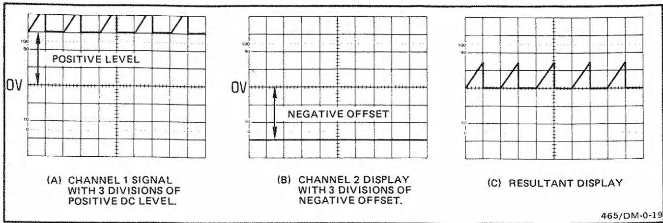
Figure 14. Algebraic addition.
