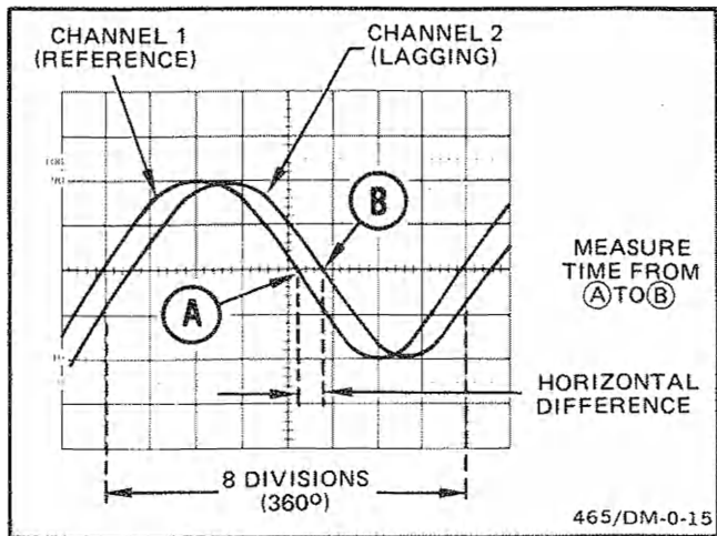
Figure 19. Phase difference.
