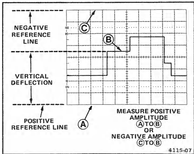
Figure 13. Instantaneous voltage measurement.
