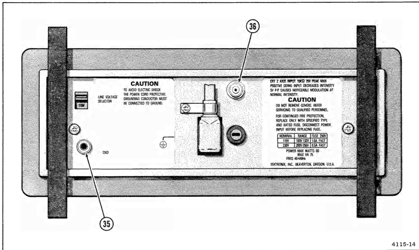
Figure 7. Rear-panel connectors.
