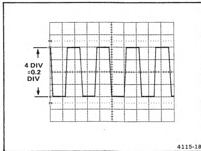
Figure 11. Vertical display accuracy.
