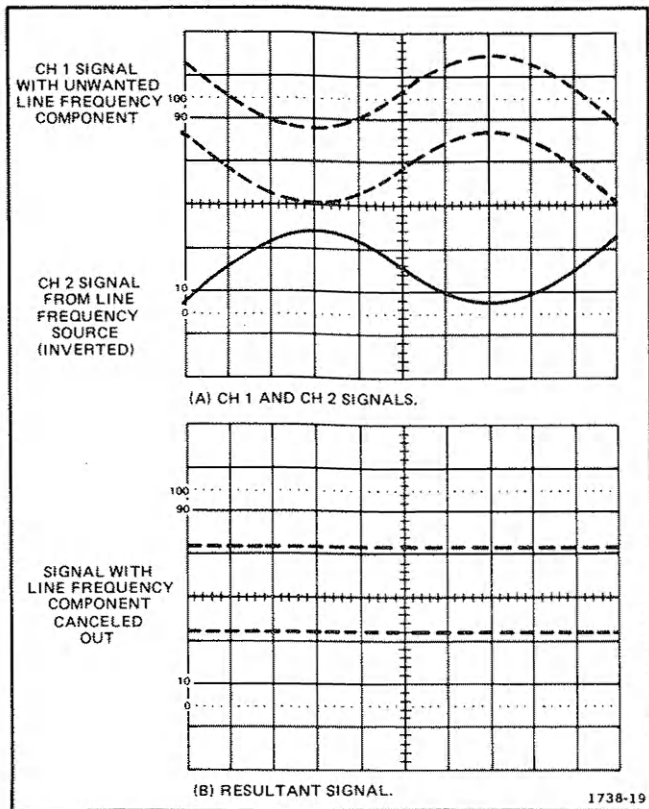
Figure 15. Common-mode rejection.
