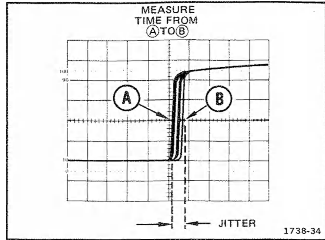
Figure 22. Pulse jitter.
