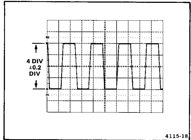
Figure 12. Vertical display accuracy.
