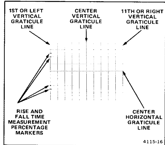
Figure 9. Graticule measurement markings.
