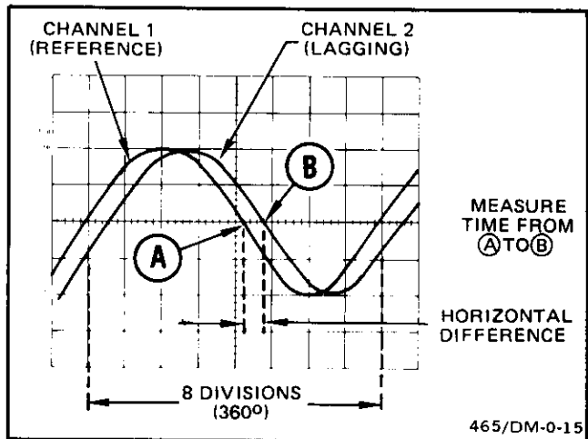
Figure 20. Phase difference.
