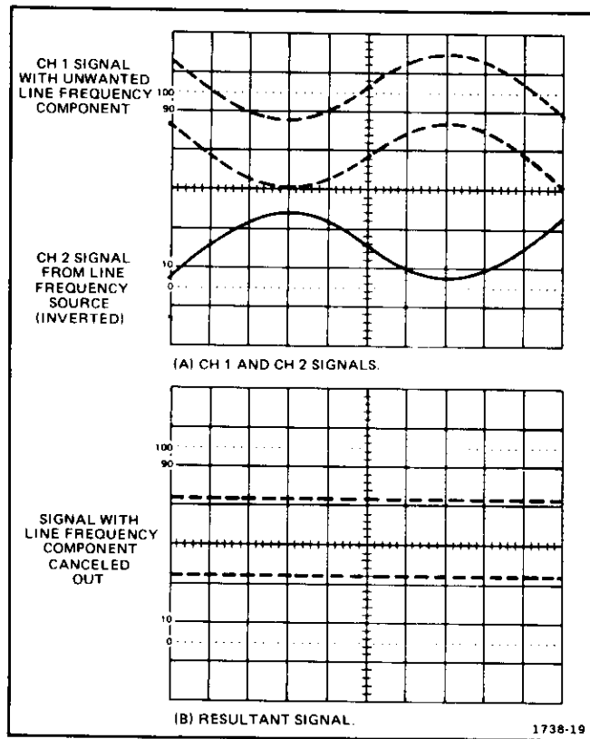
Figure 16. Common-mode rejection.
