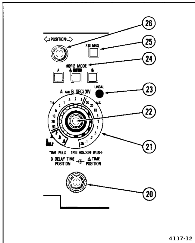
Figure 5. Horizontal controls and indicator.
