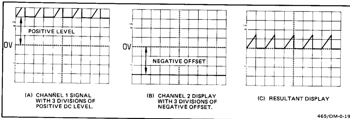
Figure 15. Algebraic addition.
