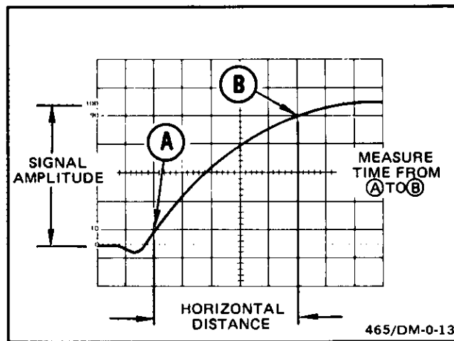
Figure 18. Rise time.
