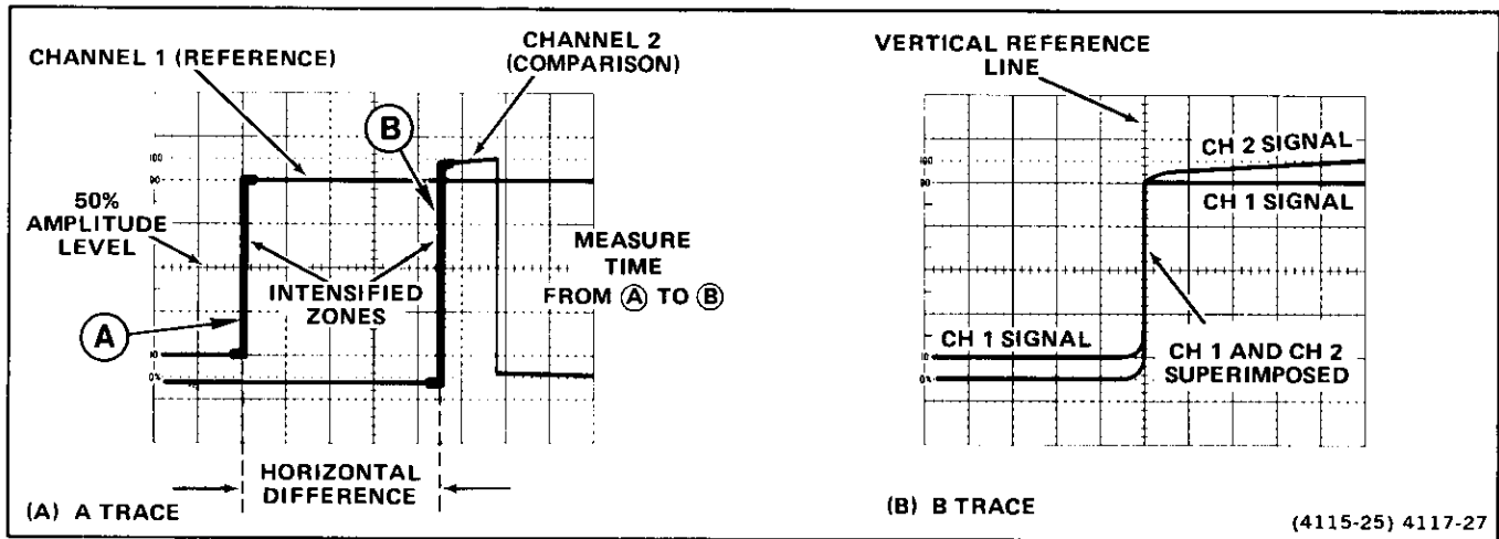
Figure 27. Time difference between two time-related pulses.
