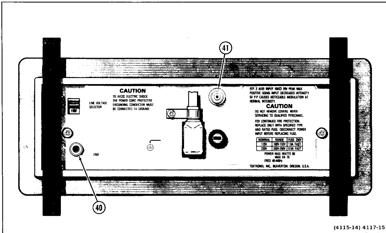
Figure 8. Rear-panel connectors.
