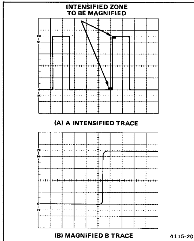
Figure 22. Delayed-sweep magnification.
