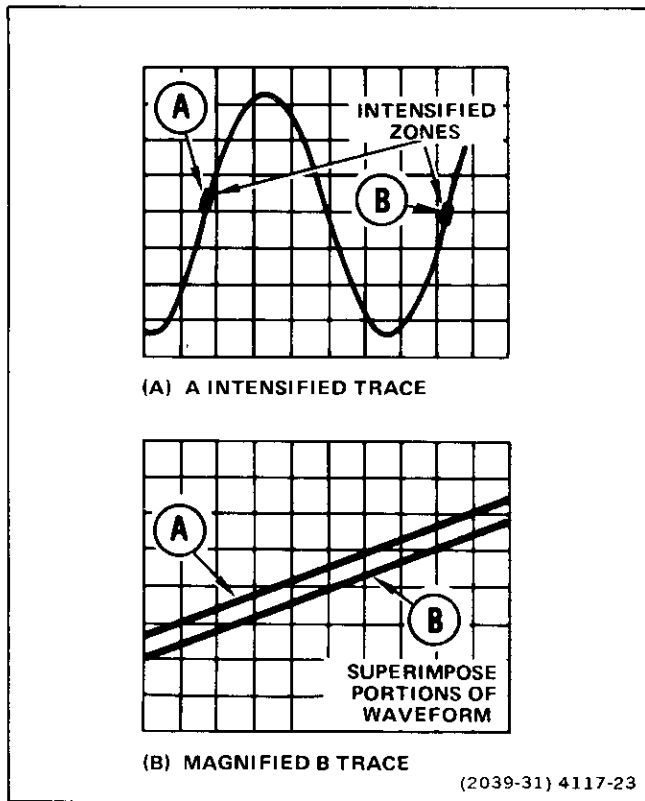
Figure 24. Time duration using delayed sweep.
