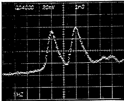
The unparalleled capability of the 7D14 is dramatically illustrated in this photo showing counting of a high-speed pulse train at 100 MHz. In fact, it's difficult, if not impossible, to measure such a signal with most counters.
