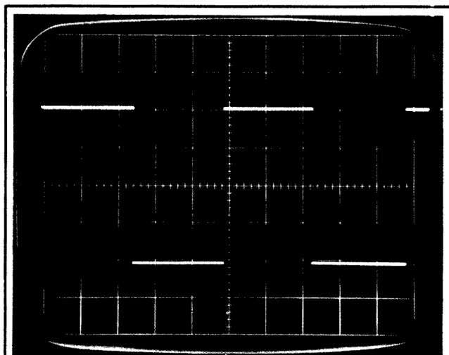
a. DISPLAY FOR CHECKING SHORT TIME CONSTANT SPIKE OR ROLLOFF.
