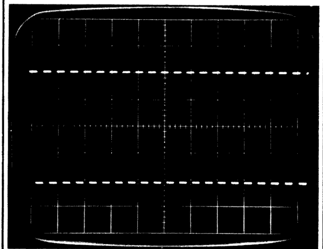
b. DISPLAY FOR CHECKING LONGER TIME CONSTANT TILT OR ROUNDING.
