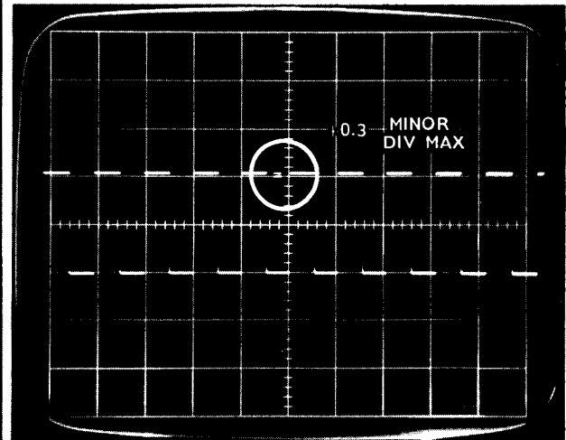
b. DEFLECTION ACCURACY \pm 3\% ( \pm 0.3 MINOR DIV).
