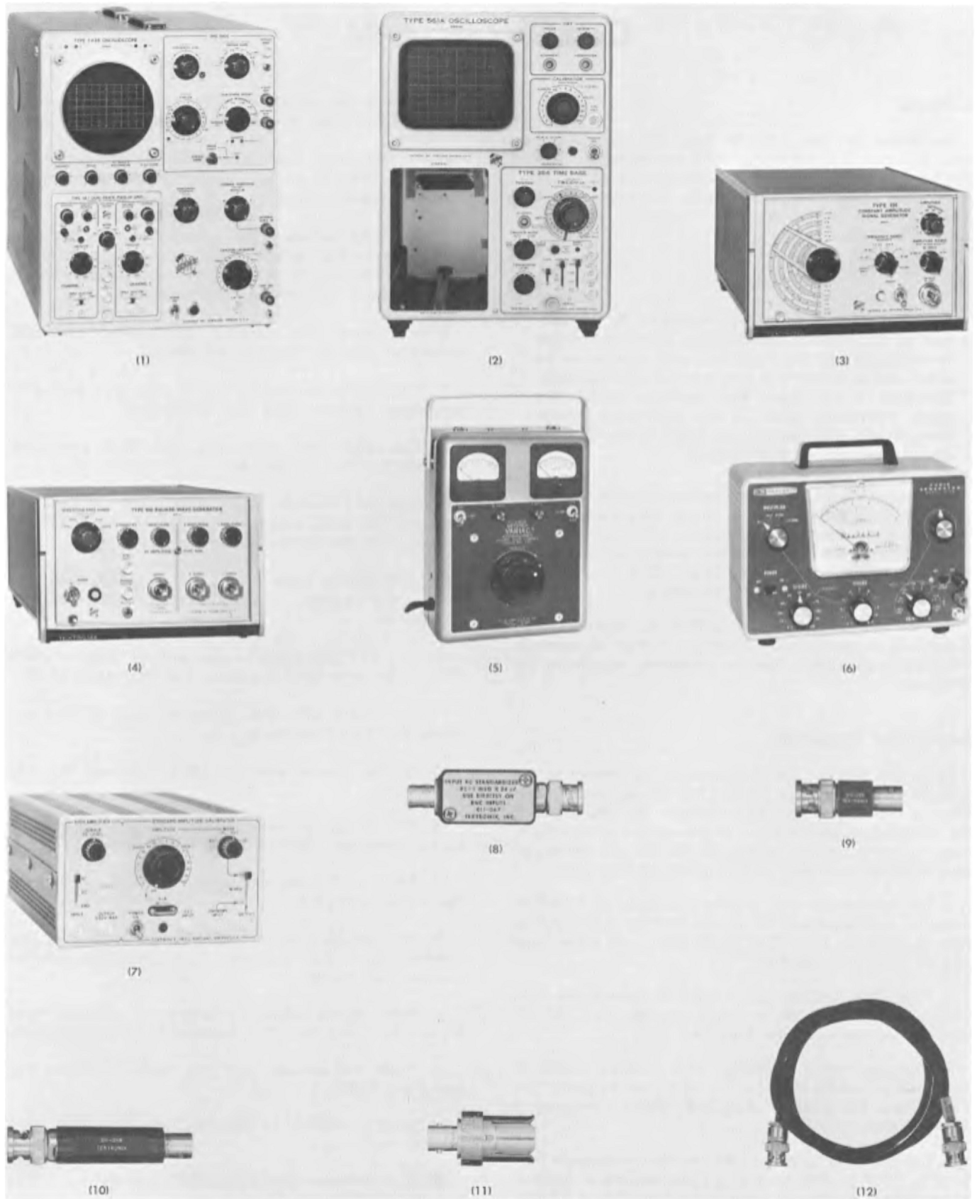
Fig. 6-1. Equipment required for calibration of the Type 3A5.
