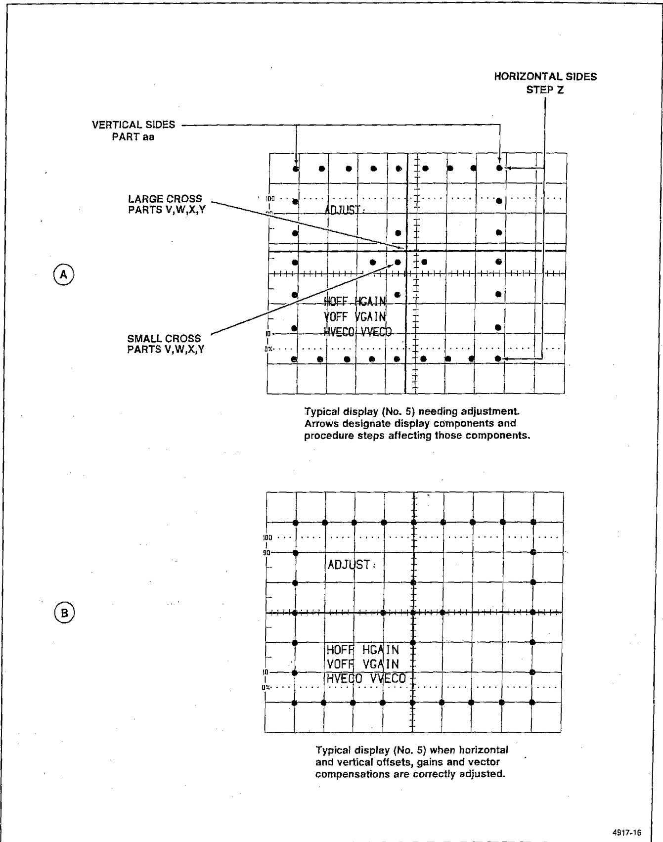
Figure 5-2 (a and b). Display 5—Vertical and Horizontal Gain, Offset, and Vector Compensation adjustments pattern.
