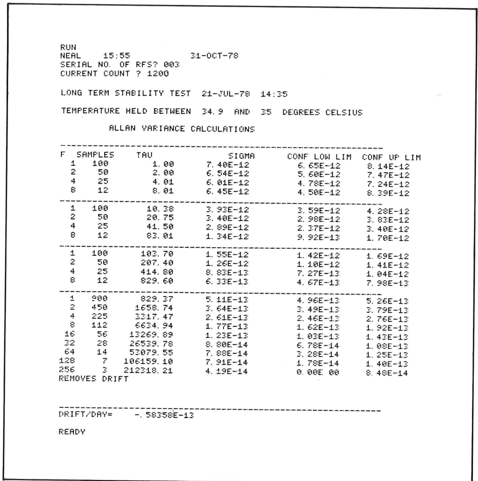
Fig. 7. The Long-Term Frequency Stability test checks the clock frequency stability over time.
