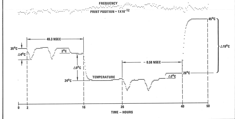
Fig. 9. Clock mounting plate temperature is graphed against the beat periods from the test.
