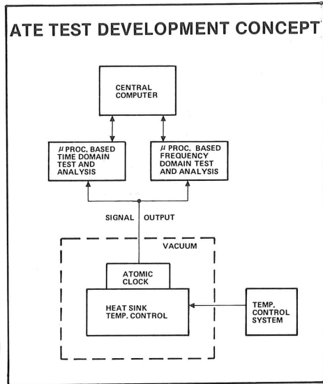
Fig. 4. The automated testing concept.
