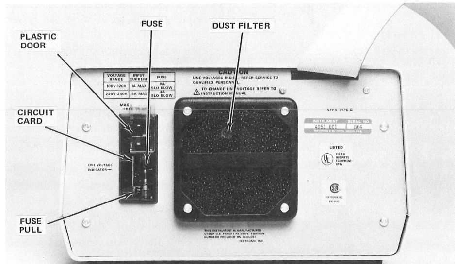
Fig. 2. The dust filter should be kept clean to ensure optimum air flow.
