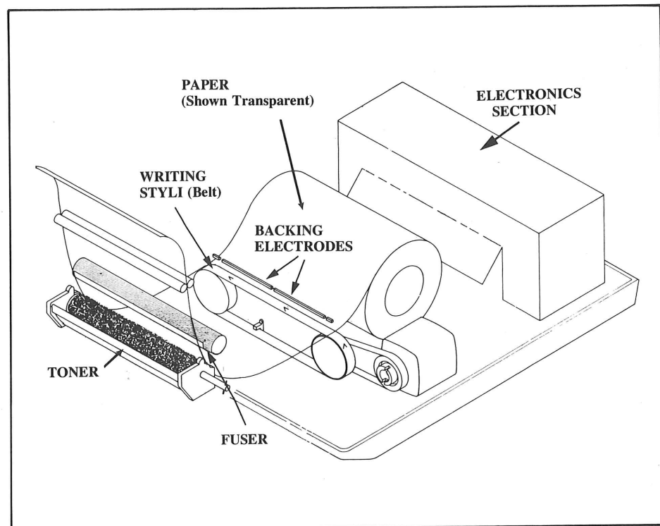
Fig. 2. The TEKTRONIX 4611 Hard Copy Unit - The paper is fed between the backing electrodes and the belt.
