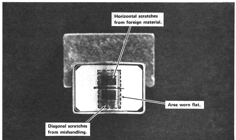
Fig. 4. Tape head damage to look for.
