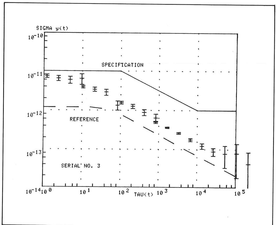
Fig. 8. Frequency vs Varying Temperature is an important test, since the satellite will encounter some predictable temperature excursions.
