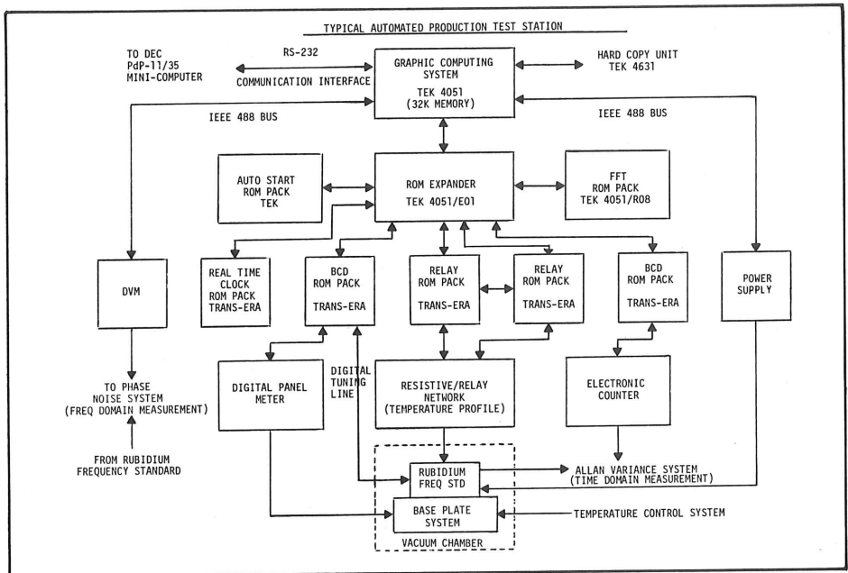
Fig. 5. A typical automated test station is illustrated in this block diagram.
