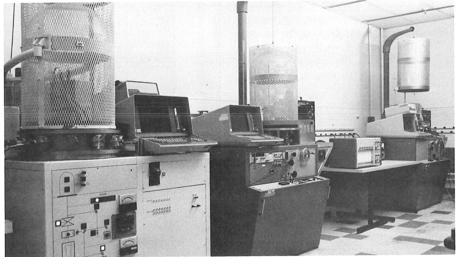
Fig. 3. Three of the four automated test stations. In the two stations on the left, clock assemblies are being tested under the bell jar in a simulated space atmosphere. The right station bell jar is about to be lowered to the base plate on the vacuum stand.
