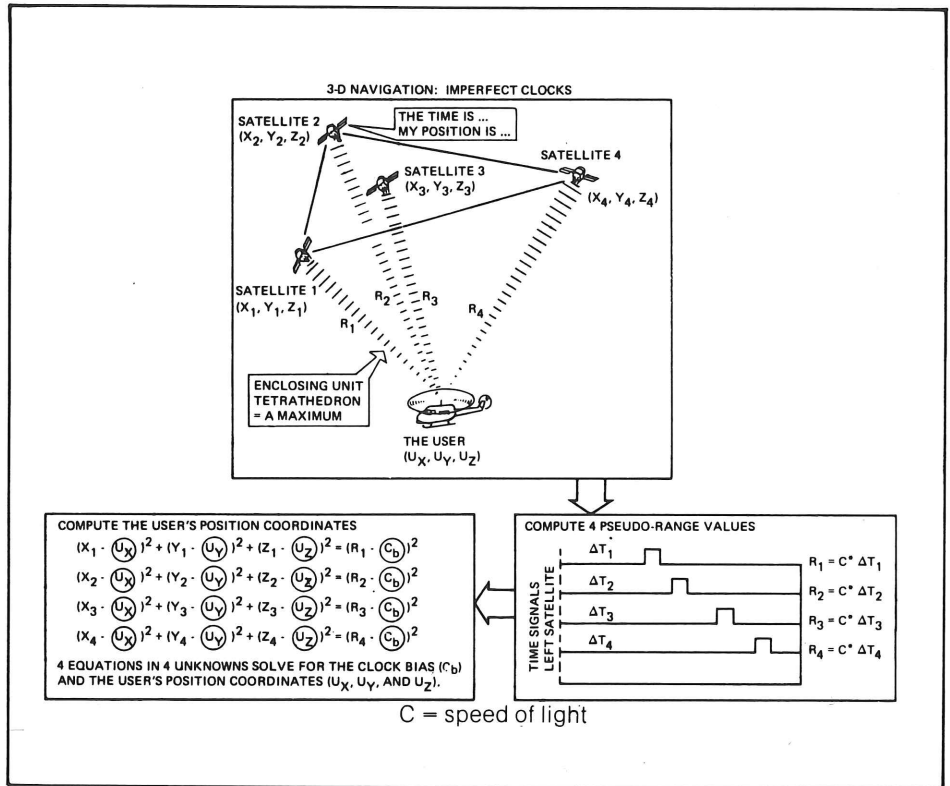
Fig. 1. Three-dimensional navigation is also possible with imperfect user clocks, by locating four satellites and computing the range to each.
