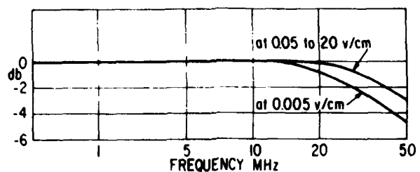
RESPONSE OF TEKTRONIX 544 OSCILLOSCOPE WITH 1A1 PREAMPLIFIER SETTING AS SHOWN FIGURE 6
