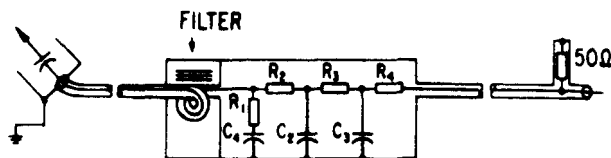
FIGURE 4-WIDE BAND ATTENUATOR
