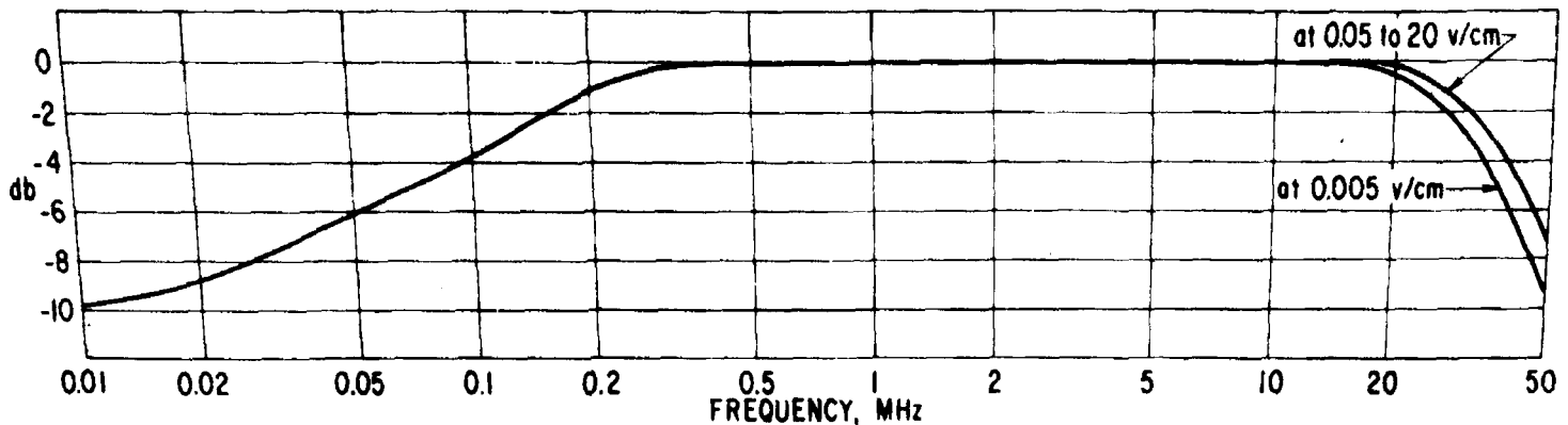
RESPONSE OF COMPLETE SYSTEM- DIFFERENTIATOR, INTEGRATOR, |A| PREAMPLIFIER WITH SETTINGS AS SHOWN, 544 OSCILLOSCOPE FIGURE 7
