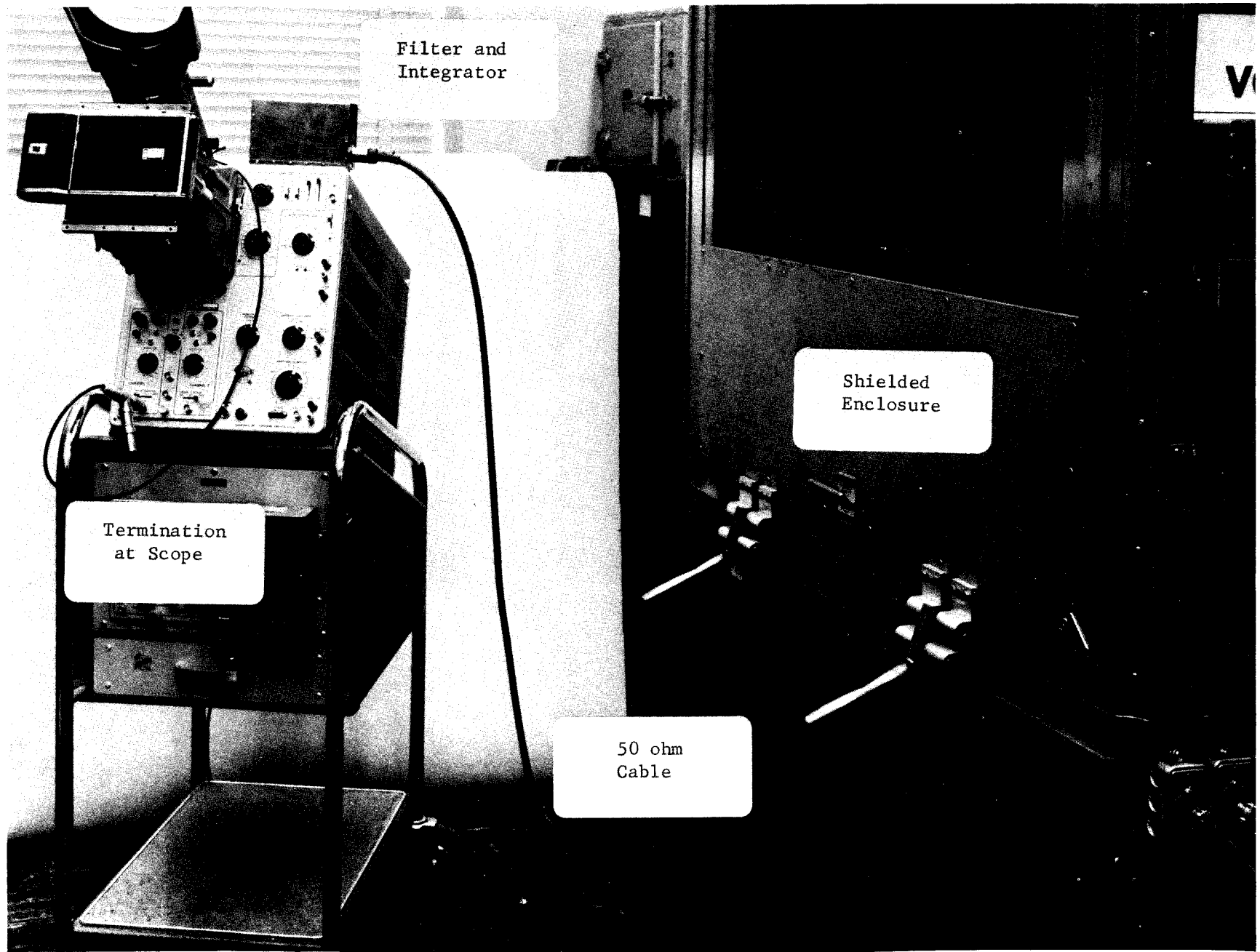
Figure 13 Installation of Mark IV at the R&D Center
