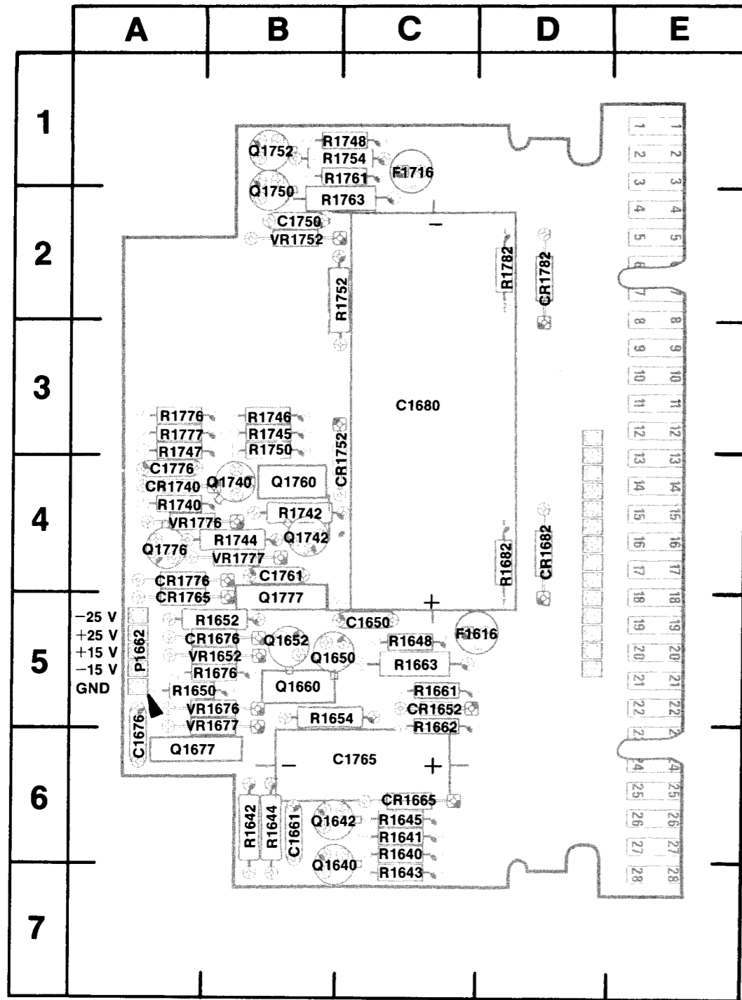
Fig. 8-7. A4 Floating Interface board (front) component locations.
