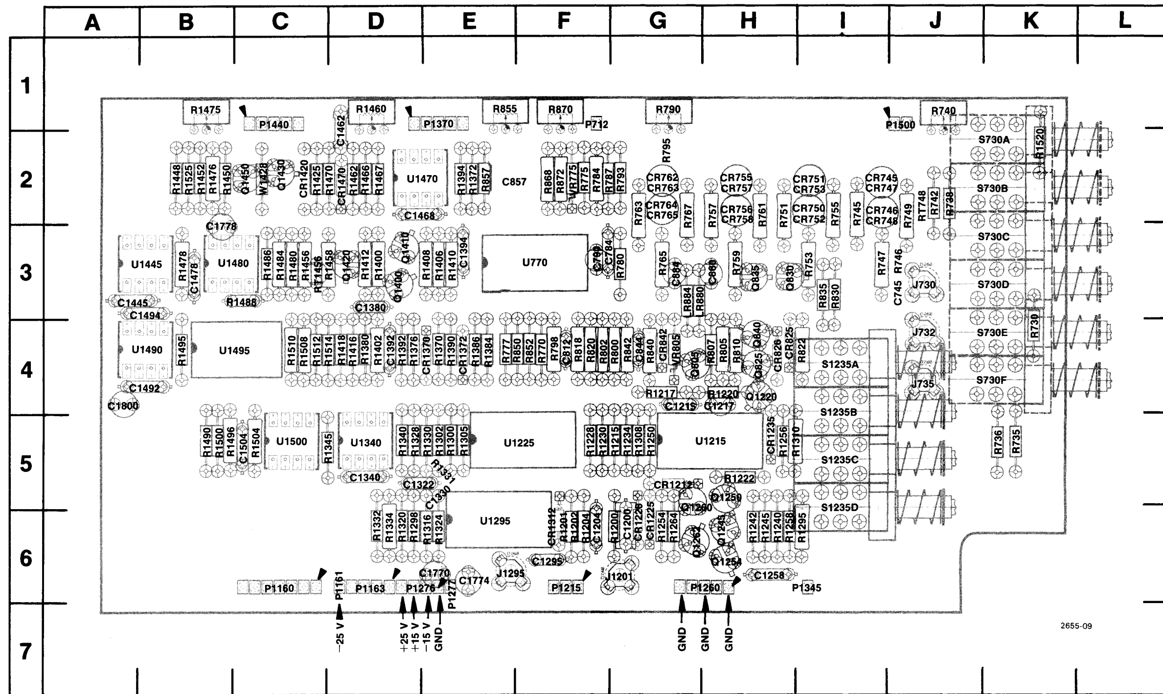
Fig. 8-6. A2 Function board component locations.
