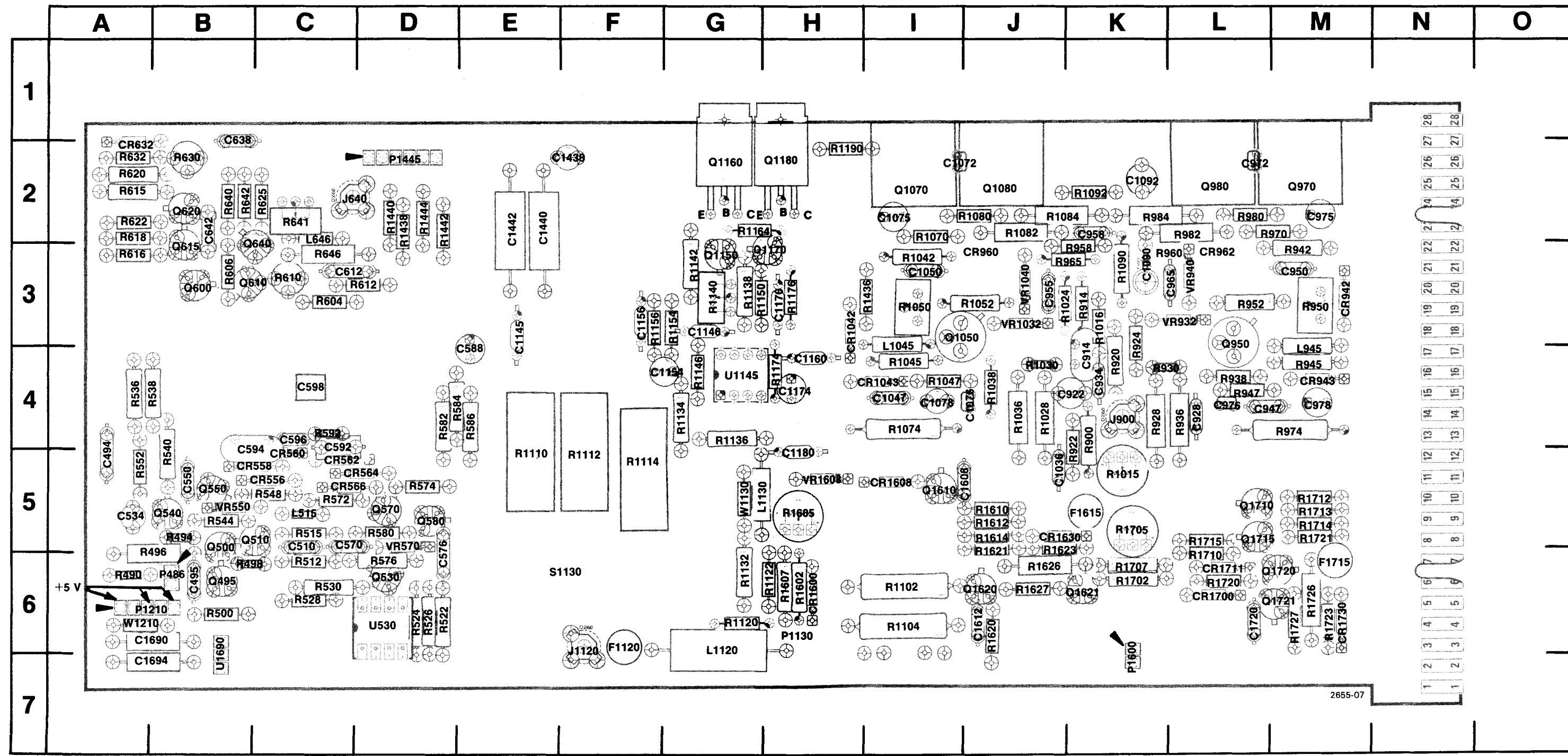
Fig. 8-4. A1 Main board (front) component locations.
