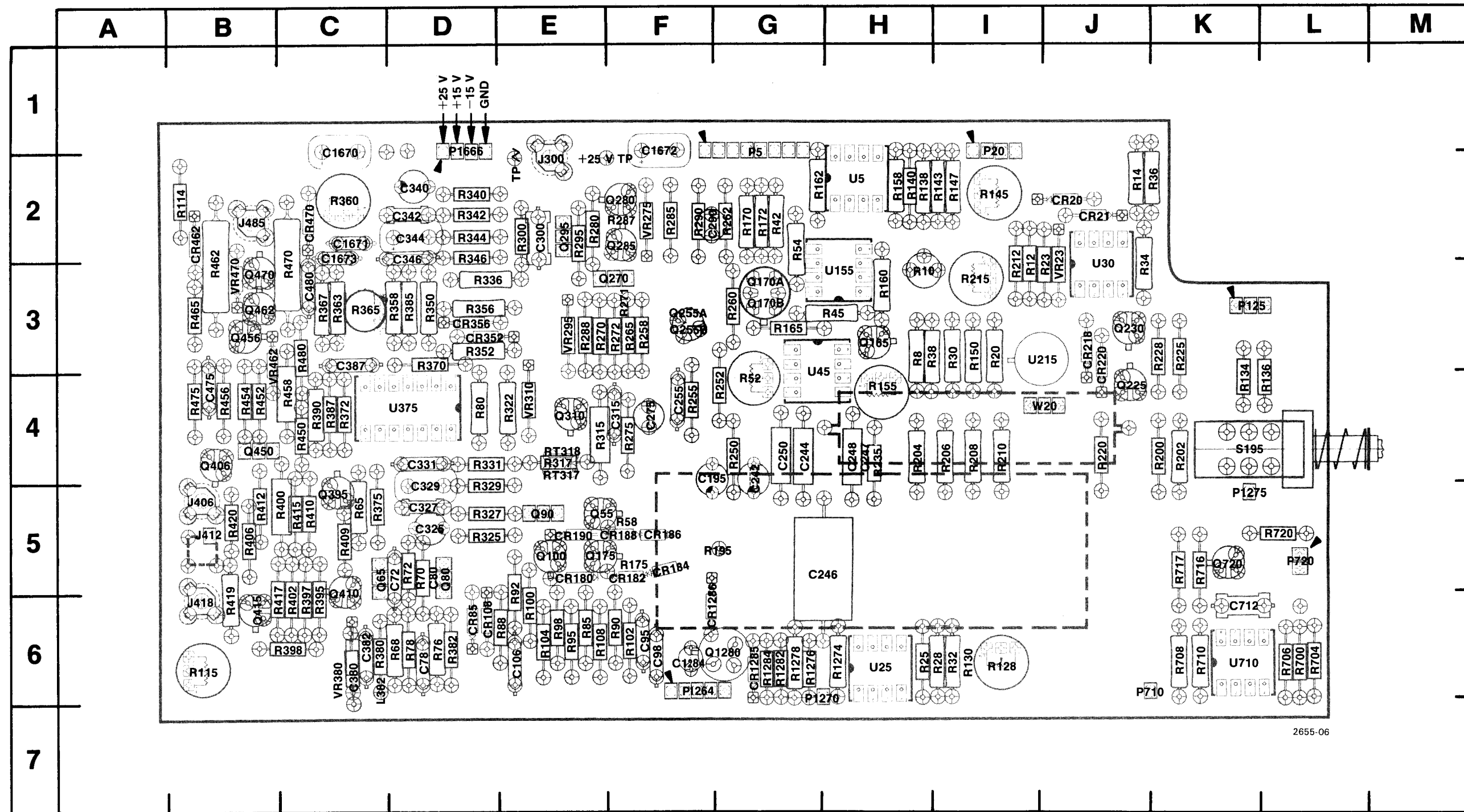
Fig. 8-3. A3 Loop board component locations.
