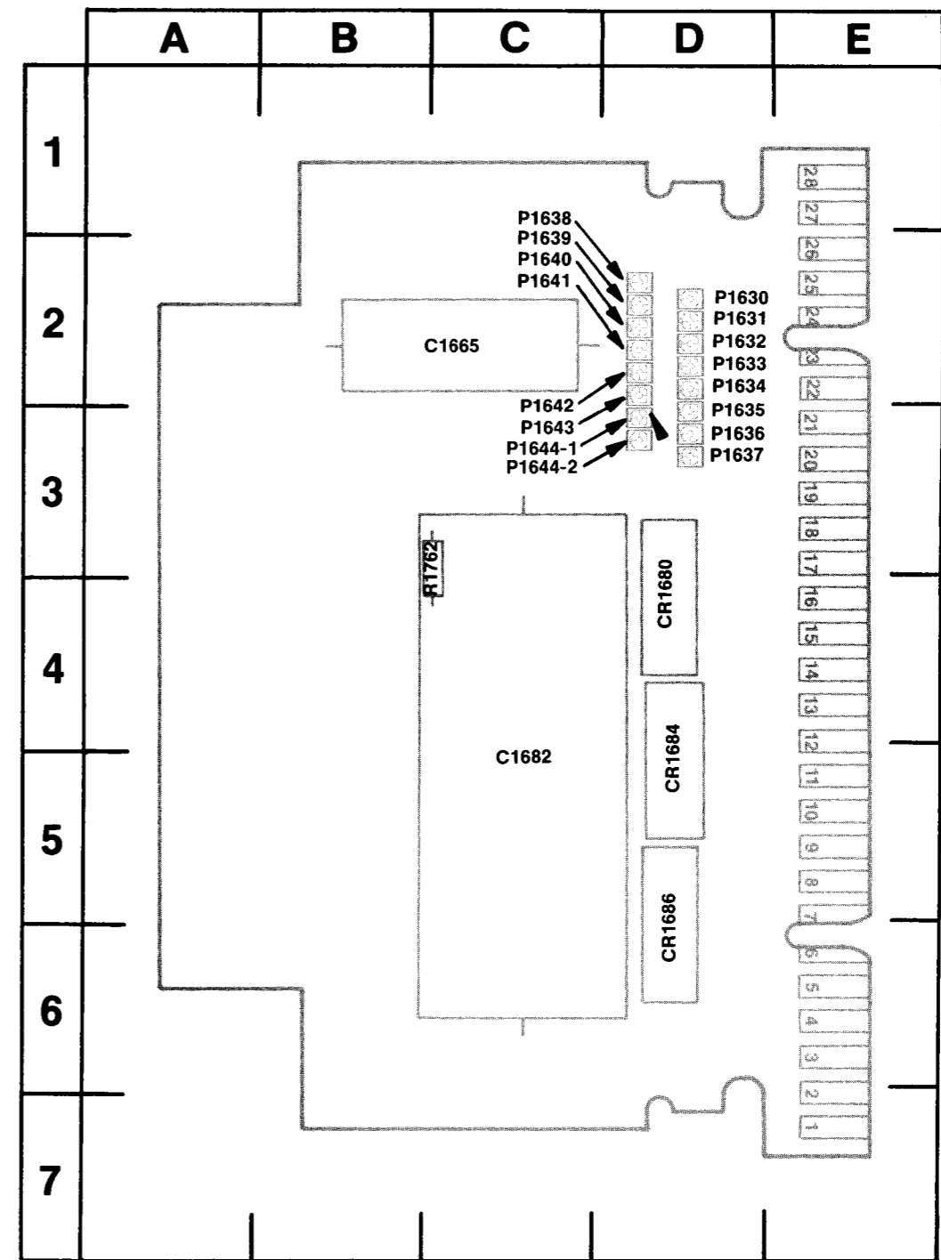
Fig. 8-8. A4 Floating Interface board (back) component locations.
