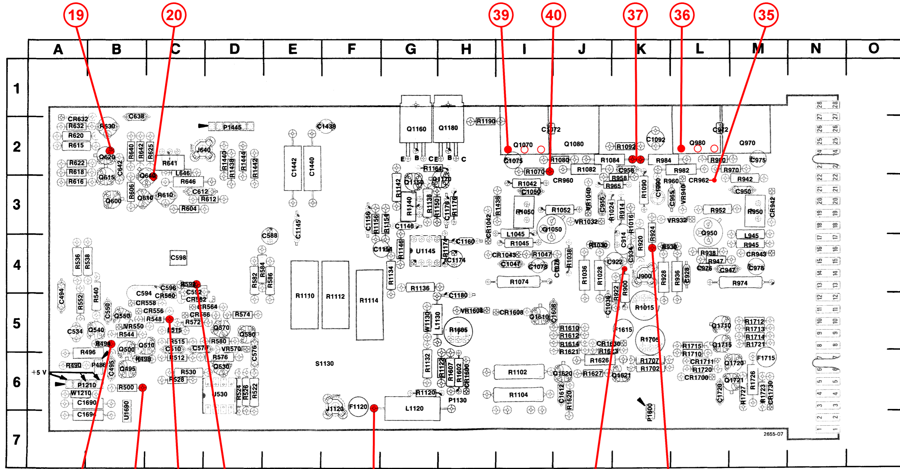
Fig. 8-4. A1 Main board (front) component locations.
