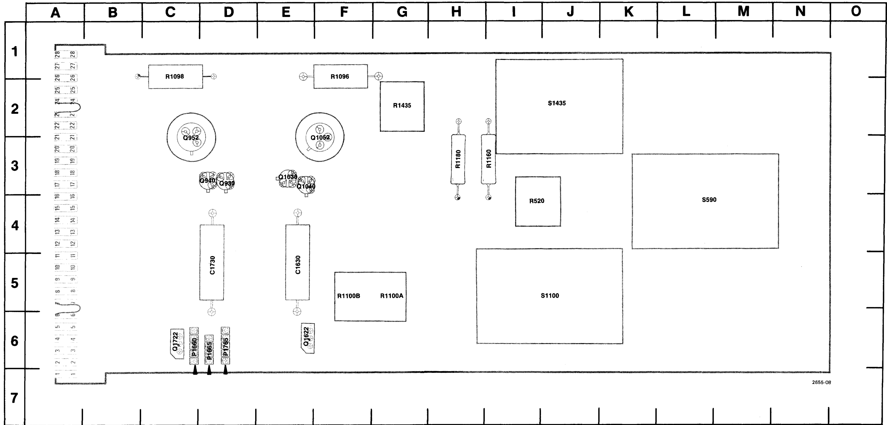
Fig. 8-5. A1 Main board (back) component locations.
