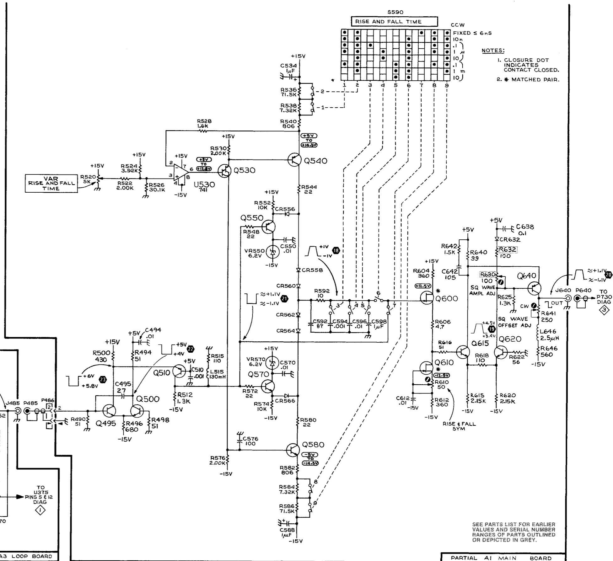
SQUARE BUFFER/VARIABLE RISE & FALL
