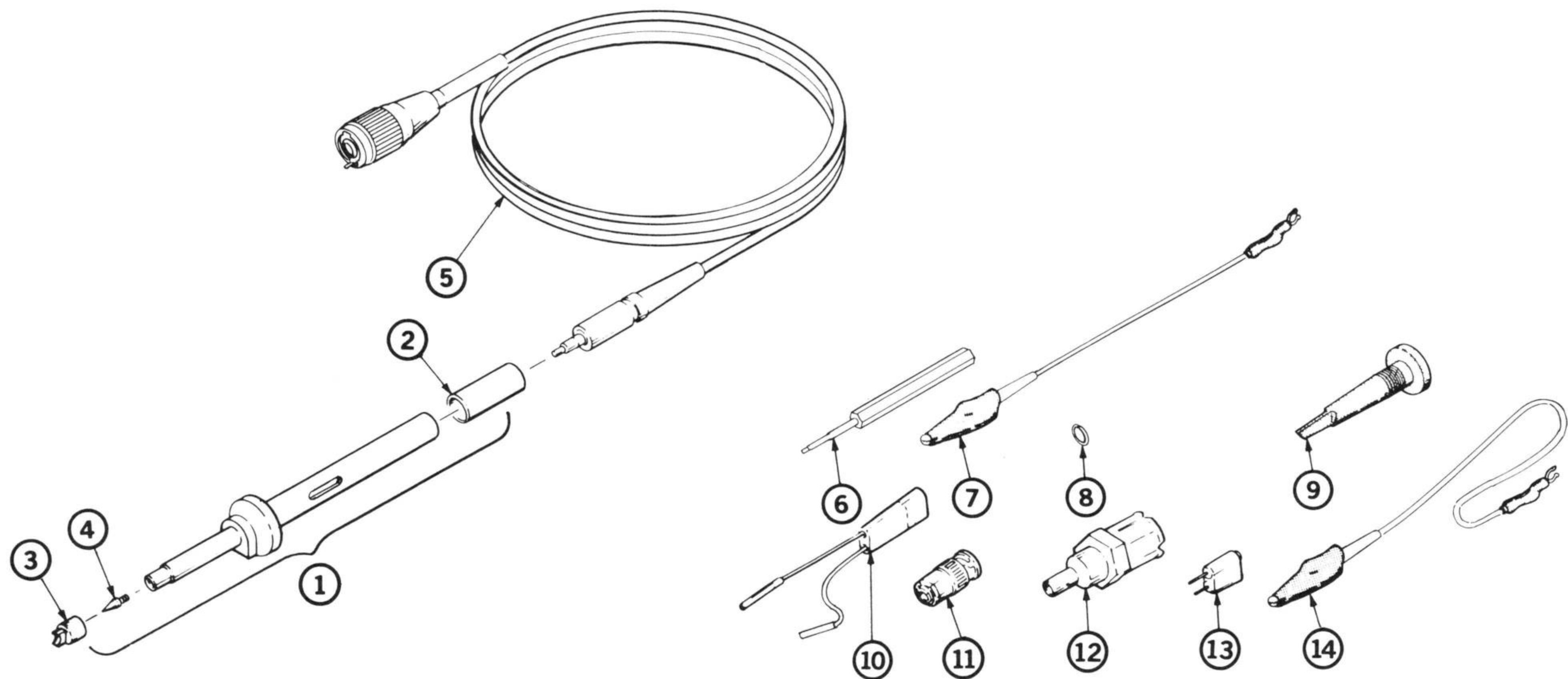
Figure 3. P6109 replaceable parts and accessories.
