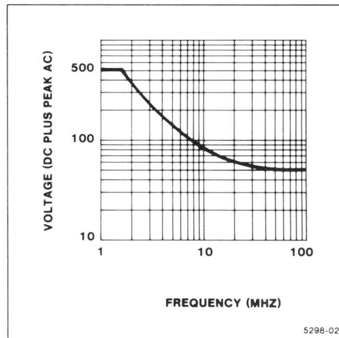
Figure 2. Typical voltage derating versus frequency.
