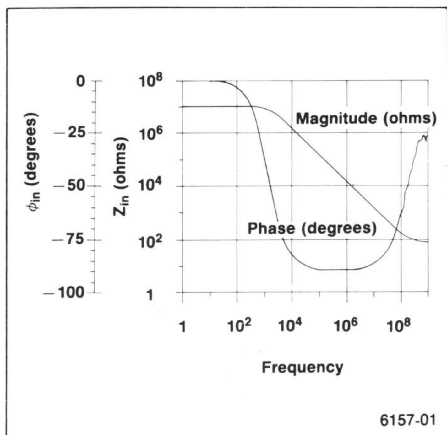
Figure 1. Typical input impedance.
