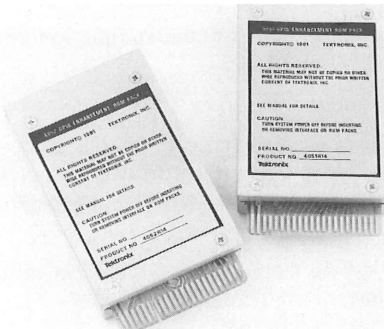
TEKTRONIX 4051R14 and 4052R14 GPIB Enhancement ROM Packs Expand Bus Control.
