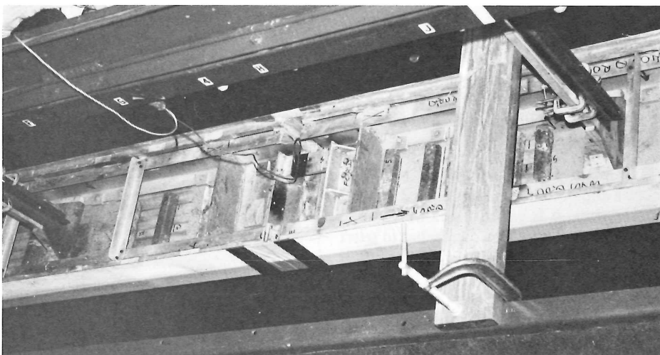
Figure 2b. Sensors on the midsection of the model pick up its bending moment. Dr. Armin Troesch is making some adjustments to the instrumentation.
