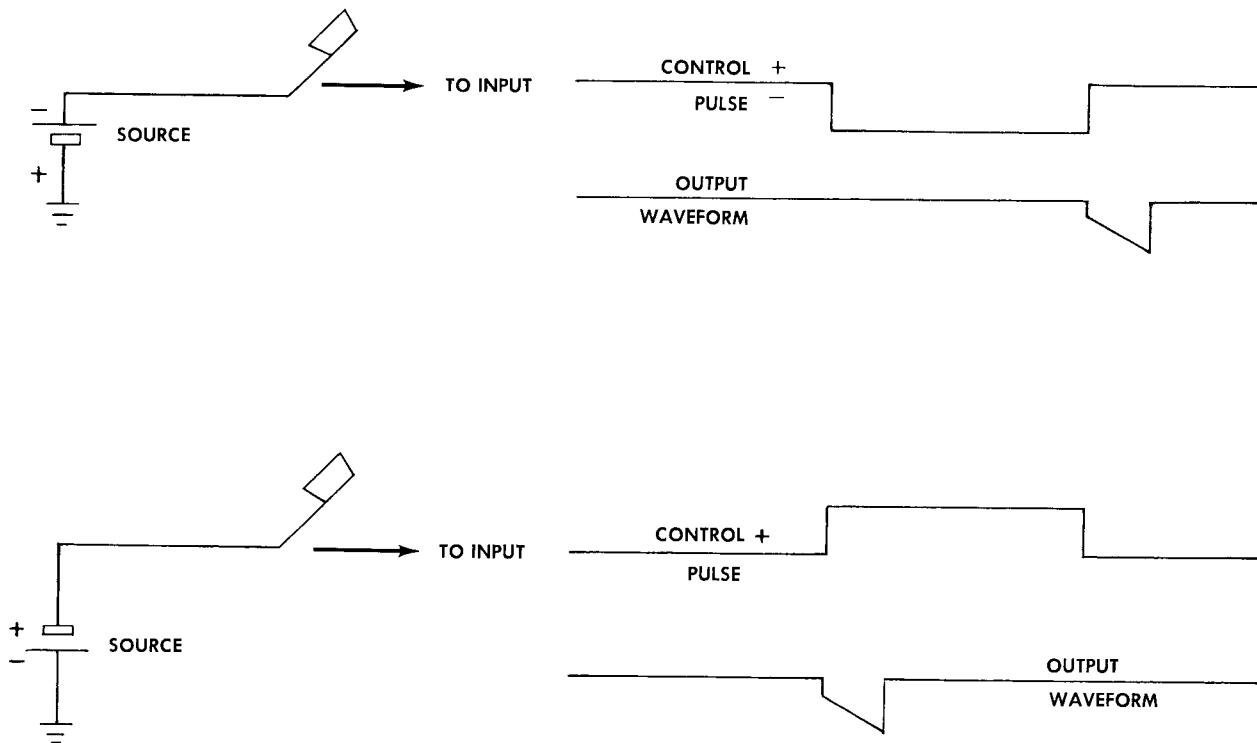
Fig. 2-12. Since the initiating pulses are positive-going waveforms, more predictable and less confusing operation will probably be obtained if the control pulse is habitually obtained from the positive terminal of the source.
