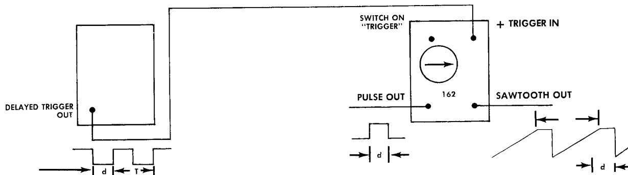
Fig. 2-10. Free running oscilloscope sweep determines rate of 162 sawtooth formation. Position of beginning of sawtooth pulse determined by setting of delayed trigger control on panel of oscilloscope. Duration of sawtooth determined by setting of waveform duration controls on panel of 162. A positive-going gate of the same duration as the sawtooth may be obtained simultaneously from the other output connection.
