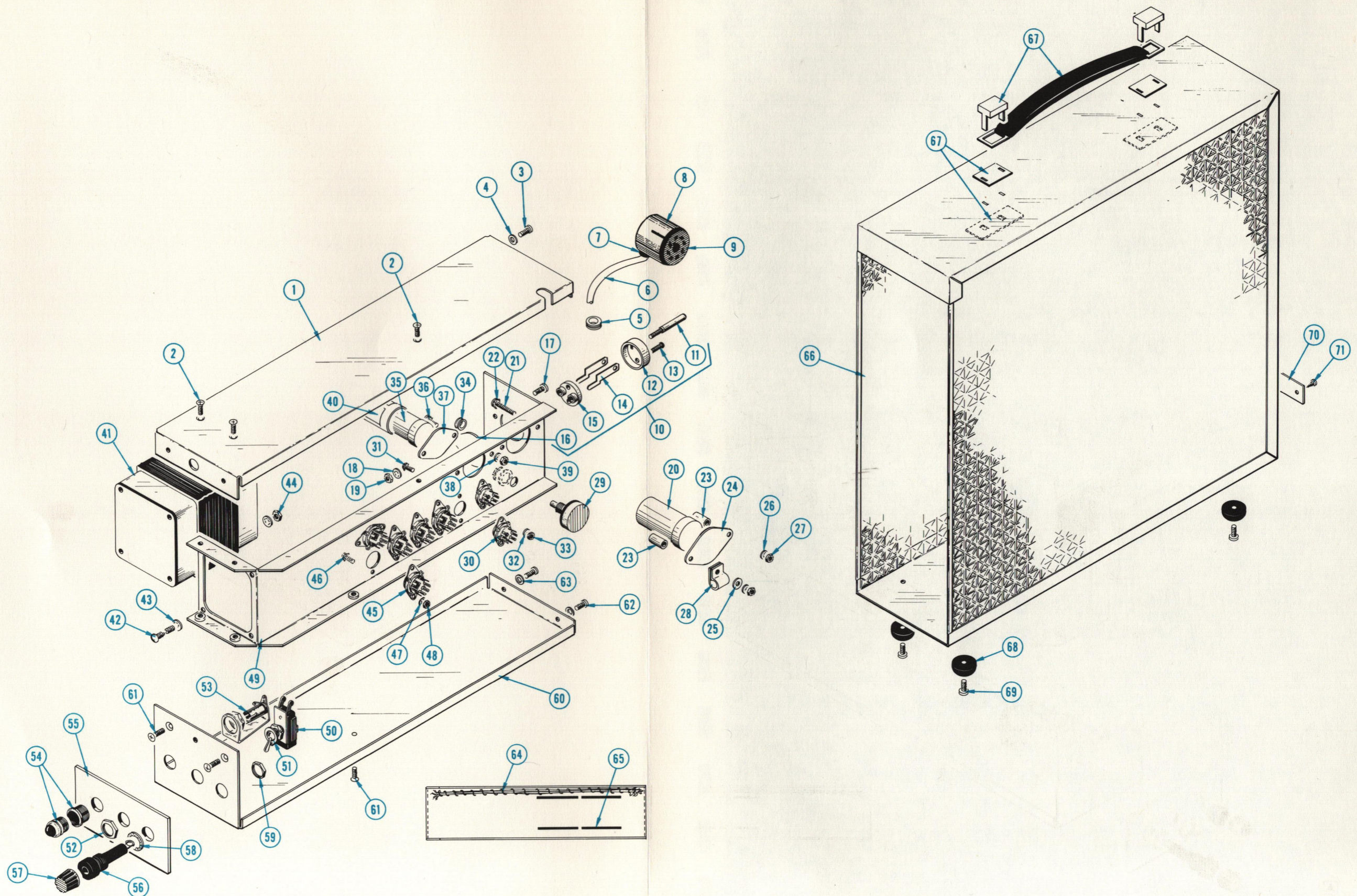
FIG. 8 TYPE 126 MECHANICAL PARTS & CABINET
