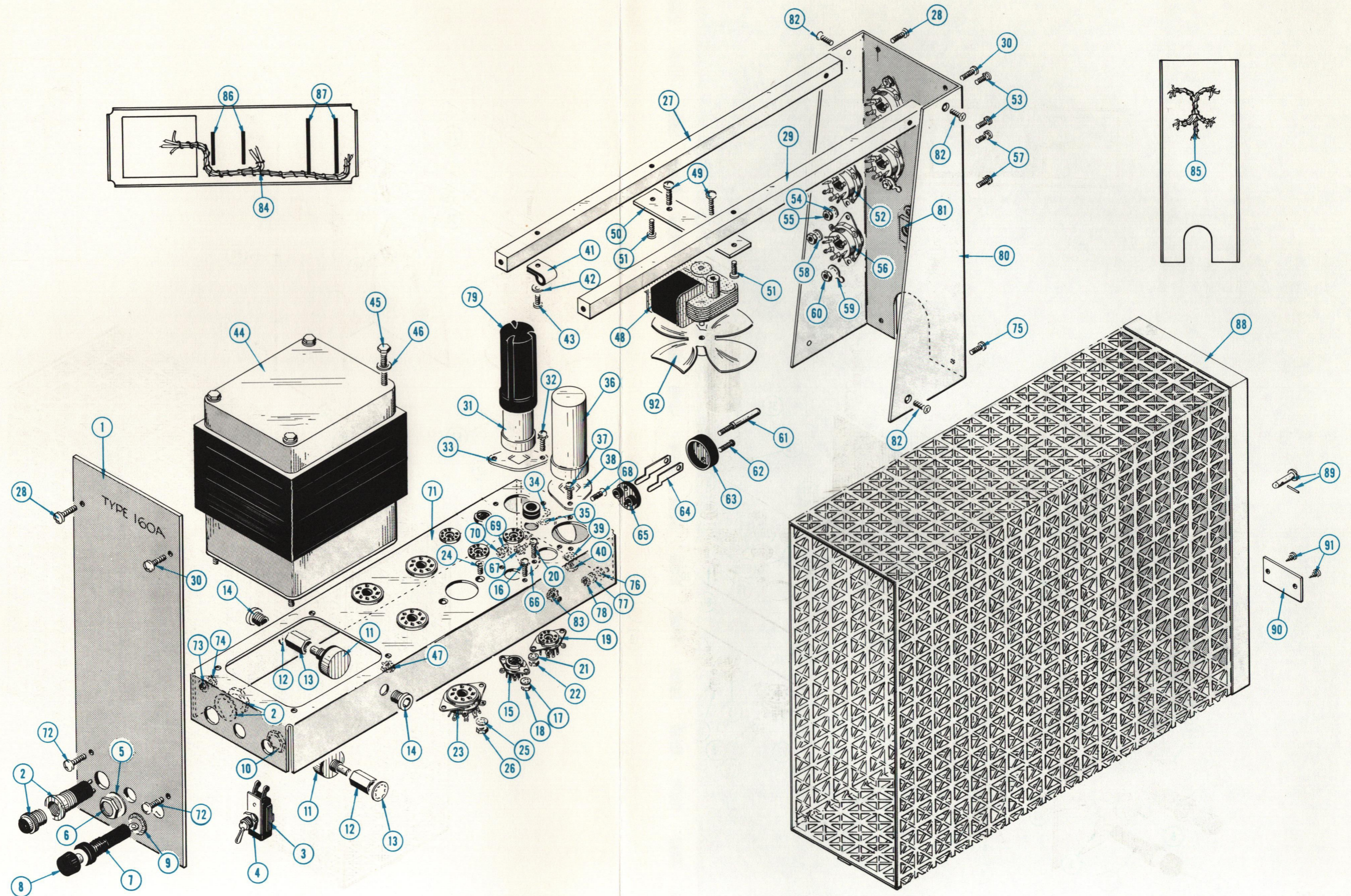
FIG. 2 TYPE 160A MECHANICAL PARTS
