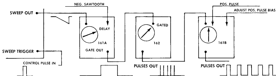
Fig. 2-21. All operations recycle at interval determined by control pulse. This initiates sweep of oscilloscope and sawtooth input to 161A. At a given time, determined by the delay setting of 161A, a positive-going gating pulse is initiated. The duration of the gate is determined by the duration settings of 161A. The 162 operates recurrently during a period determined by the gate from 161A. The frequency of operation of 162 is determined by the interval setting on the control panel of 162. The recurrent pulse output from 162 thus consists of a train of pulses of controlled time of initiation, controlled train duration and controlled repetition rate. The 161B produces a pulse out for each individual pulse in from the 162. The duration and amplitude controls the 161B permit control of the individual pulse dimensions in the train.
