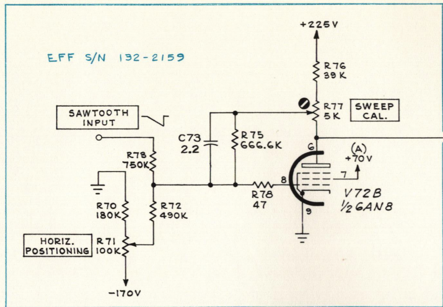
HORIZONTAL AMPLIFIER
