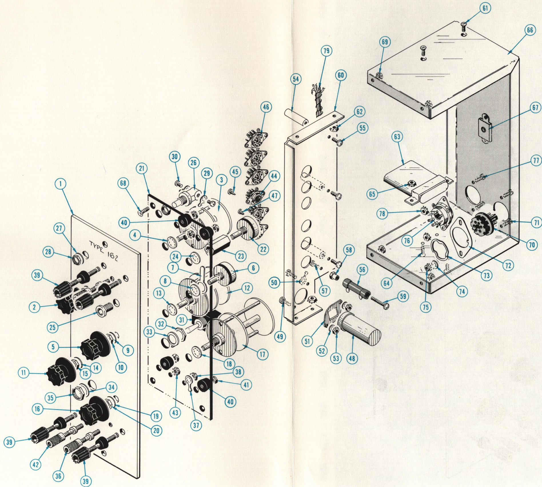
FIG. 4 TYPE 162 MECHANICAL PARTS
