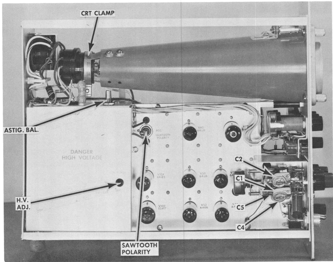
Fig. 4-11. Side view of the Type 360 Indicator Unit.
