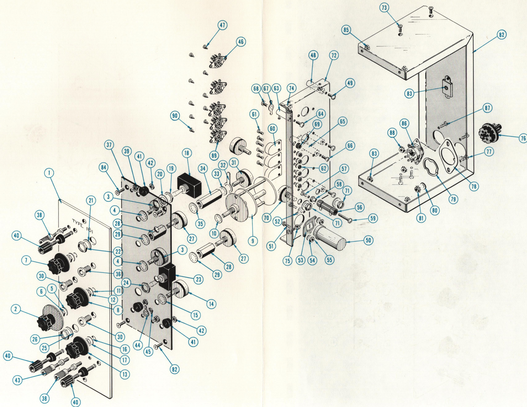
FIG. 3 TYPE 161 MECHANICAL PARTS
