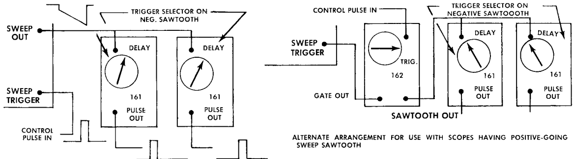
Fig. 2-20. All operations recycle at interval determined by control pulse. Delays and dimensions of output pulses determined by control settings of 161's.
