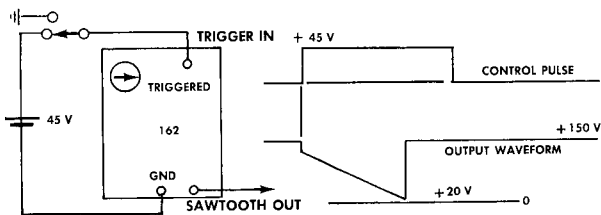
Fig. 2-4. An external battery used as the positive trigger source for a Type 162. Note that the output sawtooth starts as the triggering waveform becomes positive-going. Note also that the switch in its normally open position connects to ground.
