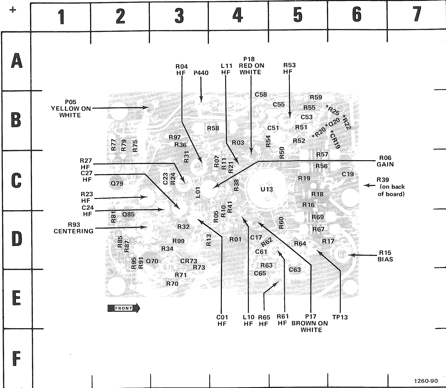
Fig. 6-20. A44 - Vertical Amplifier circuit board.
