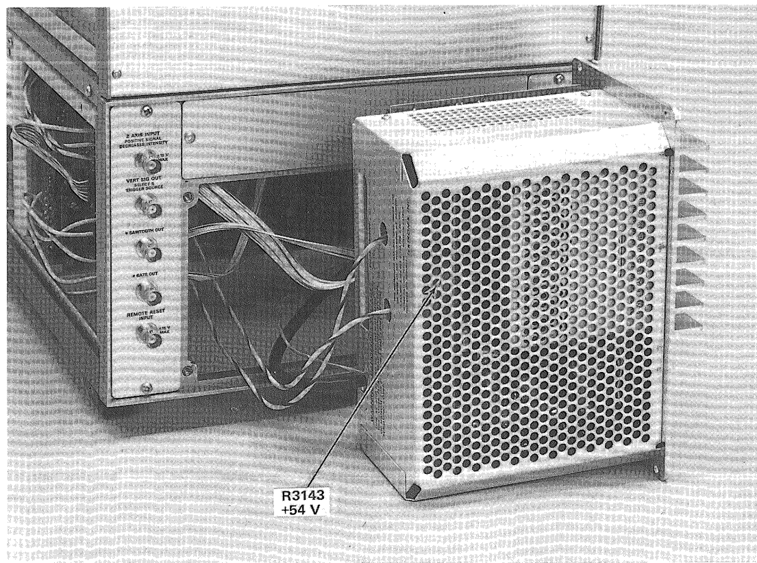
Fig. 6-27. +54-Volt adjustment, R3143, location in power unit.
