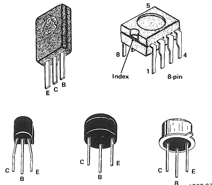
Fig. 6-25. Electrode configuration for semiconductors shown on diagram 14.
