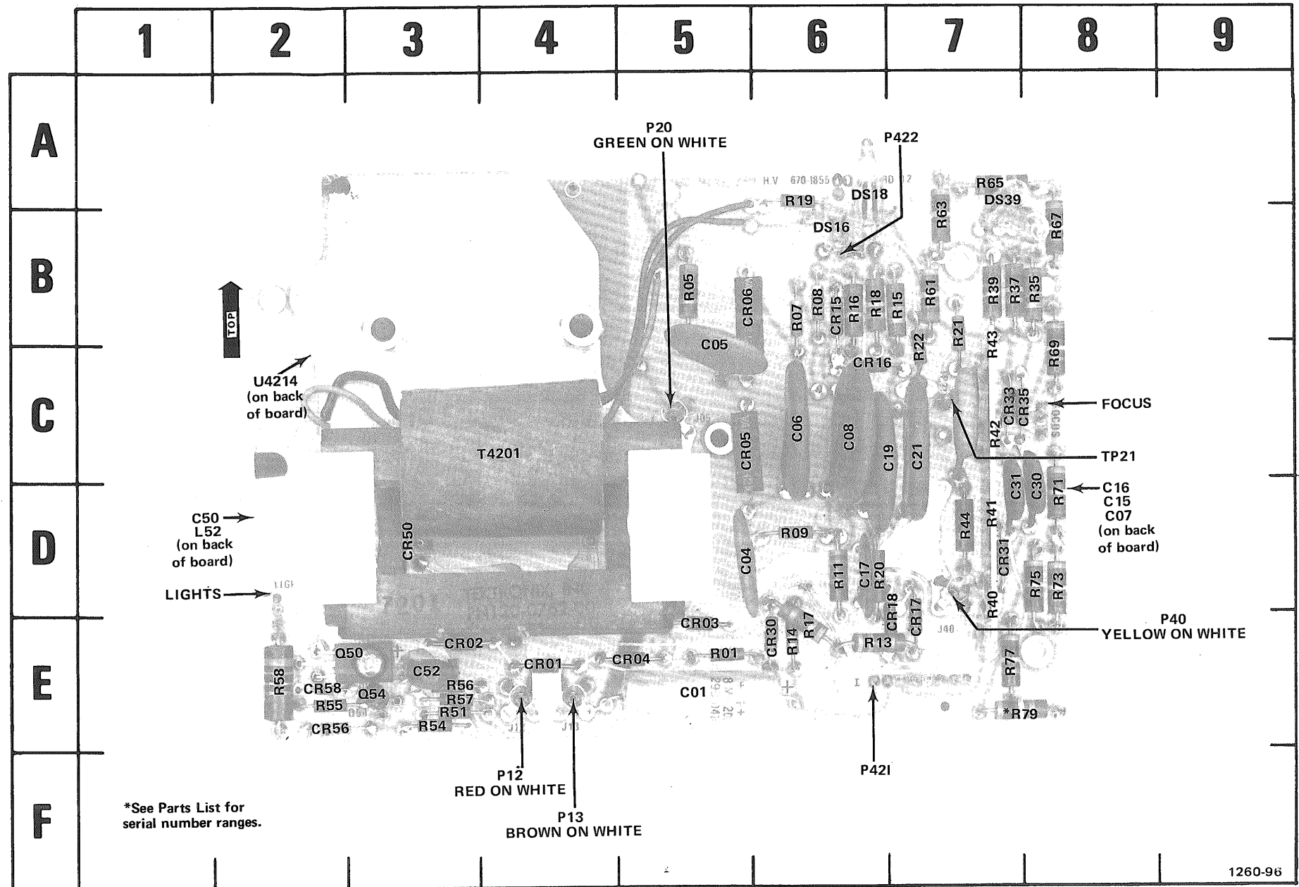
Fig. 6-24. A42-HV circuit board.
