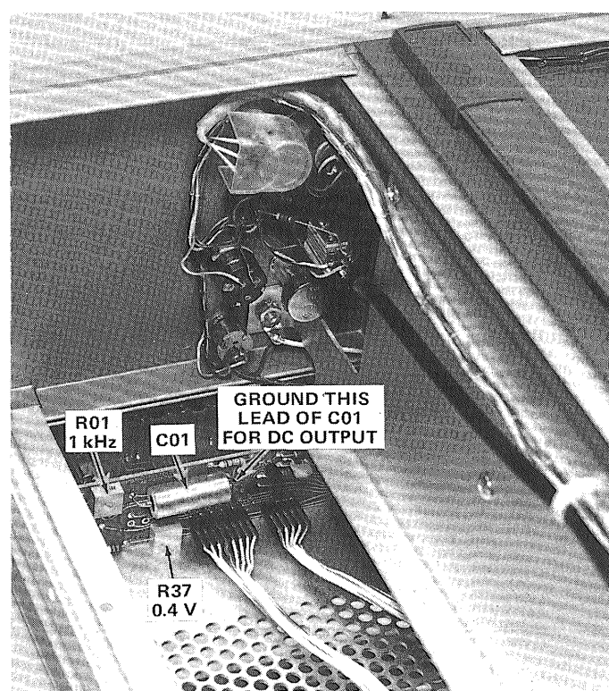
Fig. 6-35. Location of Calibrator adjustments on A10 – Calibrator board.
