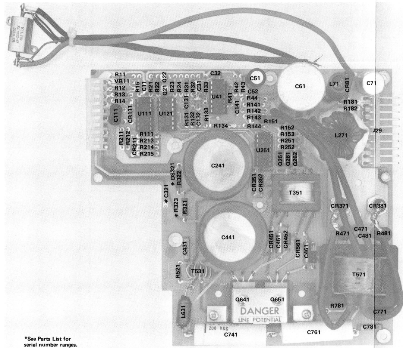
+5 Volt Output Board Component Locations (670-5622-00,01,02).
