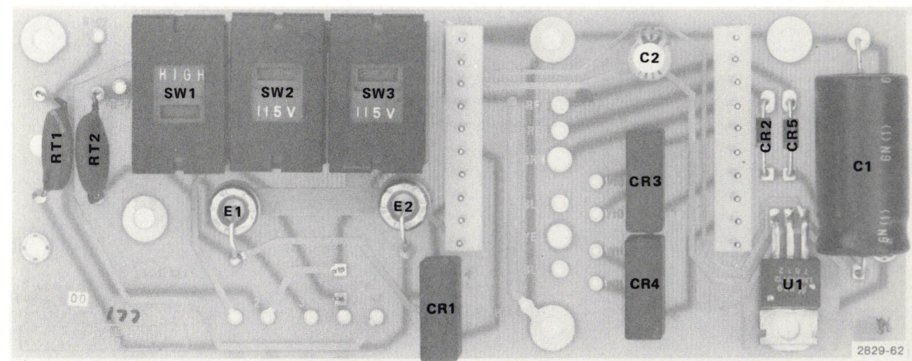
Line Selector Board Component Locations (670-5621-00).
