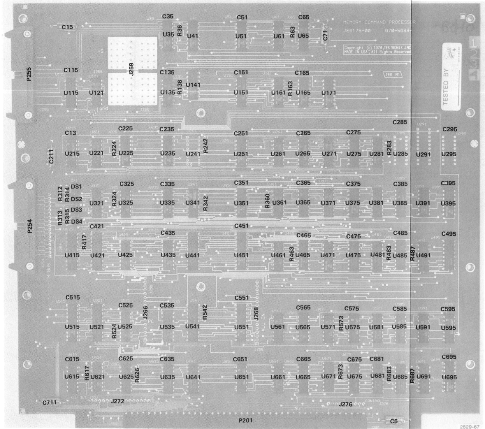
MCP Board Component Locations (670-5633-00,01).
