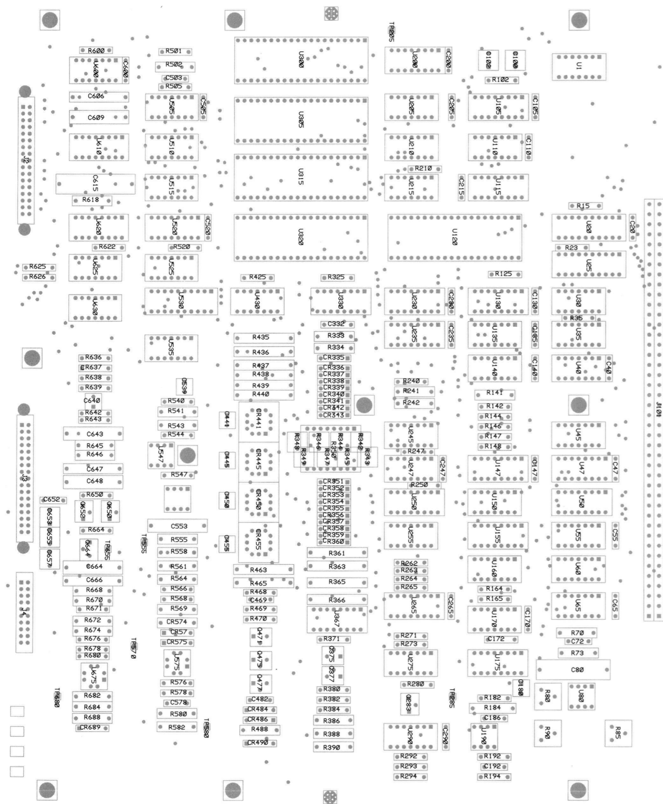
4052A I/O Board Component Locations (670-7629-00).
