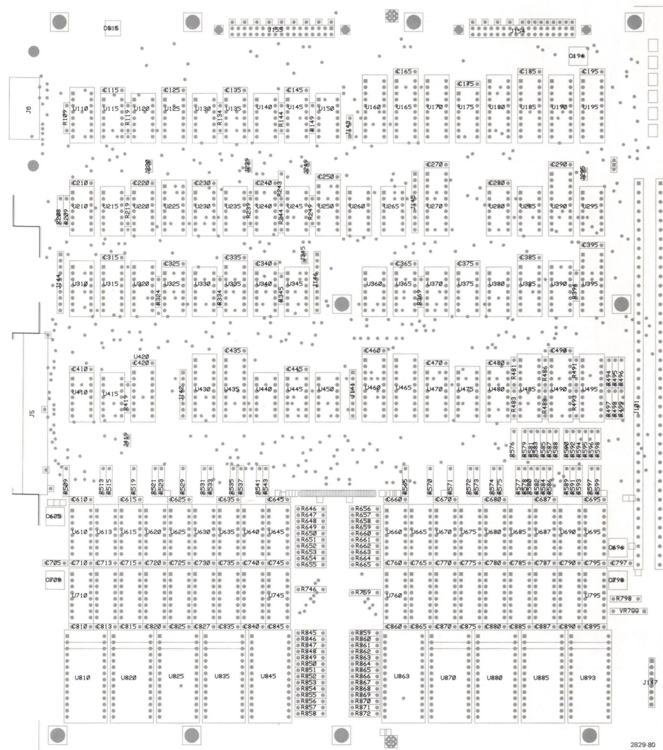
4052A MAS Board Component Locations (670-7624-00).
