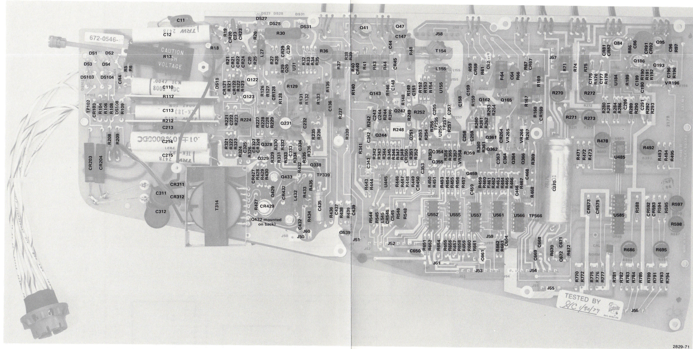
Display Board Component Locations (670-4087-05 and up).
