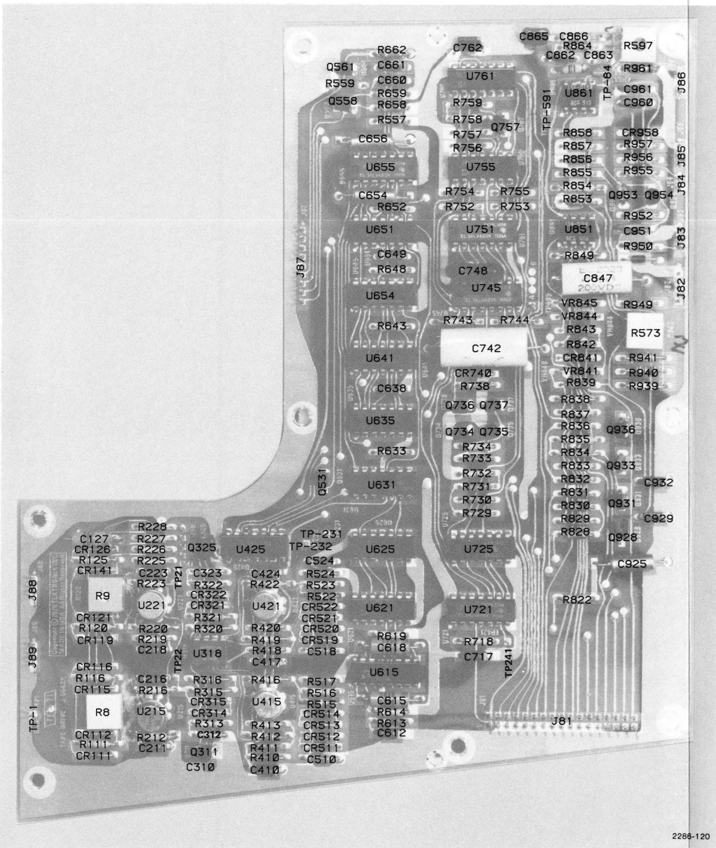
Tape Drive Board Component Locations (670-4003-04 and up).
