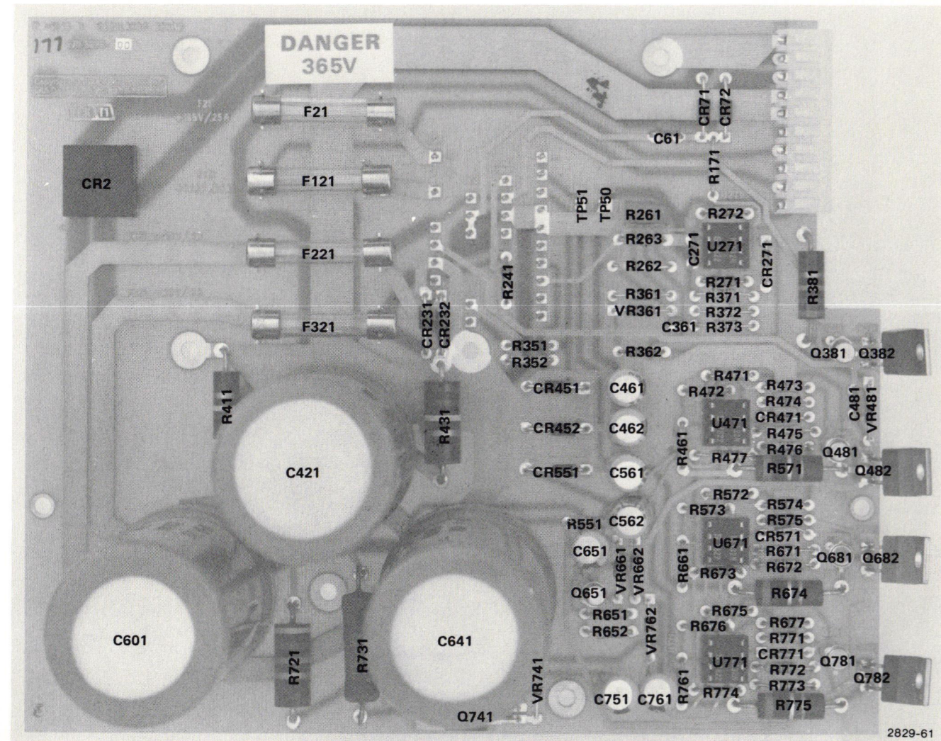
Regulator Board Component Locations (670-5623-00,01).
