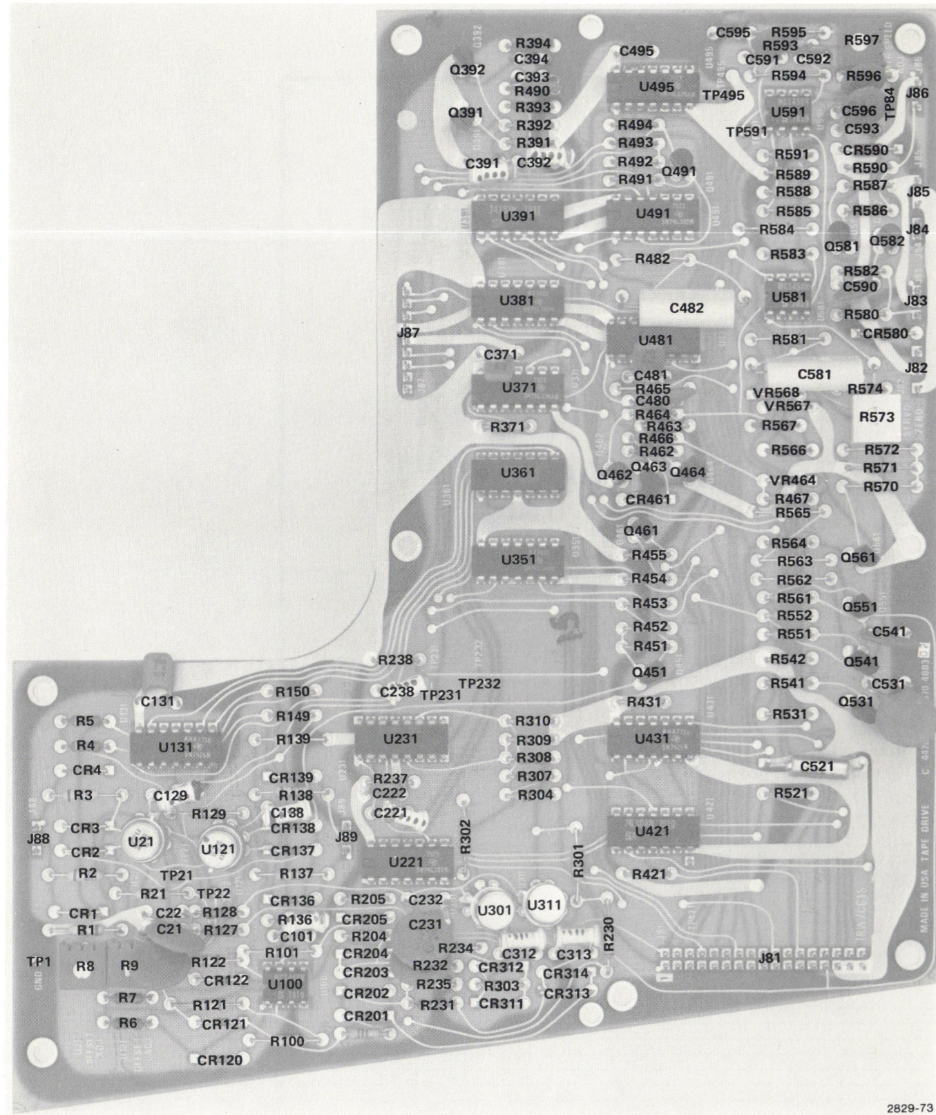
Tape Drive Board Component Locations (670-4003-00,01,02,03).
