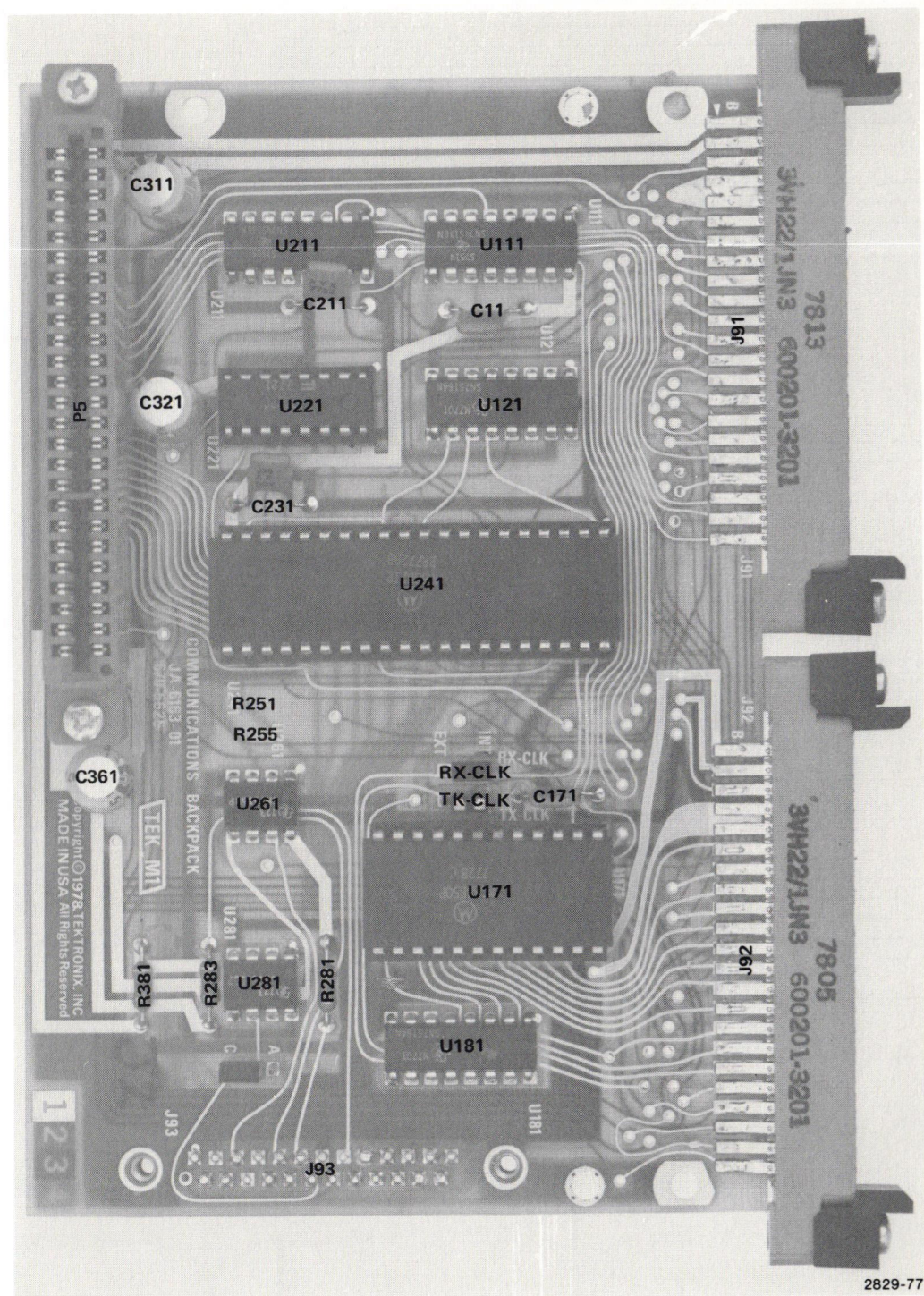
Option 01 Communication Backpack Component Locations (670-5626-00,01).
