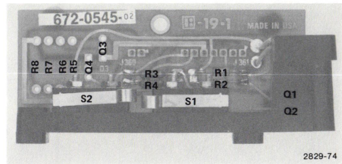
Tape Status Component Location (670-3896-00).
