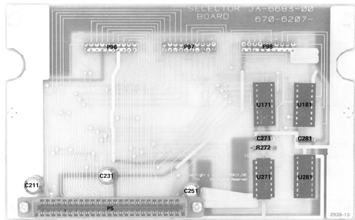
Option 02 Selector Board Component Locations (670-6207-00).
