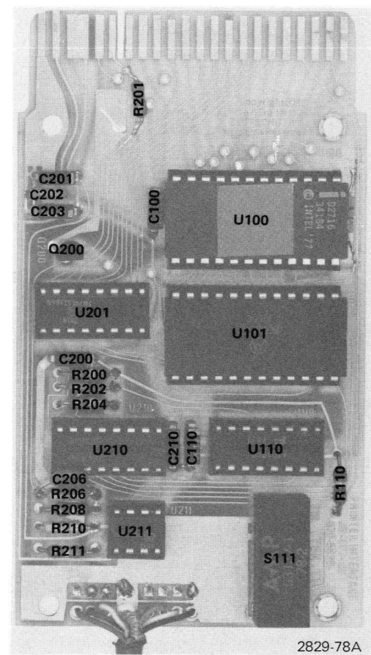
Option 10 Printer I/F Board Component Locations (670-5636-00,02,03).
