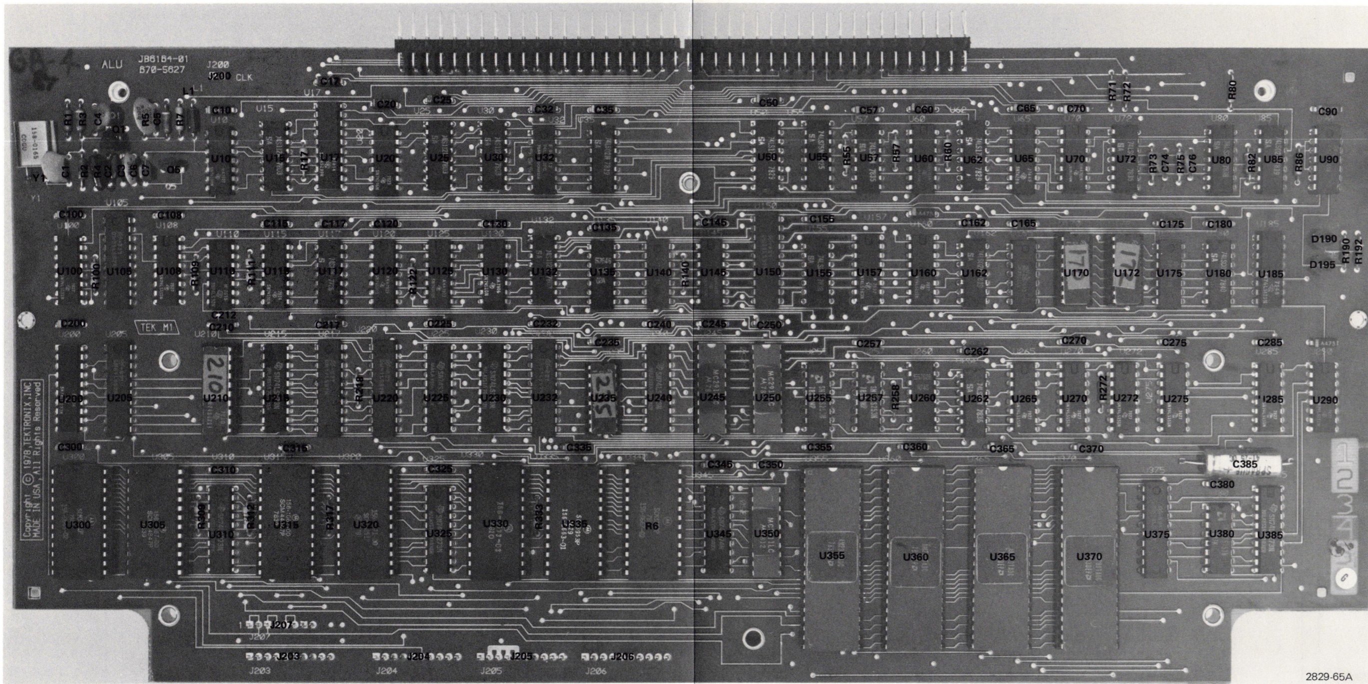
ALU Board Component Locations (670-5627-00,01,02,03 and 670-7705-00).
