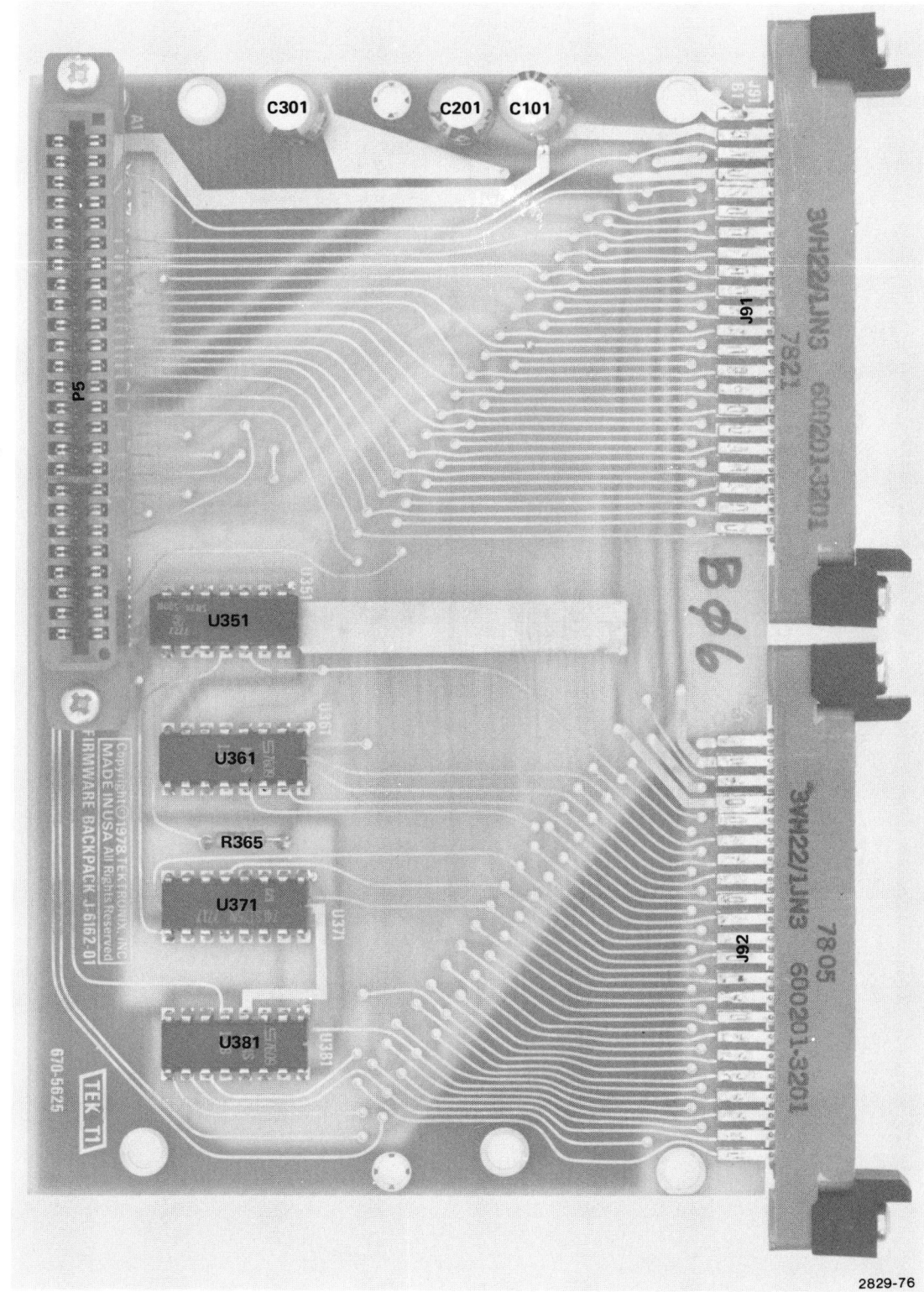
Firmware Backpack Board Component Locations (670-5625-00).
