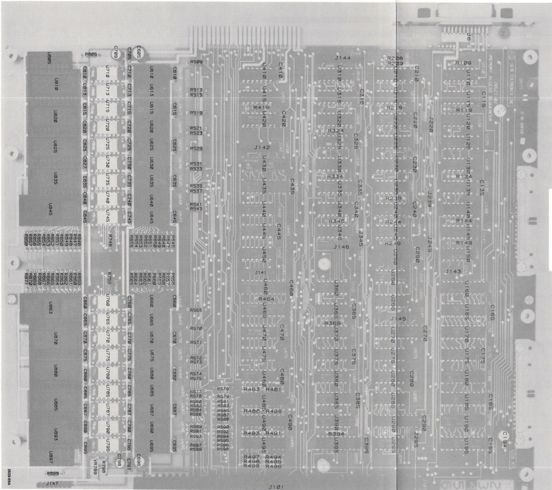
4052 MAS Board Component Locations (670-6030-00 and up).
