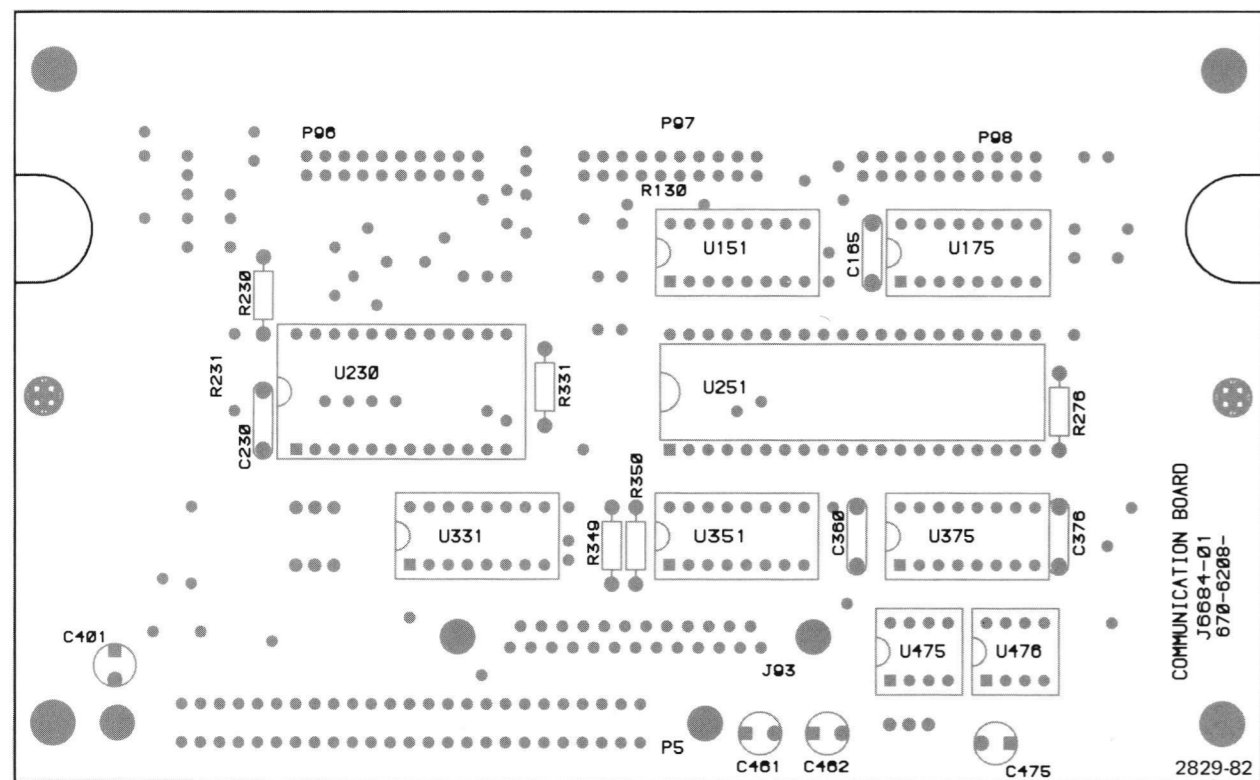
Option 03 Communication Board Component Locations (670-6208-00).
