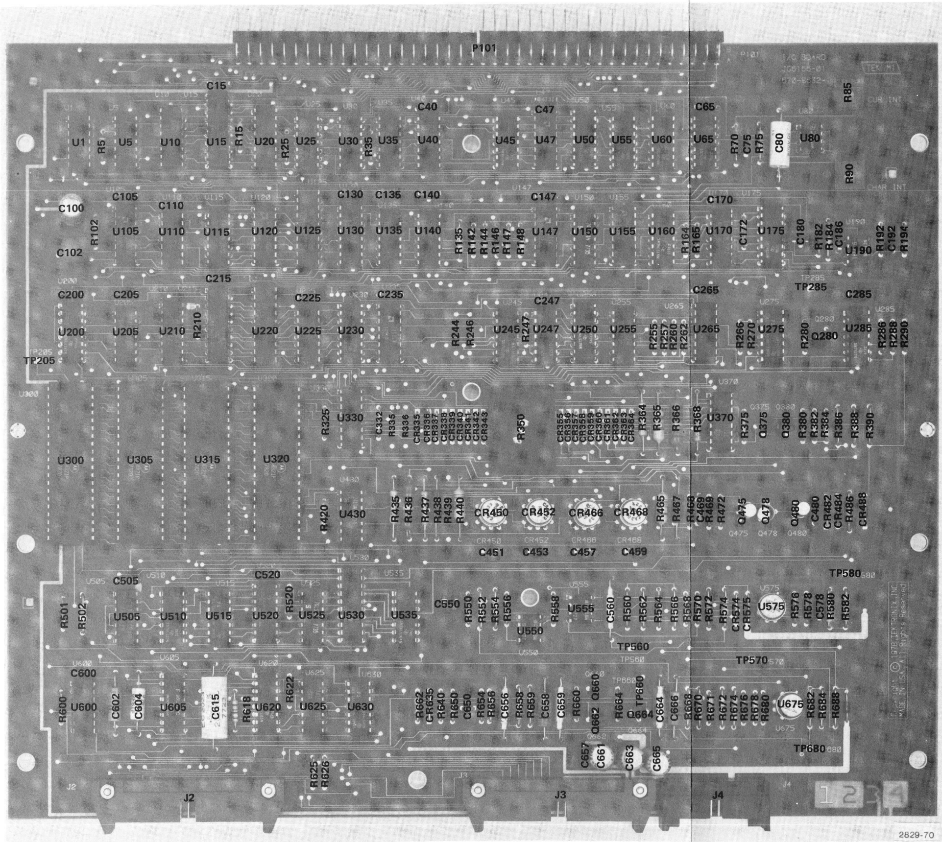
4052 I/O Board Component Locations (670-5632-00,01,02,03,04).
