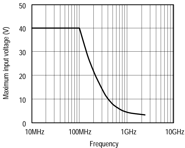
Figure 3-2: Voltage derating vs frequency
